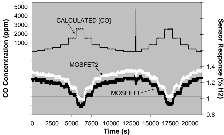
Figure 2: Results of CO cross-sensitivity test.
