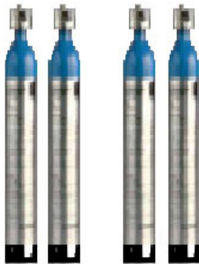
Figure 4: Hydrides metal.
