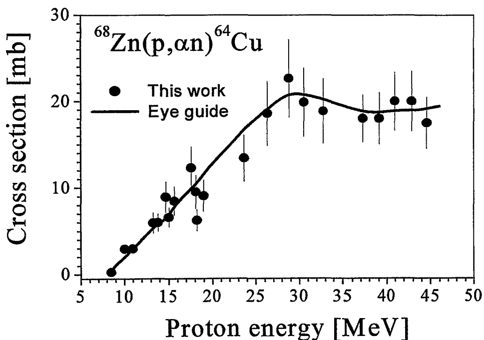
Fig. 2 Excitation function of the ^{68}\text{Zn}(p,\alpha n)^{64}\text{Cu} reaction.
