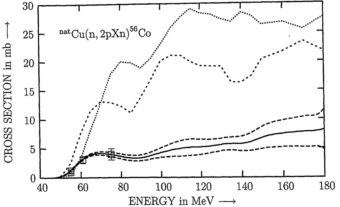
Fig. 5 Unfolded cross sections (solid line) with their uncertainties (dashed lines) for the reaction {}^{\text{nat}}\text{Cu}(n, 2pXn){}^{56}\text{Co} . The squares are cross sections reported earlier by Kim et al. [26]. The dotted and short-dashed lines represent two guess functions calculated by the ALICE-IPPE code using the Myers and Swiatecki mass formula [33] without and with shell corrections, respectively.
