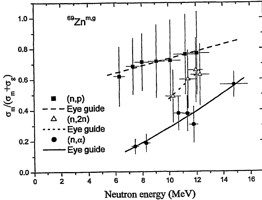
Fig. 1 Experimental isomeric cross section ratios for the formation of ^{69m,g}\text{Zn} in (n, \alpha ), (n,p) and (n,2n) reactions, shown as a function of incident neutron energy.
