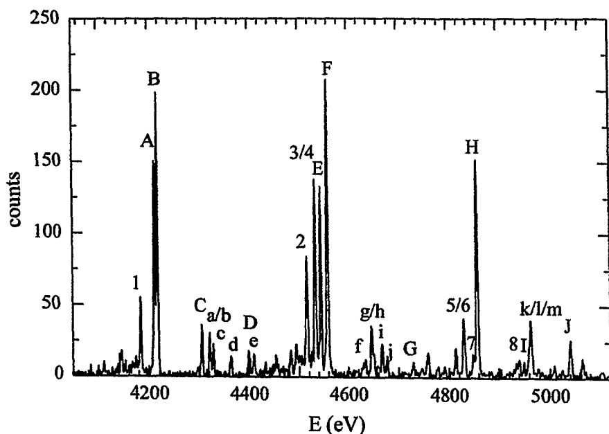
Fig. 1 Crystal diffraction spectrum of L x-ray transitions in \text{Xe}^{43+...45+}
