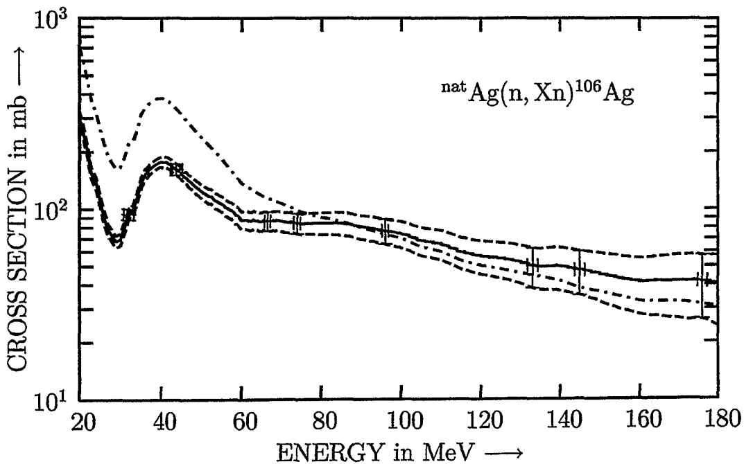
Fig. 4 Guess excitation function (dashed-dotted line) and final cross sections (solid line) with their uncertainties (dashed lines) for the reaction ^{nat}\text{Ag}(n,\text{xn})^{106}\text{Ag} . The crosses are the cross sections at the peak energies of the neutron irradiation experiments. The uncertainties in energy given for the cross sections represent the half-width of the peak in the neutron spectrum.
