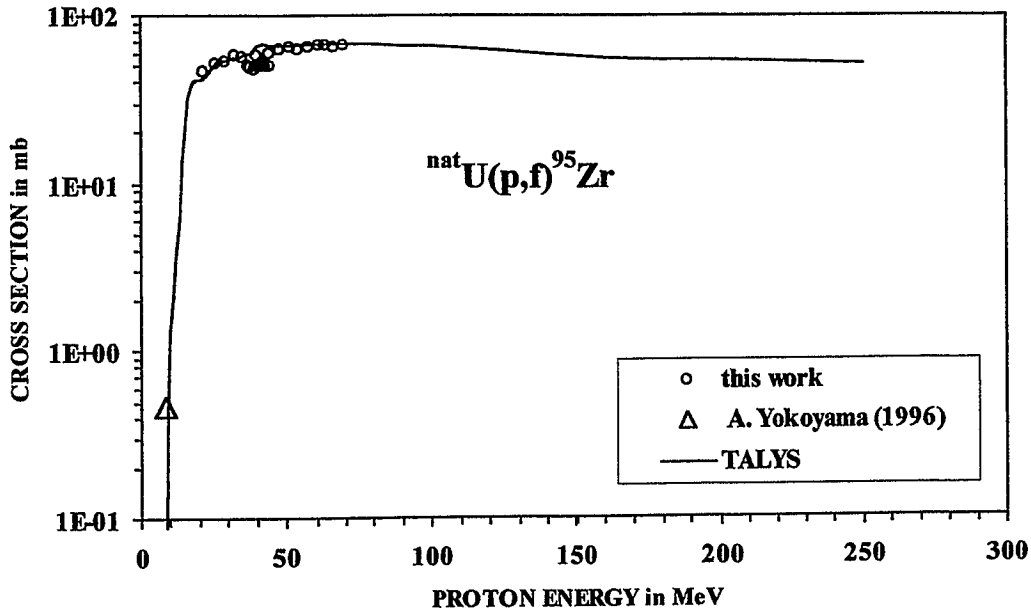
Fig. 1 Comparison of experimental cross sections from this work and from Yokoyama [14] with theoretical ones calculated by the TALYS code for the cumulative production of ^{95}\text{Zr} in proton-induced fission of natural uranium.
