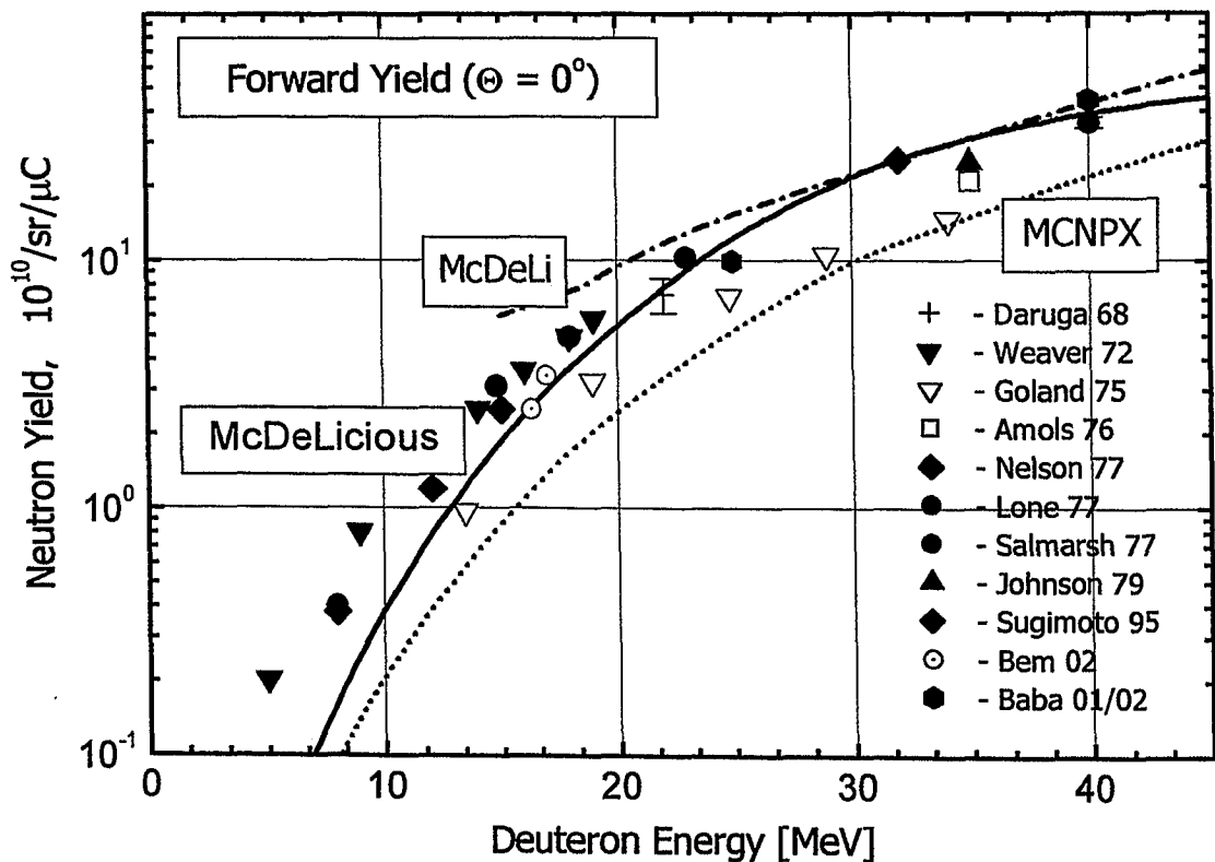
Fig. 1 Comparison of calculated and measured thick lithium target forward neutron yield data.
