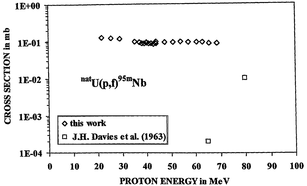
Fig. 2 Experimental cross sections from this work and from Davies et al. [15] for the production of ^{95m}\text{Nb} in proton-induced fission of natural uranium.
