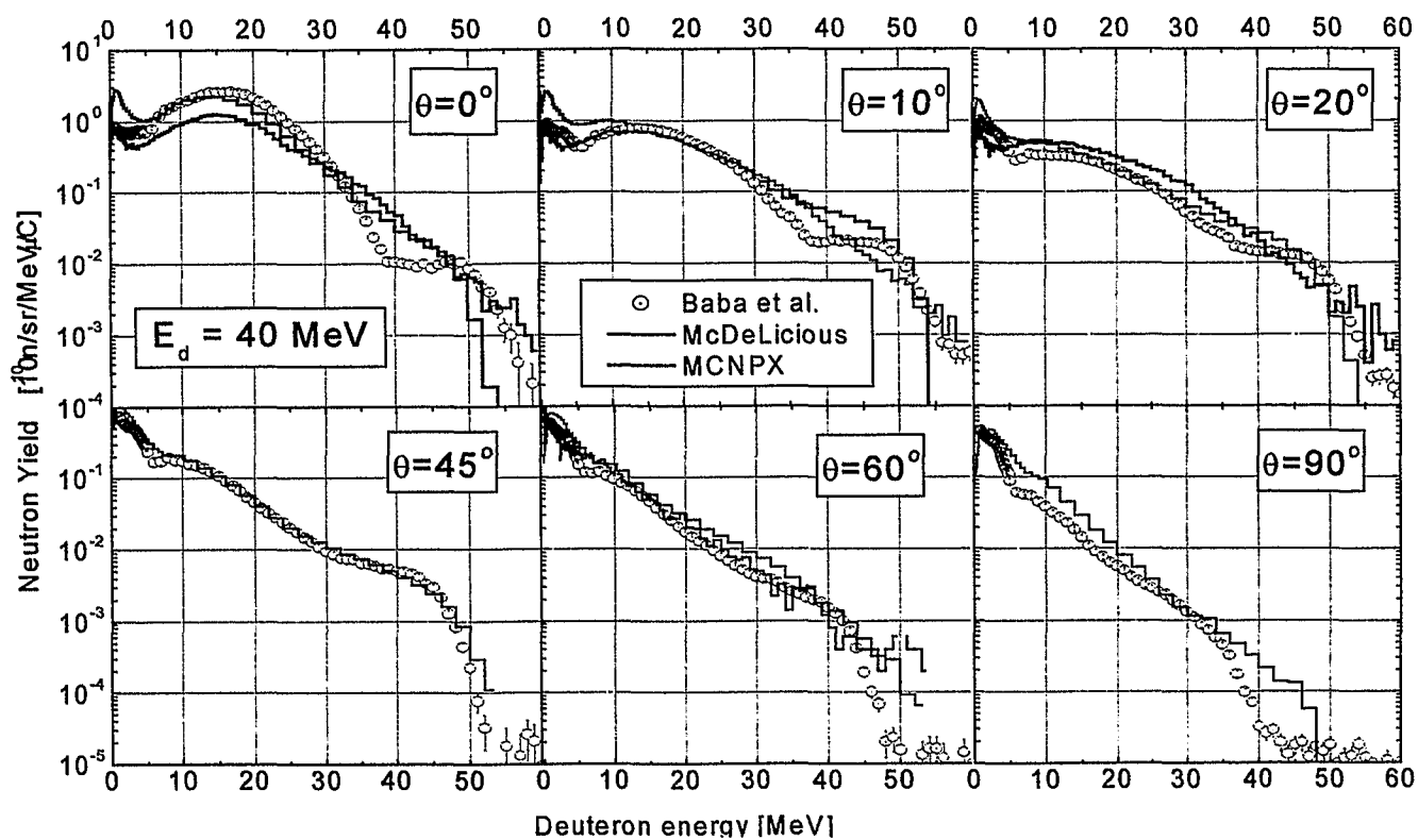
Fig. 3 Measured [4] and calculated thick target neutron yield angular spectra at an incident deuteron energy of 40 MeV.
