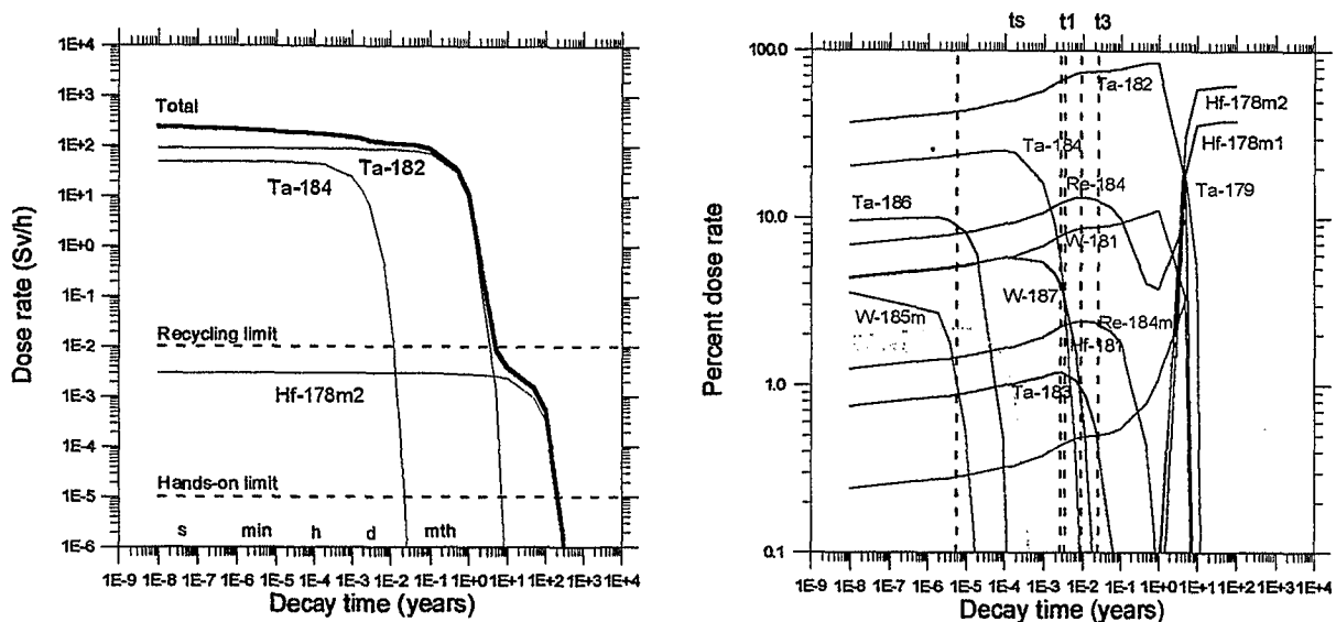
Fig. 1: Contact dose rate (left hand) and contribution of the different radionuclides to the total dose rate (right hand) after irradiation of W with 14 MeV neutrons of 1.0 MW/m 2 power density for one year as a function of decay time.
