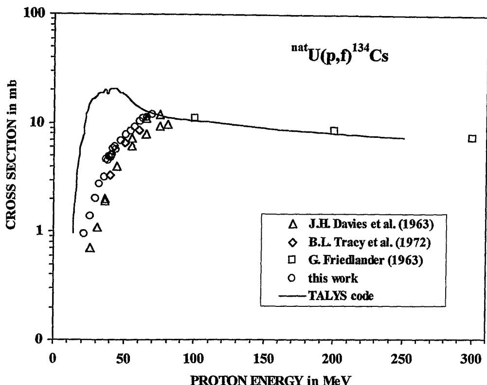
Fig. 3 Comparison of experimental cross sections from this work and from Davies et al. [15], Tracy et al. [16] and Friedlander [17] with theoretical ones calculated by the TALYS code for the independent production of ^{134}\text{Cs} in proton-induced fission of natural uranium.
