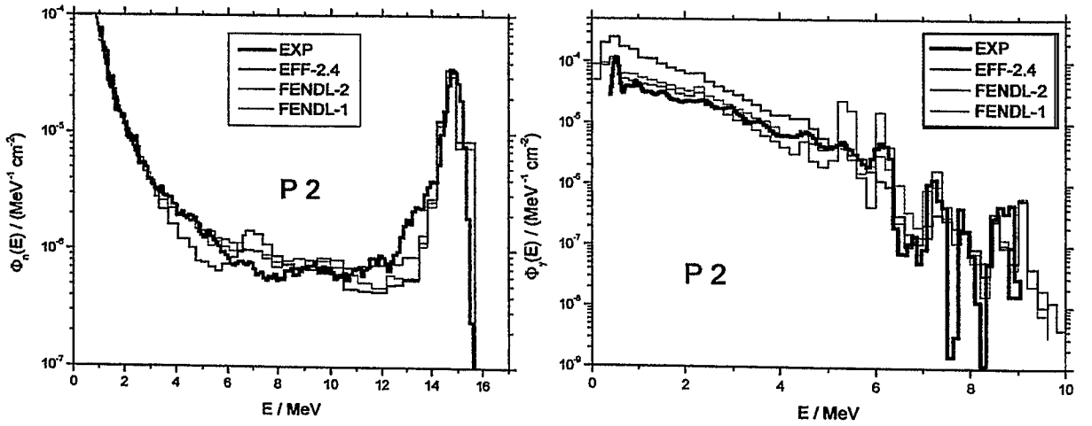
Fig. 2 Measured neutron (left hand) and \gamma -ray (right hand) flux spectra at detector position P 2 (normalised to one source neutron) in comparison to fluxes calculated with data from the libraries EFF-2.4, FENDL-1 and FENDL-2.
