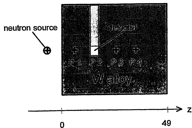
Fig. 1 Geometry of the benchmark assembly with the detector in position 2.
