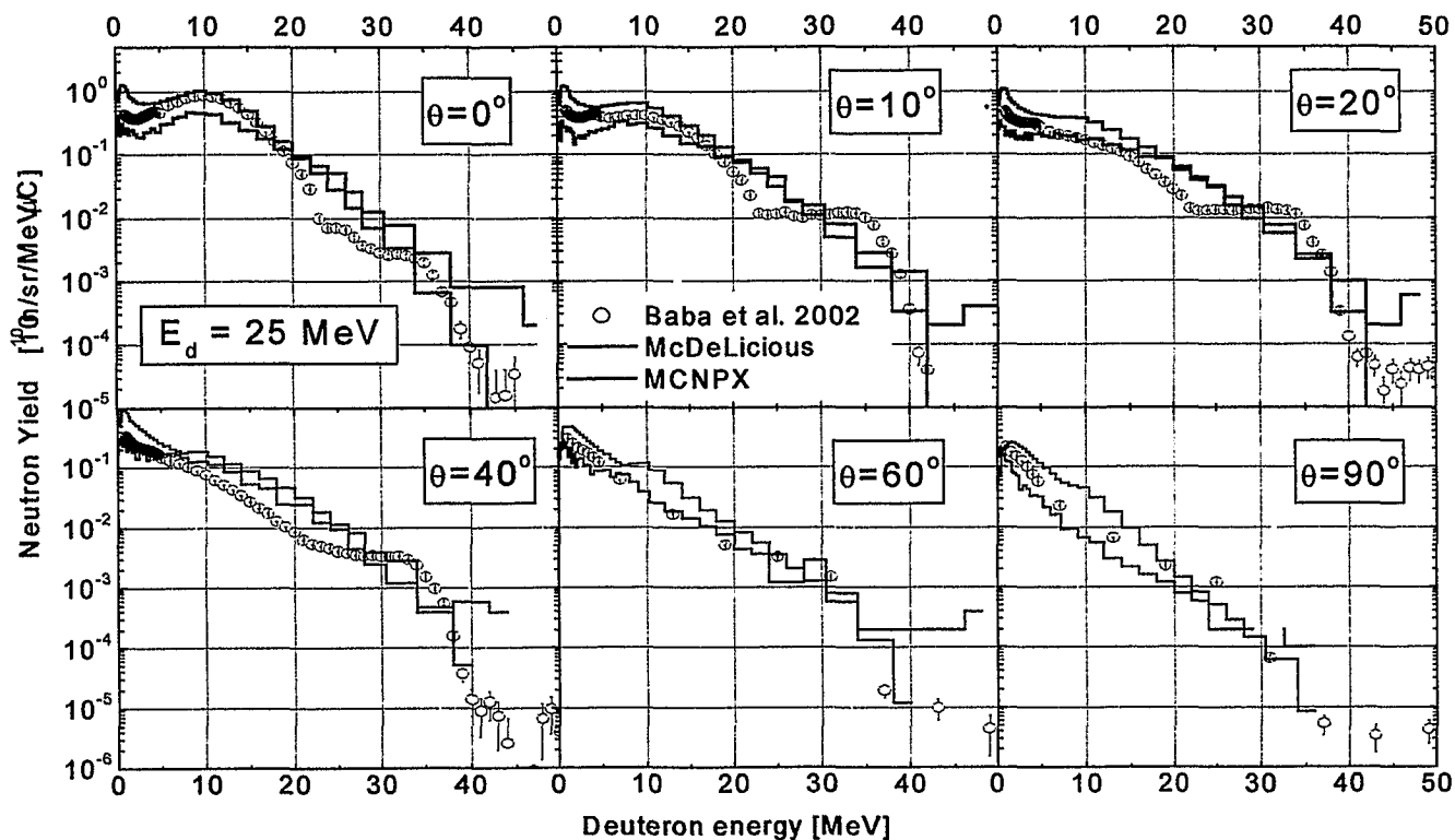
Fig. 2 Measured [4] and calculated thick target neutron yield angular spectra at an incident deuteron energy of 25 MeV.
