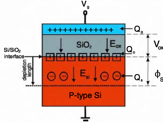
Figure 2.3: MOS capacitor under a positive applied gate voltage V_g showing charges, fields and potentials.
