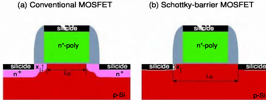
Figure 2.1: Schematic cross-section of (a) a conventional MOSFET and (b) a Schottky-barrier MOSFET.
