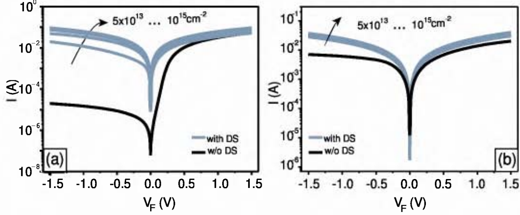
Figure 5.1: (a) I - V_F characteristics of NiSi/ n -Si (100) with and without dopant segregation. (b) I - V_F characteristics of NiSi/ p -Si (100) with and without dopant segregation. V_F is the applied voltage between the metal and the semiconductor.
