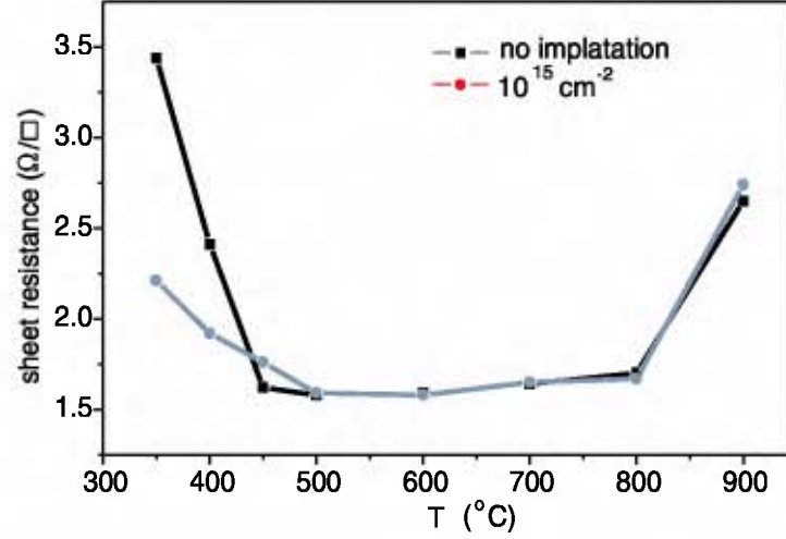
Figure 3.4: Sheet resistance versus annealing temperature. All samples were annealed for 30s.
