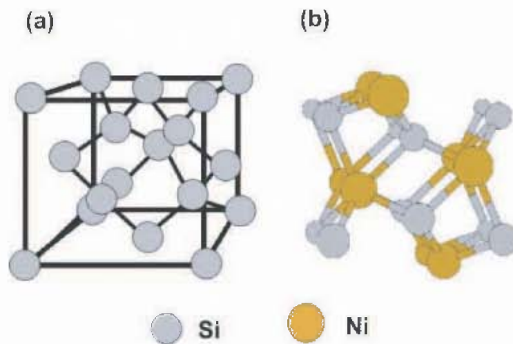
Figure 3.3: Crystal structure of (a) Silicon (Diamond structure) (b) NiSi (MnP structure)
