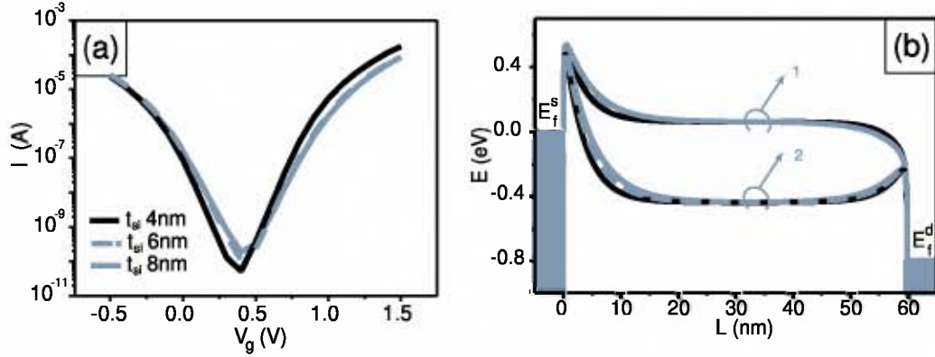
Figure 4.6: (a) Transfer characteristics for a 60 nm SB-MOSFET at V_{ds} of 0.8V with a SBH of 0.64eV, t_{ox}=1nm but different t_{si} . (b) Energy band diagram for off-state (1) and on-state (2).
