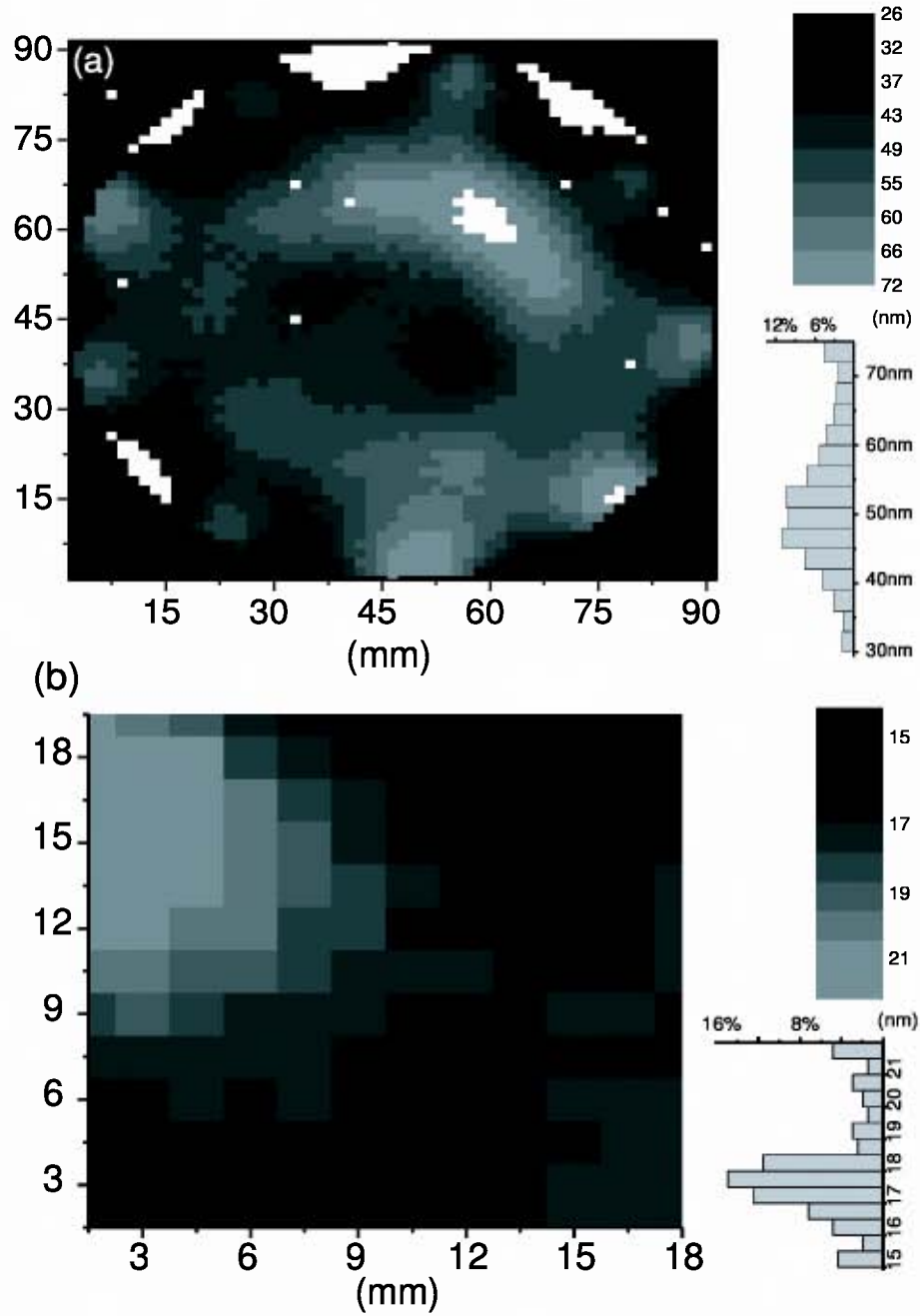
Figure 6.4: (a) Thickness map of a 4" SOI wafer after 1000°C 3 hours dry oxidation followed by the removal of the grown \text{SiO}_2 using DHF (average t_{\text{si}}=53\text{nm} ). (b) Thickness map of a 2cm x 2cm SOI sample after dry/wet oxidation and oxide stripping (average t_{\text{si}}=16\text{nm} ).
