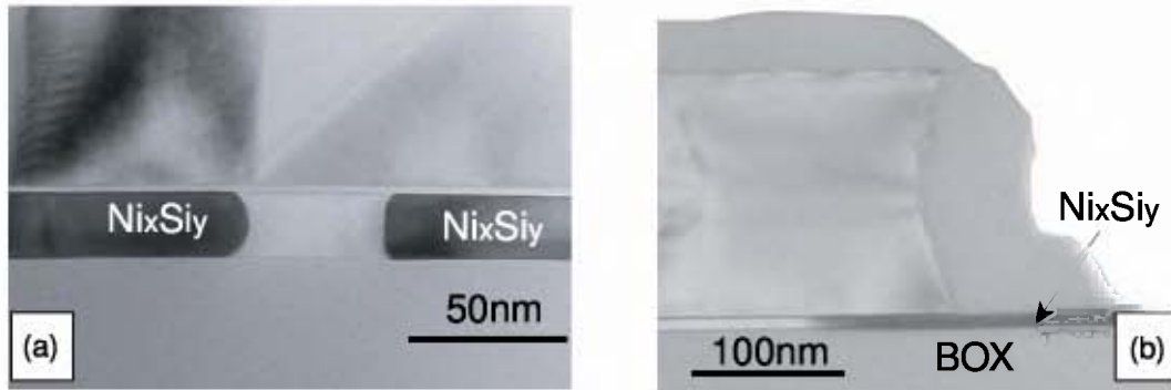
Figure 3.9: XTEM micrograph showing (a) aggressive lateral growth of \text{Ni}_x\text{Si}_y under a 1\text{ }\mu\text{m} gate length. The spacing between the \text{Ni}_x\text{Si}_y contacts shrank to 50nm during silicidation at 500^\circ\text{C} for 1min. (b) Well controlled \text{Ni}_x\text{Si}_y encroachment at 400^\circ\text{C} for 18s for a 1\text{ }\mu\text{m} channel length.
