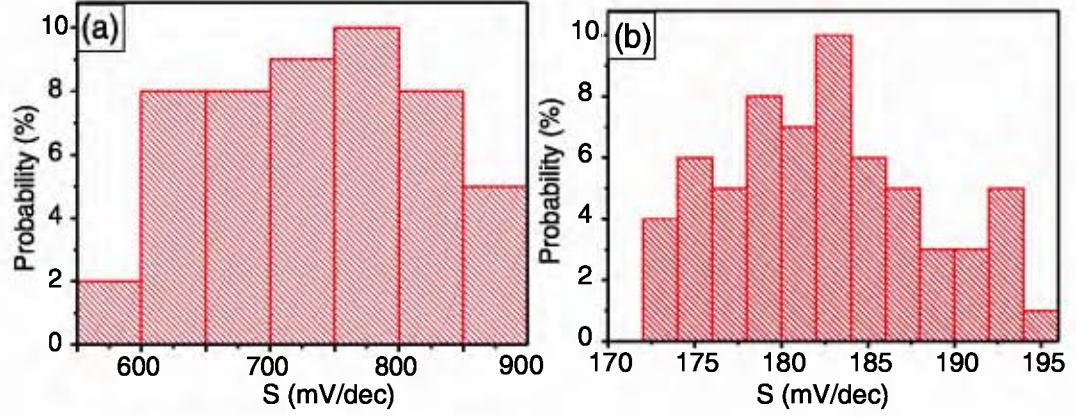
Figure 7.8: (a) Statistical distribution of S for devices with 24\text{nm} t_{ox} and thick channel. (b) Statistical distribution of S for devices with 3.7\text{nm} t_{ox} and 9\text{nm} channel thickness.
