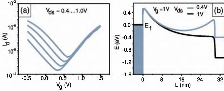
Figure 4.1: (a) Simulated transfer characteristics of a 30 nm SB-MOSFET with a SBH of 0.64eV, t_{ox}=2 nm, t_{si}=10 nm. (b) Energy band diagram in the channel for different source-drain voltages.
