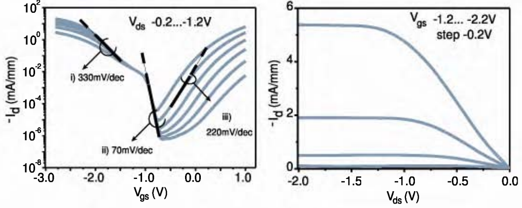
Figure 7.1: (a) Transfer characteristics of a SB-MOSFET at different V_{ds} . (b) Output characteristics at different V_{gs} . The device has a gate length of 2\mu\text{m} and gate oxide thickness t_{ox}=3.7\text{nm} and a channel thickness of t_{si}=50\text{nm} .
