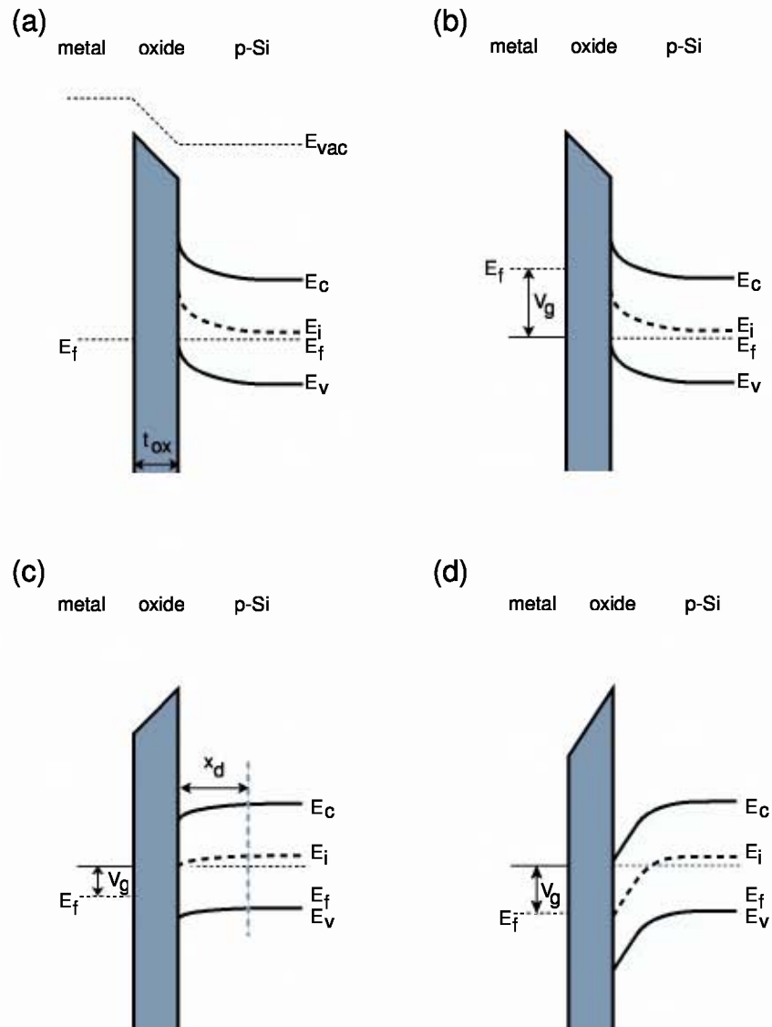
Figure 2.4: Effect of an applied voltage on a p -type MOS capacitor. (a) equilibrium, (b) accumulation, (c) onset of inversion, and (d) strong inversion.
