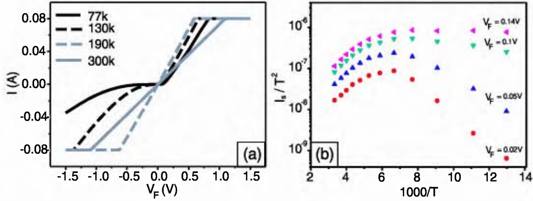
Figure 5.3: (a) Temperature dependent I - V_F characteristics of Schottky diodes with 5 \times 10^{14} \text{ cm}^{-2} As implantation. (b) Arrhenius plots for the extraction of the effective SBH.
