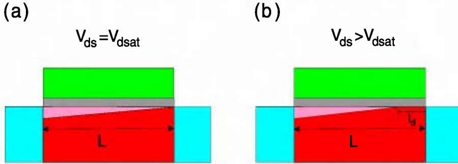
Figure 2.9: Schematic cross-section of a SB-MOSFET showing channel pinch-off as V_{ds} is increased (a) At the onset of saturation, the channel pinches off at the drain end and (b) the pinch-off point moves towards the source.
