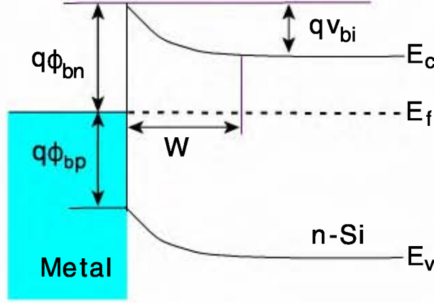
Figure 2.5: Schematic band-diagram of an ideal Schottky contact.
