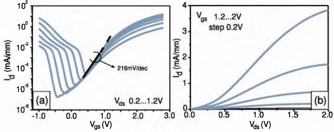
Figure 7.2: (a) Transfer characteristics of a SB-MOSFET at different V_{ds} . (b) Output characteristics at different V_{gs} . t_{ox}=3.7\text{nm} , t_{si}=50\text{nm} .
