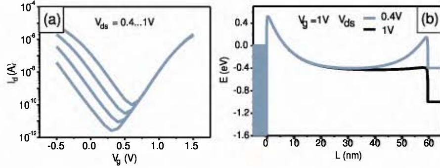
Figure 4.3: (a) Simulated transfer characteristics for a 60 nm SB-MOSFET with a SBH of 0.64eV, t_{ox}=2\text{nm} , t_{si}=10\text{nm} . (b) Energy band diagram in the channel for different source-drain voltages.
