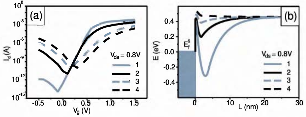
Figure 4.8: (a) Transfer characteristics of SB-MOSFETs with different dopant concentrations N_{seg} and segregation lengths. (b) Energy band diagram at gate voltage 0.1V. 1: N_{seg}=2 \times 10^{20}\text{cm}^{-3} , l_{seg}=4\text{nm} . 2: N_{seg}=2 \times 10^{20}\text{cm}^{-3} , l_{seg}=2\text{nm} . 3: N_{seg}=10^{20}\text{cm}^{-3} , l_{seg}=2\text{nm} . 4: N_{seg}=5 \times 10^{19}\text{cm}^{-3} , l_{seg}=2\text{nm} .
