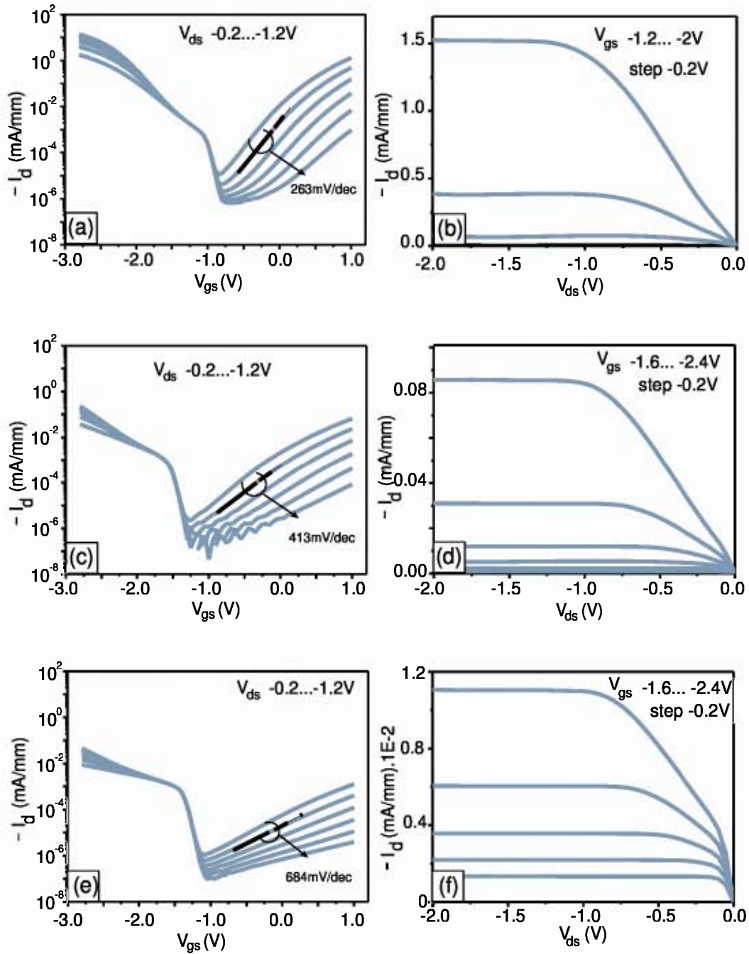
Figure 7.7: Transfer (a)-(c)-(e) and output (b)-(d)-(f) characteristics of devices with t_{ox}=6\text{nm} , 10\text{nm} and 16\text{nm} , respectively.
