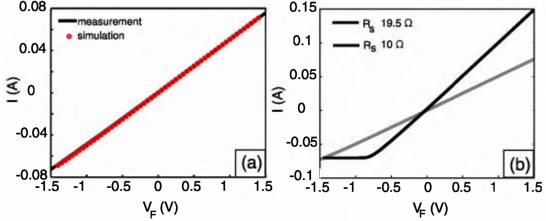
Figure 5.2: (a) Simulated and experimental I - V_F characteristics of NiSi/ n -Si (100) with 10^{14}\text{cm}^{-2} As implantation. The SBH is \phi_{bn}=0.37\text{eV} and the series resistance is R_s=19.5\Omega . (b) shows the impact of the series resistance on the I - V_F characteristics of a Schottky diode.
