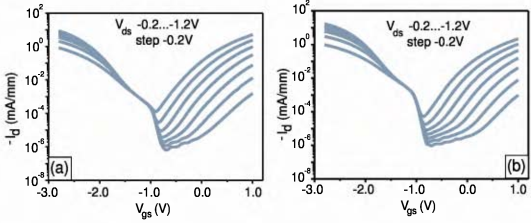
Figure 7.3: (a) Transfer characteristics of a SB-MOSFET at different V_{ds} with t_{ox}=3.7\text{nm} and t_{si}=50\text{nm} . (b) Transfer characteristics of a SB-MOSFET after source-drain exchange.
