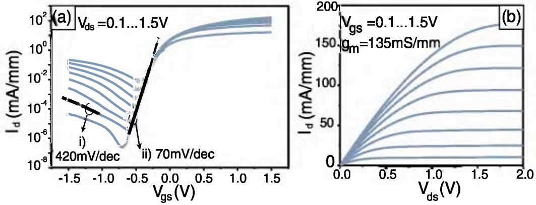
Figure 7.9: (a) Transfer characteristics and (b) Output characteristics of a SB-MOSFET with arsenic dopant segregation. Device has a channel length of L = 1\mu\text{m} and a channel width of W = 40\mu\text{m} . The device exhibits n -type characteristics with an inverse subthreshold slope in the n -branch close to the thermal limit.
