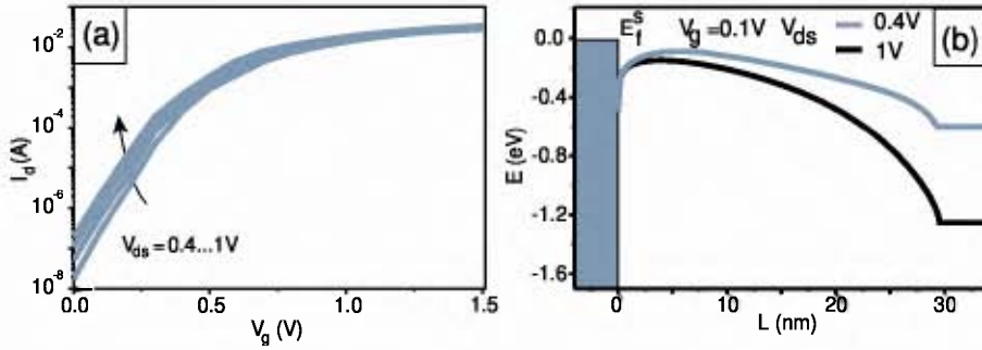
Figure 4.1: (a) Simulated transfer characteristics of a 30 nm SB-MOSFET with a SBH of 0.64eV, t_{ox}=2 nm, t_{si}=10 nm. (b) Energy band diagram in the channel for different source-drain voltages.
