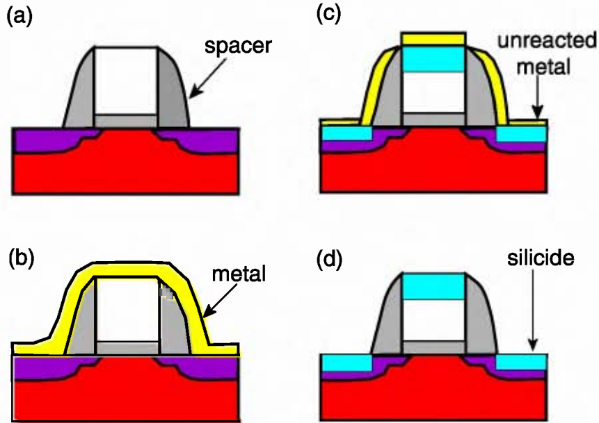
Figure 3.1: A typical salicide process. (a) MOSFET formation, (b) metal deposition, (c) silicidation by RTP annealing and (d) removal of unreacted metal.
