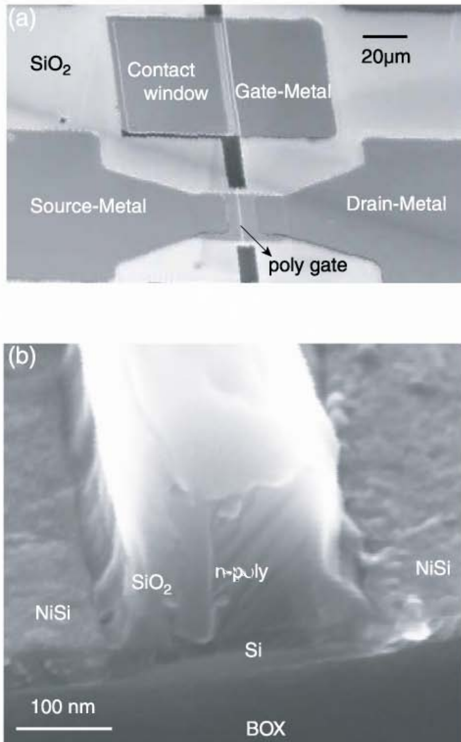
Figure 6.3: SEM images of a SB-MOSFET with a 100nm gate length.
