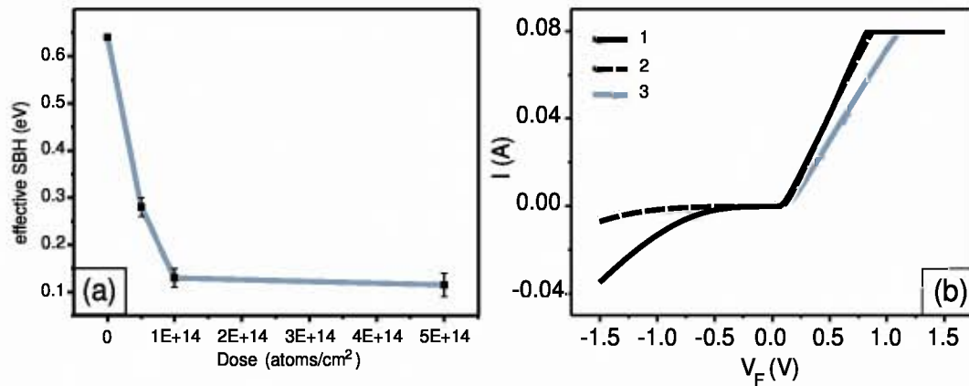
Figure 5.5: (a) Extracted effective SBH at different arsenic implantation doses. (b) I-V_F characteristics of the Schottky diodes with different implantation doses: 1: 5 \times 10^{14} \text{ cm}^{-2} , 500°C; 2: 10^{15} \text{ cm}^{-2} , 500°C; 3: 5 \times 10^{14} \text{ cm}^{-2} , 450°C.
