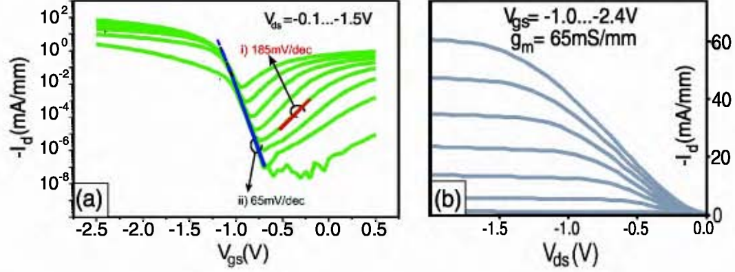
Figure 7.11: (a) Transfer and (b) output characteristics of a SB-MOSFET with boron dopant segregation. The device has a gate length of L = 1\mu\text{m} and a gate width of W = 40\mu\text{m} . The device exhibits p -type characteristics with an inverse subthreshold slope in the p -branch close to the thermal limit.
