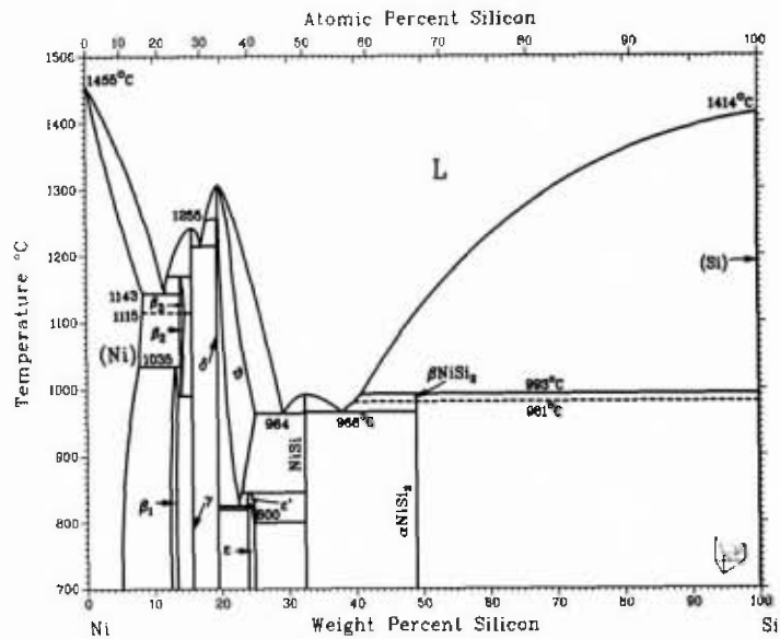
Figure 3.2: Nickel-Silicon phase diagram.
