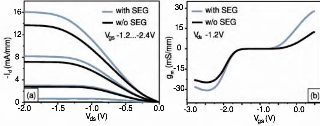
Figure 7.6: (a) Comparison of output characteristics of a device with and without selective epitaxy. (b) Transconductance comparison for device with and without selective epitaxy. The device has a gate oxide thickness of t_{ox}=3.7\text{nm} and a channel thickness of t_{si}=9\text{nm} .
