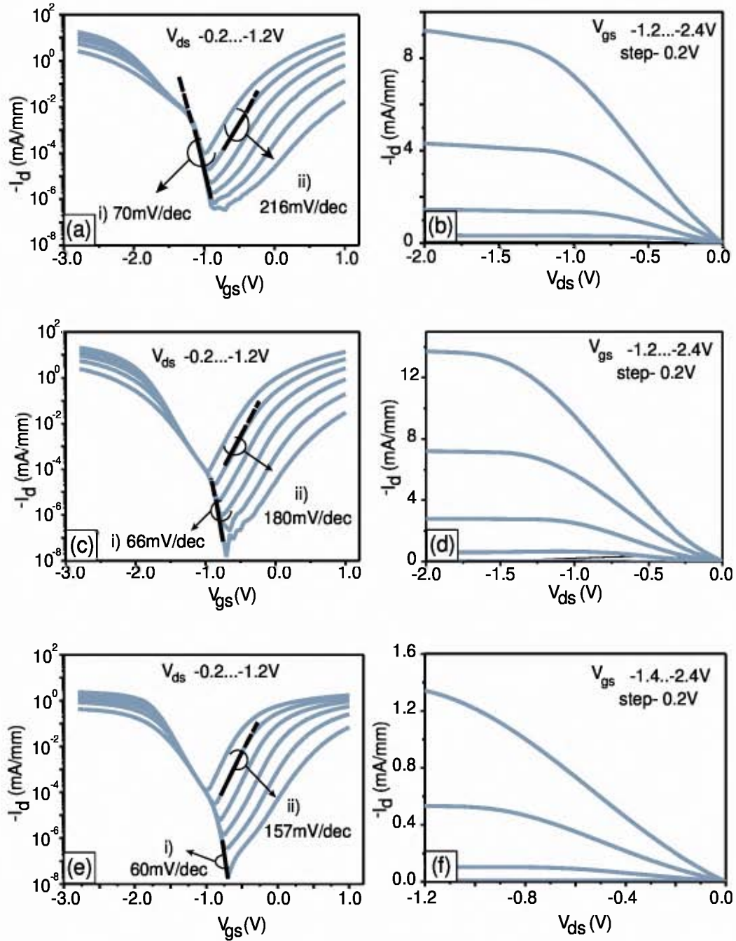
Figure 7.4: Transfer (a)-(c)-(e) and output (b)-(d)-(f) characteristics of devices with the same oxide thickness t_{ox} = 3.7\text{nm} but with varying t_{si} = 25\text{nm} , 9\text{nm} and 7\text{nm} . The gate length is 2\mu\text{m} .
