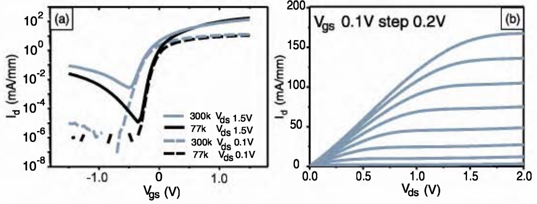
Figure 7.14: (a) Transfer characteristics of a SB-MOSFET with arsenic dopant segregation at different temperature and V_{ds} . (b) Output characteristics at 110K showing a sub-linear effect at low V_{ds} .
