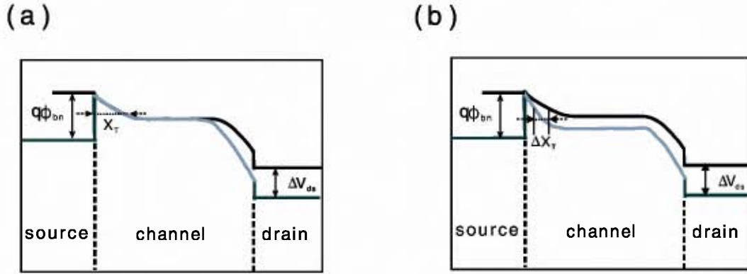
Figure 2.11: Energy band diagram of a SB-MOSFET with different negative V_{ds} . (a) small V_{ds} (b) large V_{ds} .
