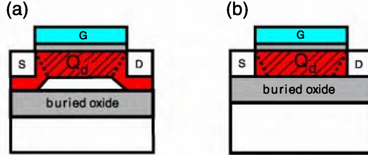
Figure 2.13: Partially depleted SOI MOSFET (a) versus fully depleted SOI MOSFET (b). Depicted is the depletion charge Q_d distribution which is controlled by the gate.
