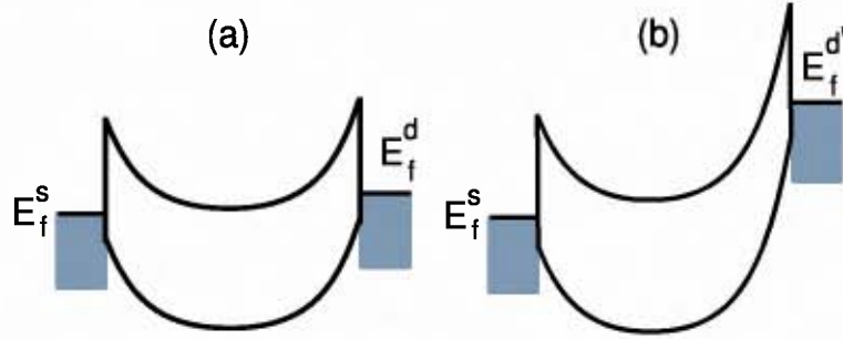
Figure 2.11: Energy band diagram of a SB-MOSFET with different negative V_{ds} . (a) small V_{ds} (b) large V_{ds} .
