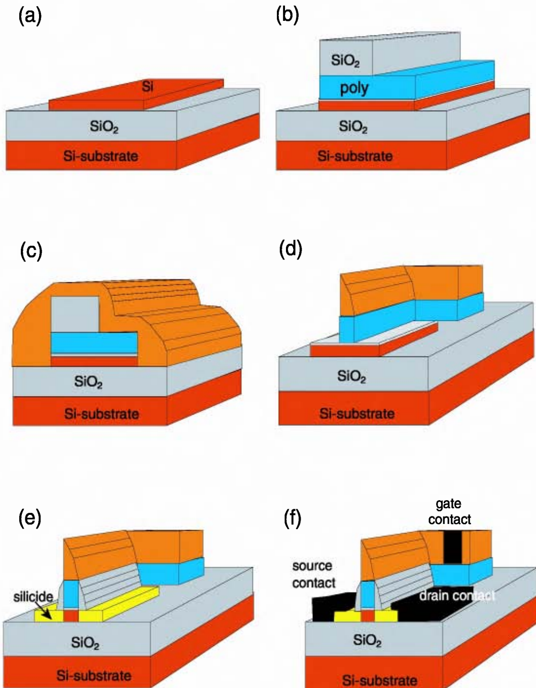
Figure 6.2: Schematic illustration of the fabrication process of short-channel SB-MOSFETs.
