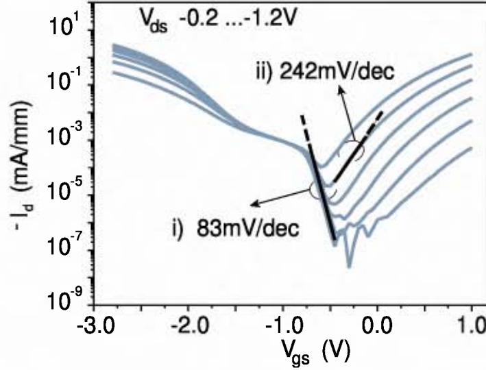
Figure 7.15: Transfer characteristics of a SB-MOSFET with L=100\text{nm} W=20\mu\text{m} .
