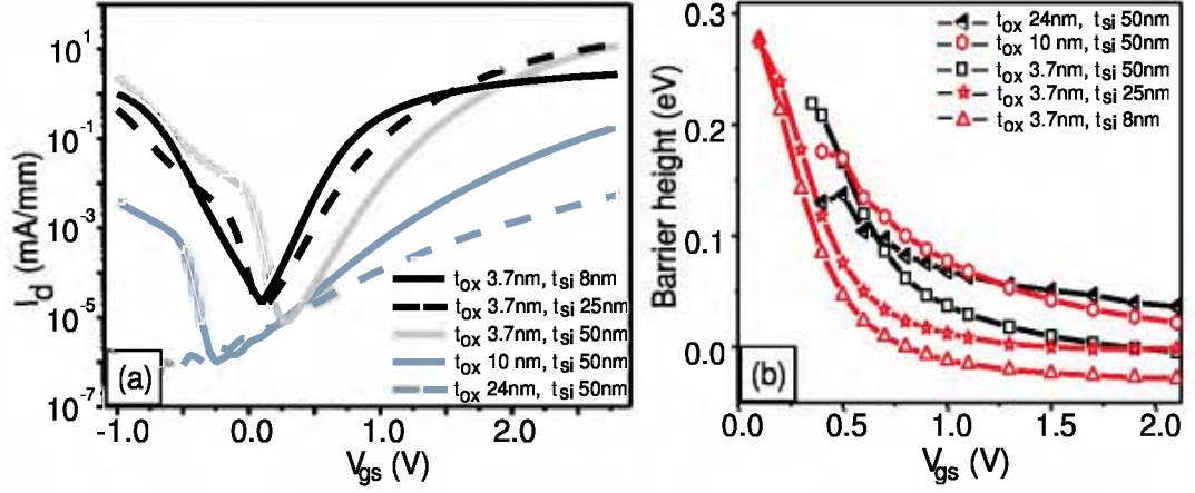
Figure 7.12: (a) I - V characteristics of SB-MOSFETs with different geometrical parameter sets at V_{ds}=1 V. (b) Extracted effective SBH for electrons based on the temperature dependent measurements.
