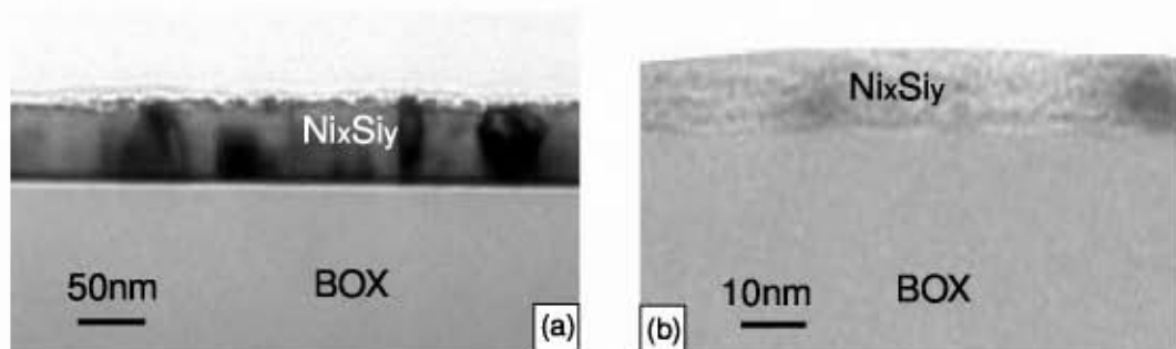
Figure 3.7: TEM image of a fully silicided layer on (a) 50nm SOI and (b) 10nm SOI.
