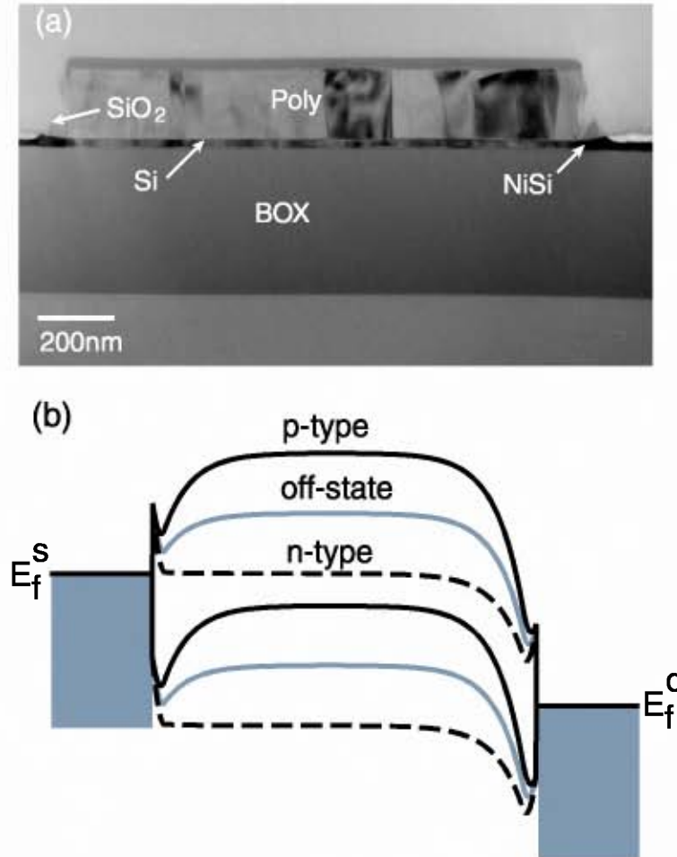
Figure 7.10: (a) TEM image of a fabricated SB-MOSFET with dopant segregation at the silicide/Si interface. (b) Energy band diagram for a SB-MOSFET with dopant segregation under three different gate voltages and a drain voltage of 1V.
