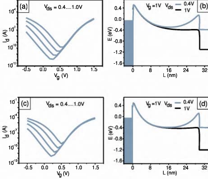
Figure 4.4: (a) Transfer characteristics of a 30 nm SB-MOSFET at different V_{ds} with a SBH of 0.64eV, t_{ox}=2 nm, t_{si}=6 nm. (b) Barrier lowering becomes less as compared to Fig. 4.1. (c) t_{ox}=1 nm, t_{si}=6 nm. (d) The minimum potential in the conduction band no longer depends on V_{ds} .
