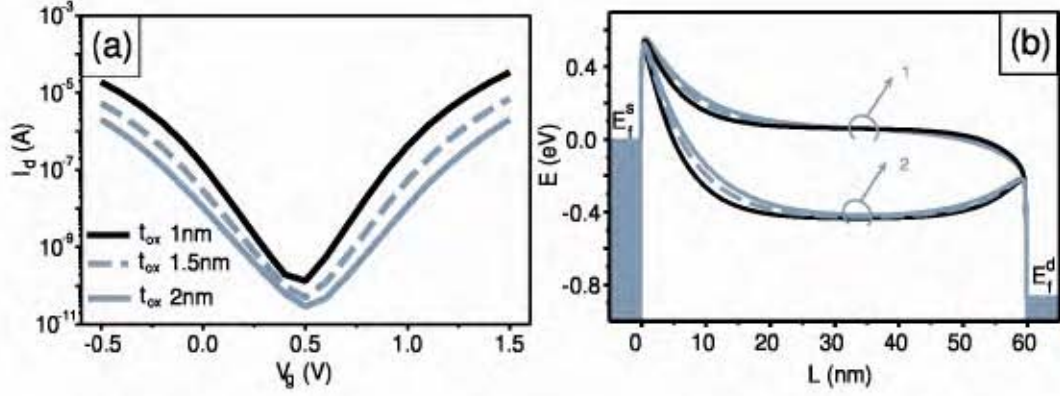
Figure 4.5: (a) Transfer characteristics for a 60 nm SB-MOSFET at V_{ds} 0.8V with SBH 0.64eV, t_{si}=10\text{nm} but different t_{ox} . (b) Energy band diagram for off-state (1) and on-state (2).
