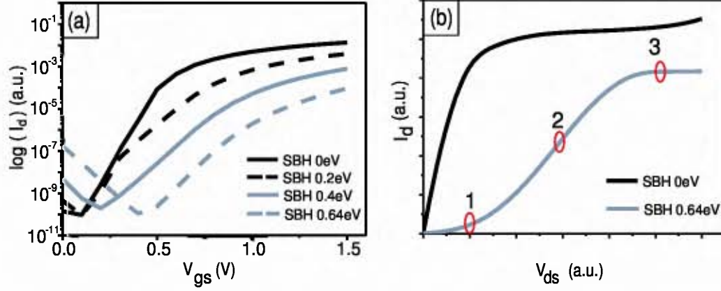
Figure 2.8: Transfer (a) and output (b) characteristics of a long-channel SB-MOSFET with different SBH. 1. Sub-linear region; 2. Linear region; 3. Saturation region.
