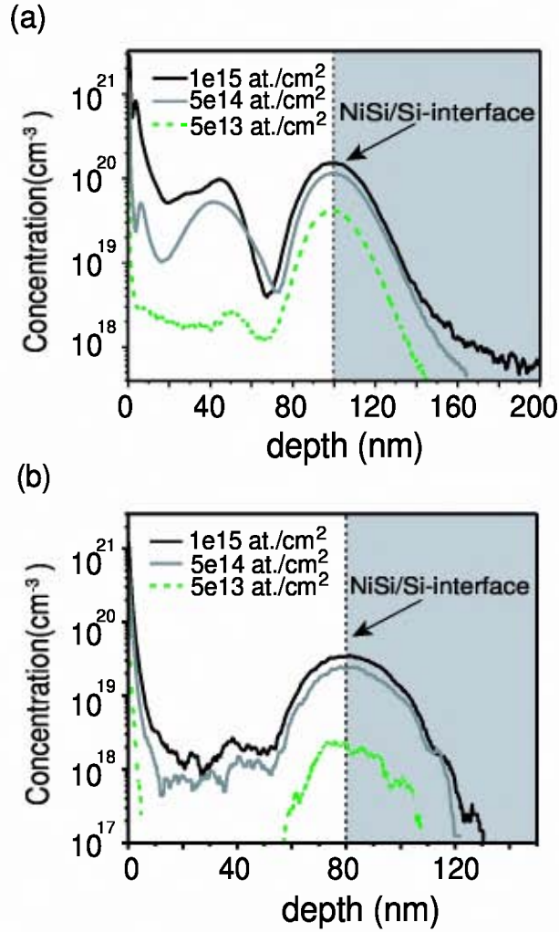
Figure 3.8: (a) As segregation at the NiSi/Si interface and (b) B segregation at the NiSi/Si interface. Three different implantation doses were investigated.
