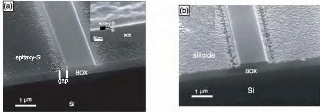
Figure 6.5: (a) SEM of an elevated source-drain test structure. The inset shows a magnification after selective epitaxy, Si thickness increases from 9nm to 30nm (b) SEM photograph after silicidation of an elevated source-drain structure.
