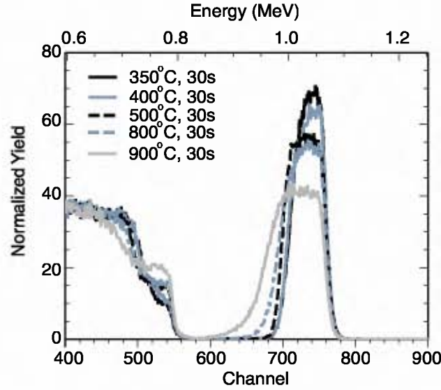
Figure 3.5: RBS spectra of nickel silicide film on silicon substrate at different annealing temperatures.
