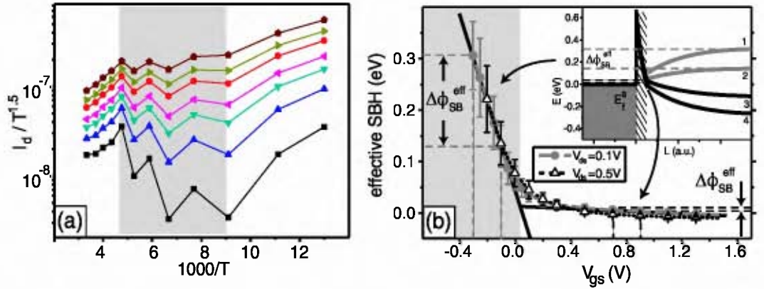
Figure 7.13: (a) Typical Arrhenius plots used for extraction of effective SBH (shaded area 210K-110K). (b) Extracted effective SBH as a function of V_{gs} at V_{ds}=0.1 V (gray circles) and 0.5 V (triangles) for electron injection; the error bars result from the uncertainty in determining the slope from the Arrhenius plots. The SBH exhibits a one-to-one change (see the slope in the shaded area) with increasing V_{gs} in the subthreshold region, but a much smaller in the strongly-on region. The inset shows calculated conduction band profiles in the subthreshold region (1, 2) and in the device's on-state (3, 4) for two different V_{gs} .
