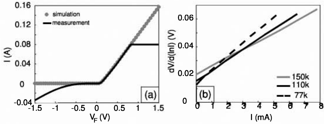
Figure 5.4: (a) Simulated and experimental results of a Schottky diode with 5 \times 10^{14} \text{ cm}^{-2} arsenic implantation measured at 77K. (b) The experimental dV/d(\ln I) versus I plot at different temperatures.
