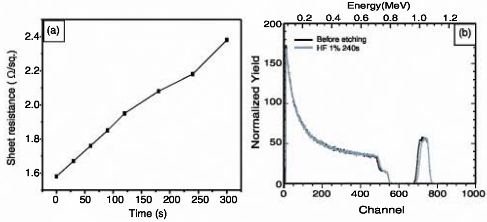
Figure 6.7: (a) The sheet resistivity of a nickel silicide film etched in DHF versus etching time. (b) RBS spectra before DHF and after 240s DHF etch.
