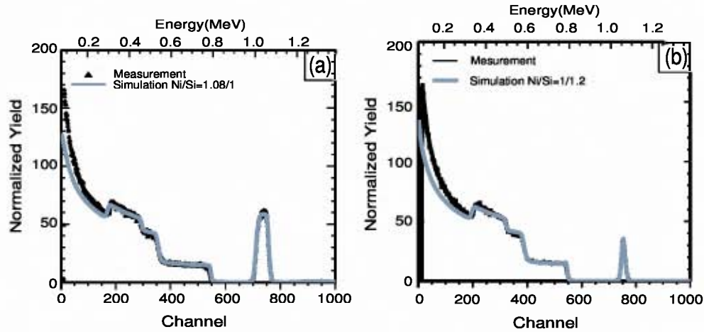
Figure 3.6: RBS spectra of nickel silicide layers formed on (a) 50nm SOI (b) 10nm SOI.
