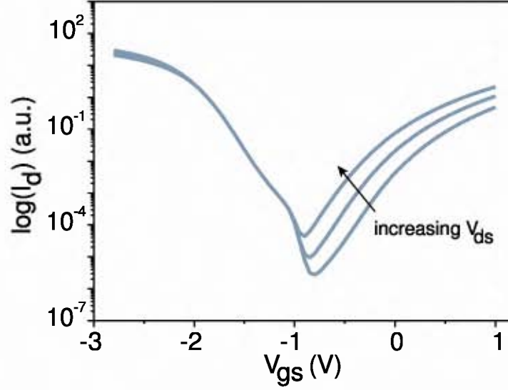
Figure 2.10: Transfer characteristics of SB-MOSFET with different negative V_{ds} .
