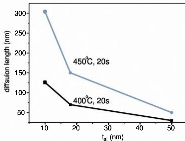
Figure 3.10: Lateral \text{Ni}_x\text{Si}_y growth under the gate spacer and into the channel versus SOI thickness for two annealing conditions.
