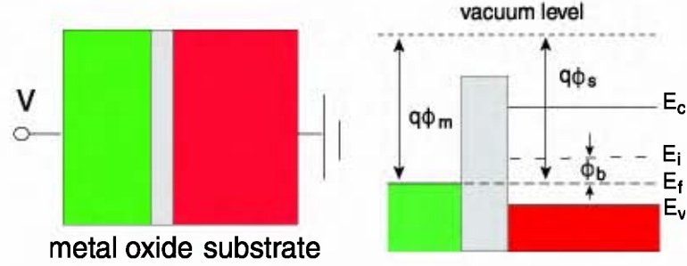
Figure 2.2: The MOS capacitor.
