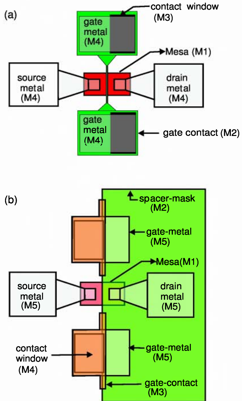
Figure 6.1: Schematic illustration of the mask layout for the fabrication of (a) long-channel SB-MOSFETs and (b) short-channel SB-MOSFETs.
