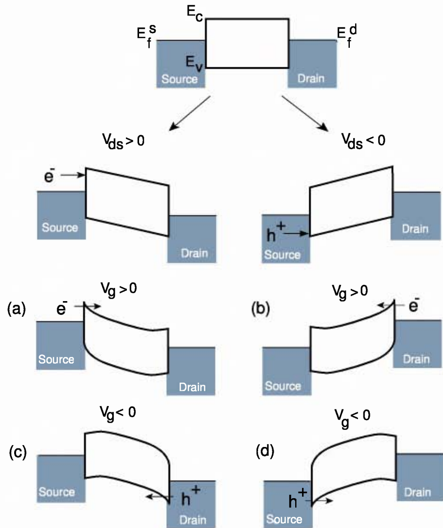
Figure 2.7: Schematic energy band diagrams to demonstrate the operating principle of SB-MOSFETs. (a)-(b) nMOS; (c)-(d) pMOS.
