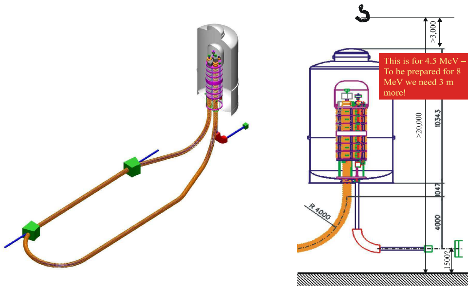
Fig. 32: Planned geometry of the electron cooler. Stability of the electron beam is monitored with a particle beam (third outlet of the high voltage tower). Shown are the dimensions for 4.5 MeV. In case of 8 MeV the tank height has to be extended by 3 m. 30 m of installation space in the cooler straight of HESR is required.
