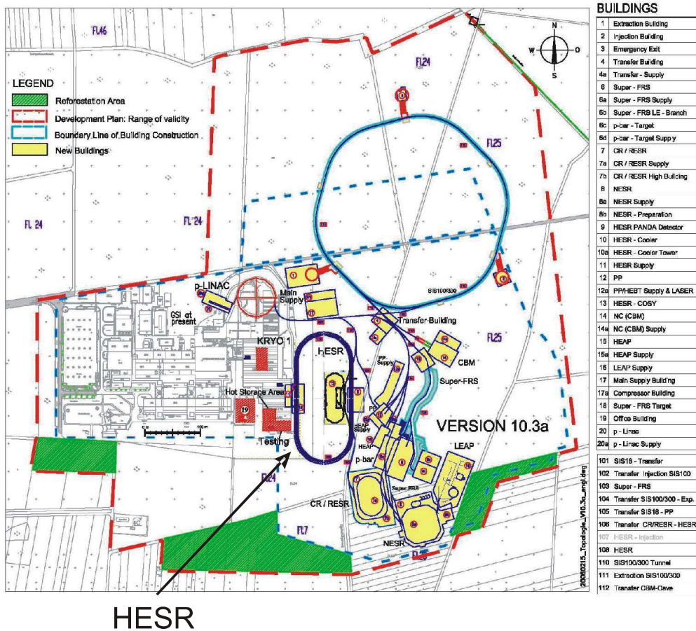
Fig. 31: FAIR topology including buildings. Left hand side: existing GSI facility. The position of HESR is indicated.
