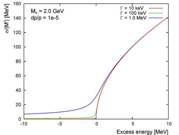
Fig. 36: Energy dependence of the simulated D_{sJ}^*(2317)^+ D_{sJ}^*(2317)^- cross section for 10^{-5} relative momentum spread of the antiproton beam.
