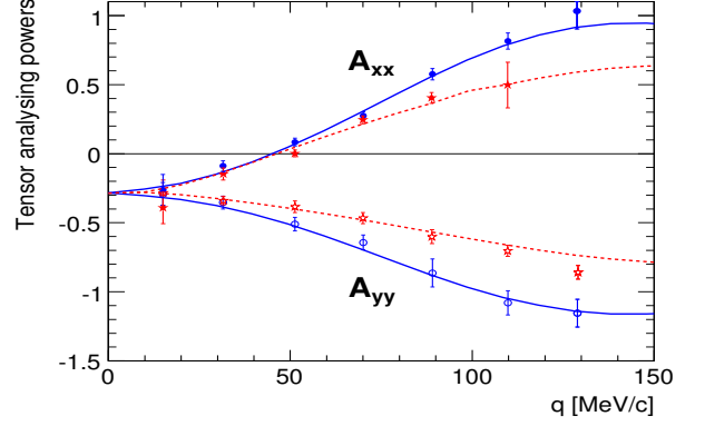
Fig. 6: Values of the tensor analysing powers A_{yy} and A_{xx} extracted for the dp \rightarrow (pp)n reaction for 0 < E_{pp} < 1 MeV (circles) and 1 < E_{pp} < 3 MeV (stars). The curves correspond to the predictions of the impulse approximation program, for which the input amplitudes at 585 MeV were taken from SAID; 0 < E_{pp} < 1 MeV (solid) and 1 < E_{pp} < 3 MeV (broken).
