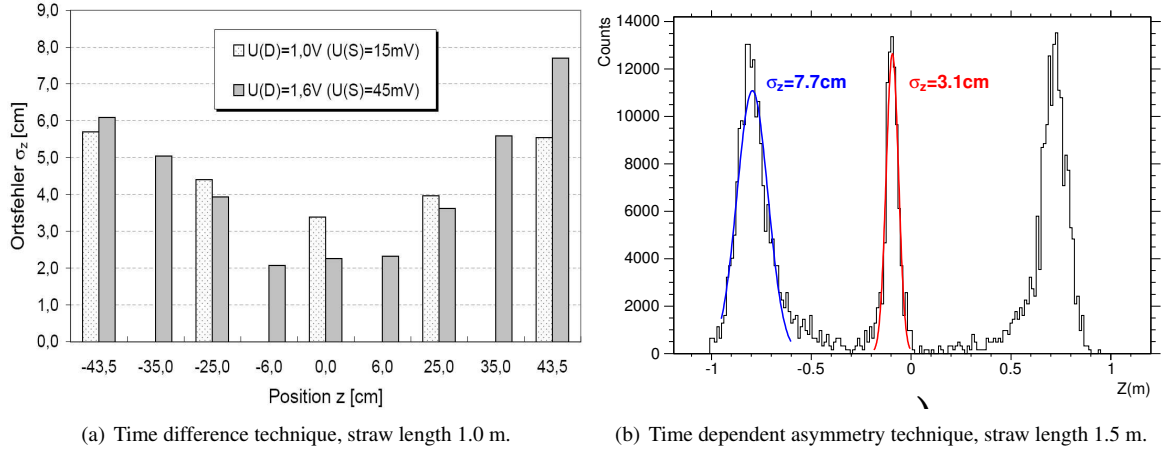
Fig. 35: Resolutions along the straw axis illuminated with ^{90}\text{Sr}/^{90}\text{Y} using different z-position reconstruction techniques for a double sided readout; the two measurements in the left plot represent two settings of the preamplifiers.
