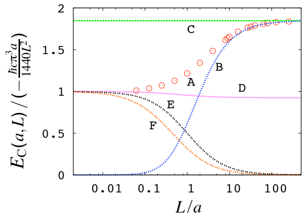
Fig. 19: Predictions for the scalar Casimir energy \mathcal{E}_C(a, L) of the Dirichlet sphere-plate configuration divided by the leading scale -\hbar c \pi^3 a / 1440 L^2 as function of the separation L between the surfaces in units of the radius a of the sphere. Circles (A) represent the exact data for the sphere-plate system, curve (B) shows the s -wave approximation, line (C) represents the predicted asymptotic limit 2 \times 90/\pi^4 , where 90/\pi^4 is the asymptotic value of the semiclassical Gutzwiller formula including all repeats of the two-bounce periodic orbit (see line D). Curves (E) and (F) display the results of two different Ansätze for the proximity-force approximation.
