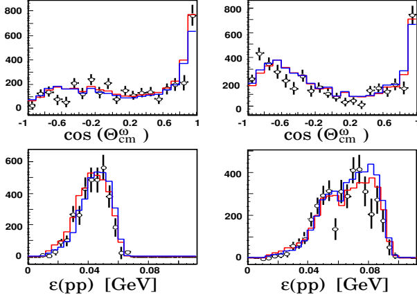
Fig. 5: Differential distributions of pp \rightarrow pp\omega events along the the \omega center-of-mass angle \Theta_{\text{cm}}^{\omega} and along the relative kinetic energy \varepsilon(pp) of two protons obtained at Q = 60 MeV (left column) and at Q = 92 MeV. Phase-space simulations assuming an isotropic angular distribution of the two protons are shown by red lines. The blue lines correspond to a \cos^2(\Theta_{\text{cm}}^{pp}) angular dependence.
