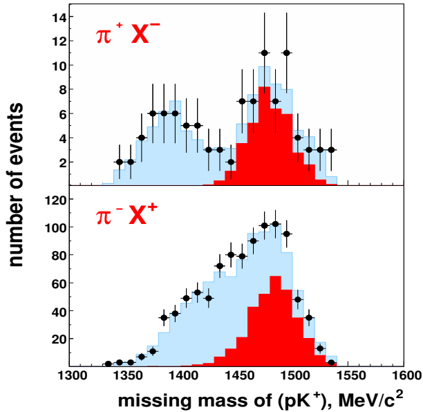
Fig. 2: Missing-mass MM(pK^+) spectra for the reaction pp \rightarrow pK^+\pi^+X^- (upper) and pp \rightarrow pK^+\pi^-X^+ (lower). Experimental data points with statistical errors are compared to the fitted overall Monte-Carlo simulations (shaded histogram, blue). The contribution from the Y^{0*} resonance with a mass of M(Y^{0*}) = (1480 \pm 15) \text{ MeV}/c^2 and a width \Gamma(Y^{0*}) = (60 \pm 15) \text{ MeV}/c^2 is shown as a solid (red) histogram.
