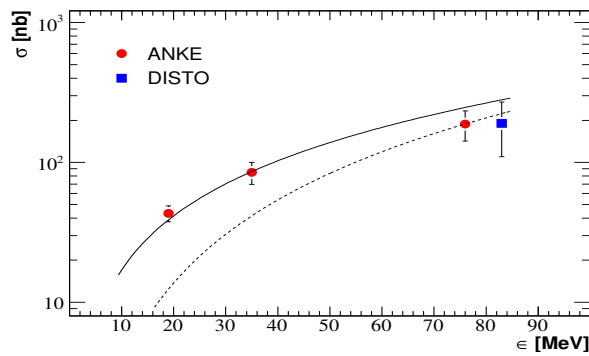
Fig. 4: Total cross section for \phi -meson production in pp collisions as a function of the excess energy Q . The error bars include both statistical and systematic uncertainties. The dashed line shows a phase-space calculation, fixed to the high energy ANKE result, while the solid line includes proton-proton final-state interaction and is normalized to fit all ANKE data.
