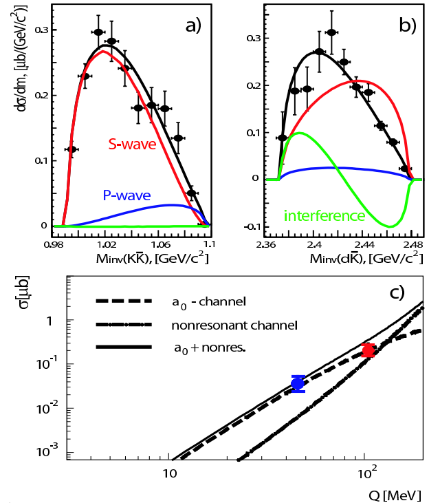
Fig. 3: K\bar{K} (a) and d\bar{K} (b) invariant mass distributions for the reaction pp \rightarrow dK^+\bar{K}^0 at Q = 105 \text{ MeV} . The lines denote a partial wave decomposition with the K\bar{K} pair in a relative S - and P -wave, respectively. Total cross section (c) as a function of Q in comparison with theoretical predictions for a_0^+ production and non-resonant background.
