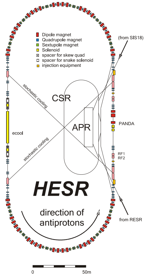
Fig. 30: Schematic layout of the HESR lattice. Equipment for experiment, stochastic and electron cooling, compensation solenoids, and injection are included. Possible locations of a future Antiproton Polariser Ring (APR) and a Cooler Synchrotron Ring (CSR) for polarised antiprotons are indicated.
