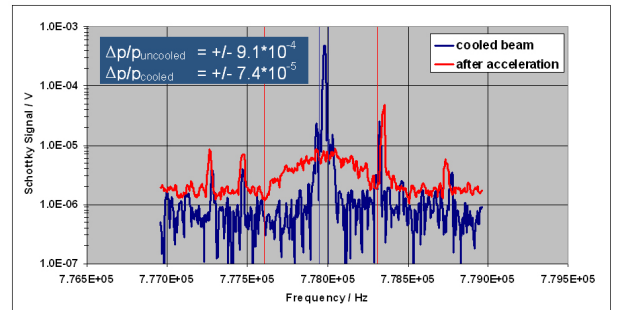
Fig. 23: Reduction of the momentum spread of protons after acceleration to 508 MeV/c with electron cooling, using an electron energy of 70 keV.
