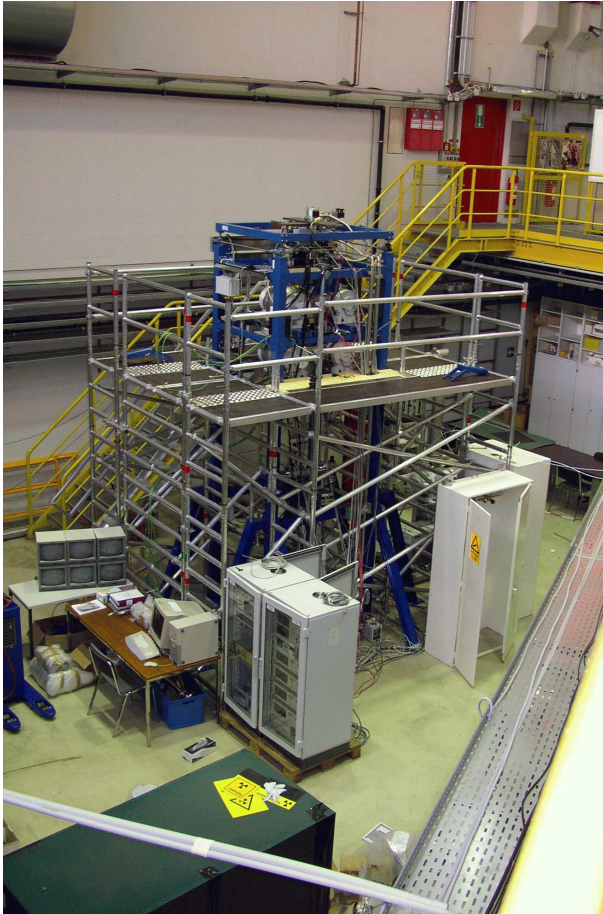
Fig. 9: Test setup of the WASA pellet target at COSY with pellet generator (top), a dummy vacuum chamber around the nominal interaction zone, and pellet beam dump (bottom).
