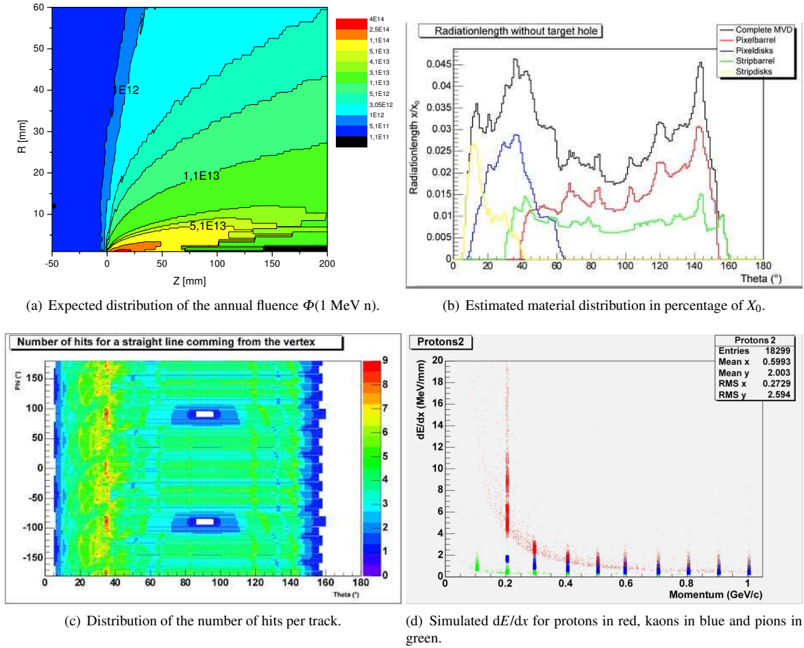
Fig. 34: Selected simulation results for 10^7 \bar{p}p -annihilations per sec. at 15 GeV/c with the PANDA MVD .
