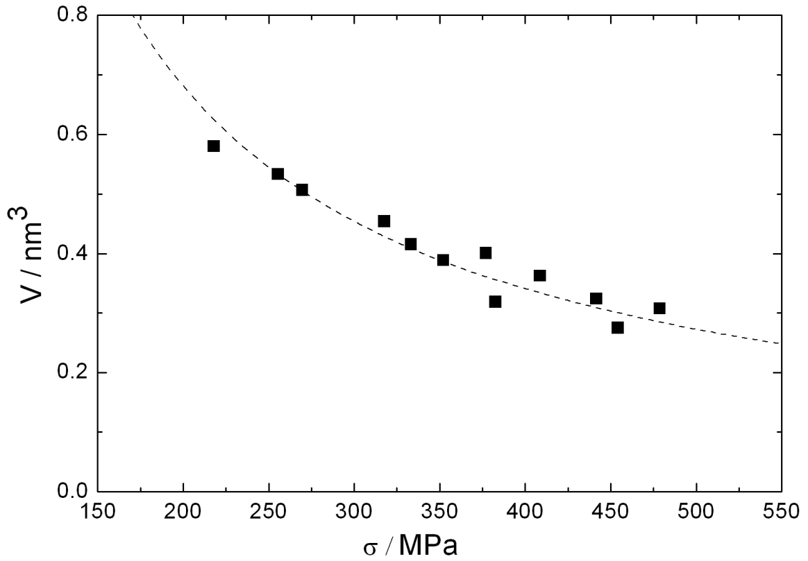
Figure 5.6: Activation volume V of \text{Mg}_{32}(\text{Al,Zn})_{49} , evaluated from stress-relaxation experiments, as a function of stress \sigma . The dashed curve is a fit which follows the hyperbolic function V = 136/\sigma .
