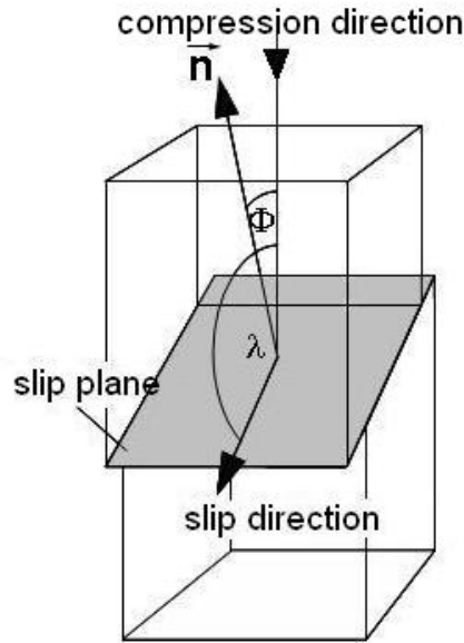
Figure 3.5: The orientation of the slip system with respect to the compression direction defines the Schmid factor m_s . It is calculated from the angles between compression direction and slip-plane normal \Phi and compression direction and slip direction \lambda , respectively.
