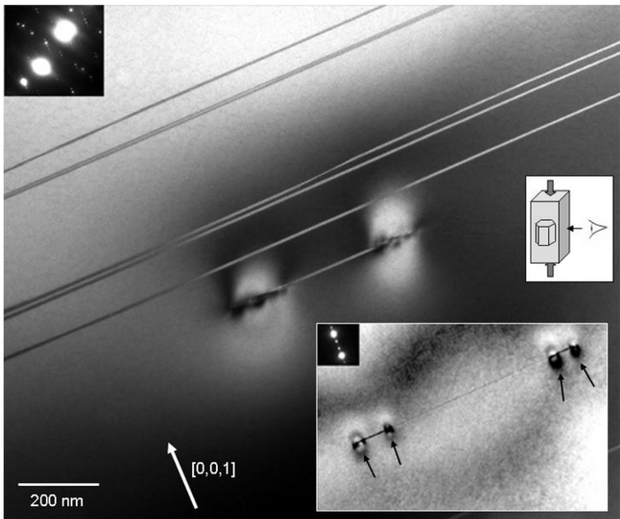
Figure 4.18: TEM micrograph close to the [1,\bar{1},0] zone axis using a two-beam condition with \vec{g} = (5,3,\bar{6}) . Several stacking faults and a dislocation loop in edge-on orientation are visible. The inset in the lower-right corner shows the loop in almost end-on orientation using \vec{g} = (0,0,12) . Each segment is split into two partial dislocations (black arrows).
