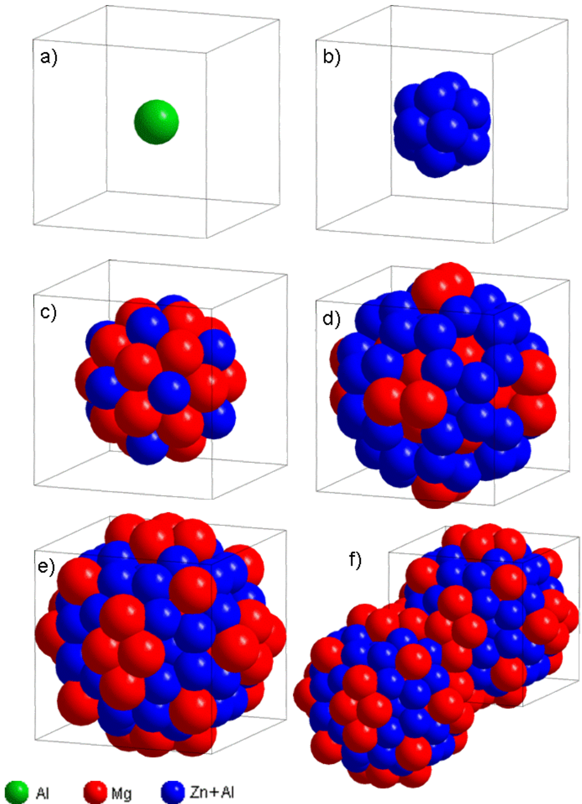
Figure 5.2: Successive atom-shell structure of the Bergman cluster (a-e) at the body-centred position of the \text{Mg}_{32}(\text{Al,Zn})_{49} unit cell (grey cubic frame). (f) Bergman clusters at centre and one corner position of the unit cell.
