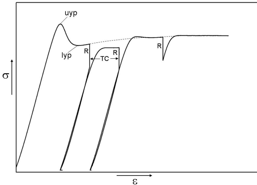
Figure 3.8: Exemplary stress-strain curve of a deformation experiment, illustrating the sequence of conducted stress-relaxation tests “R” and temperature changes “TC”. The upper- and the lower- yield point of the deformation behaviour are indicated “uyp” and “lyp”, respectively. The dashed line denotes the interpolated course of the curve.
