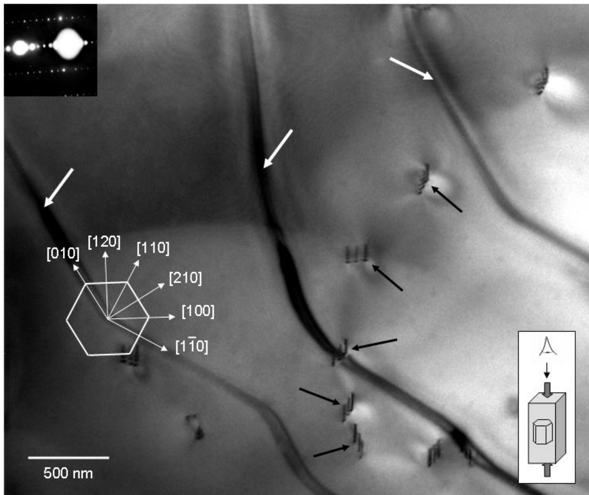
Figure 4.16: TEM micrograph close to the [0,0,1] zone axis. Parts of faceted dislocation loops with (0,0,1) habit planes are visible as long dark lines (white arrows). Facets have line directions parallel to \langle 1,0,0 \rangle or \langle 1,\bar{1},0 \rangle directions as indicated by the inset on the left-hand side. c-axis dislocations are also visible (black arrows).
