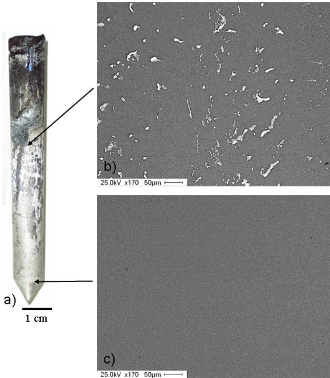
Figure 2.7: (a) \text{Mg}_{32}(\text{Al,Zn})_{49} crystal grown by means of the Bridgman technique. (c) SEM micrograph of a crystal part solidified in an early stage of the growth process. One homogenous solid phase is visible (Bergman phase). (b) SEM micrograph of a crystal part solidified in a later stage of the growth, where solidification of a secondary phase (bright contrast) has set in.
