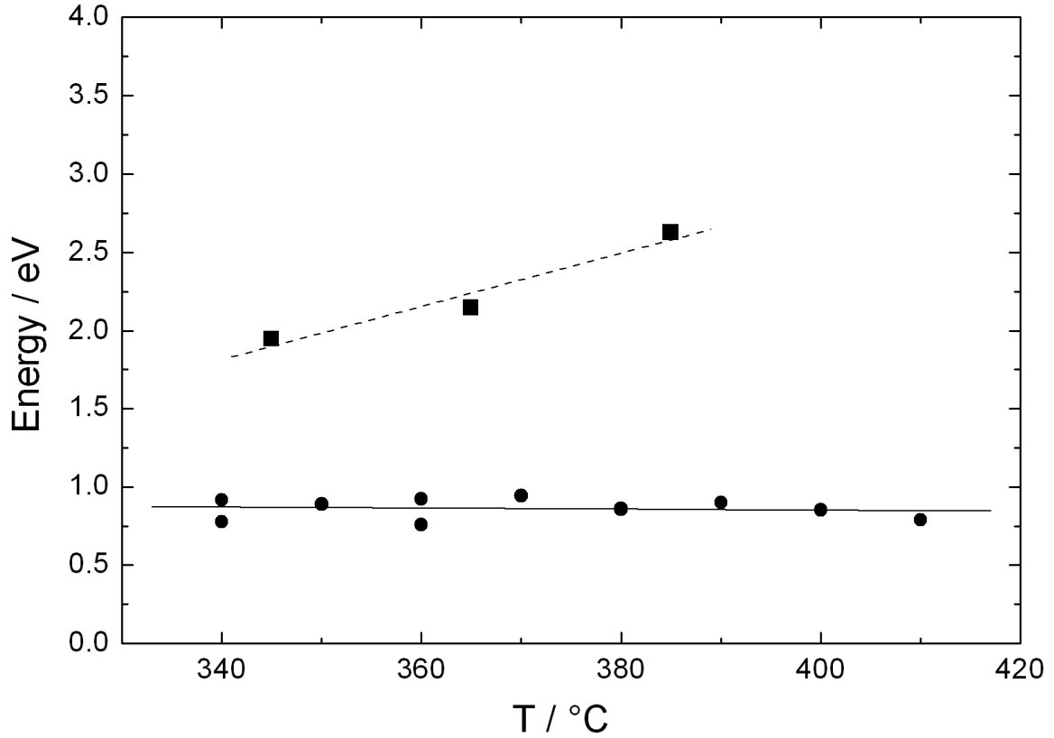
Figure 5.7: Activation enthalpy \Delta H (squares) and work term \Delta W (circles) of \text{Mg}_{32}(\text{Al,Zn})_{49} as a function of temperature. The dashed and solid lines are linear fits of the activation enthalpy and the work term, respectively.
