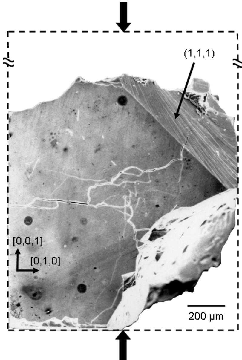
Figure 6.7: Fragment of a \beta -Al-Mg sample featuring a smooth (1,1,1)-fracture surface after deformation testing (deformed at 200 °C). The compression direction (large black arrows) corresponded to the [0,0,1] direction. The initial sample shape is indicated by the dashed line.
