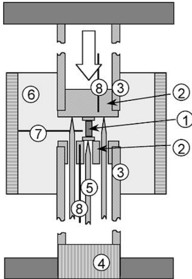
Figure 3.9: Schematic setup of the Zwick Z050 deformation machine; for explanations see text.
