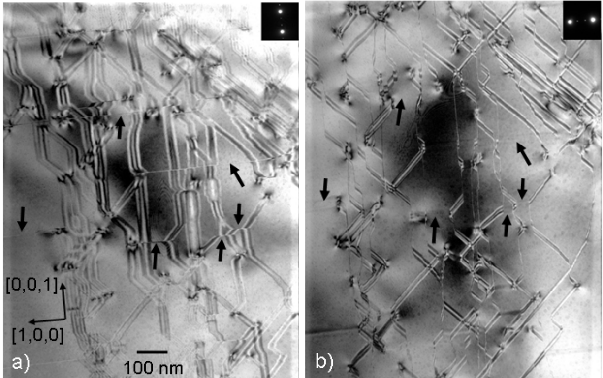
Figure 5.14: TEM micrograph of a specimen with orientation close to the [0,1,0] zone axis using the reflections \vec{g} = (0,0,\bar{6}) (a) and \vec{g} = (\bar{6},0,0) (b). Stacking faults with [0,0,1] normal vectors (black arrows) are extinct in (b).
