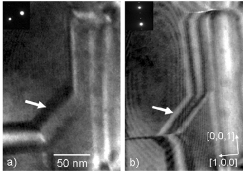
Figure 5.16: Stacking faults in a TEM specimen close to the [0,1,0] zone axis using two-beam conditions with \vec{g} = (5,0,3) (a) and \vec{g} = (0,0,\bar{6}) (b). A stacking fault with displacement vector along [\bar{1},0,6] is indicated by a white arrow.
