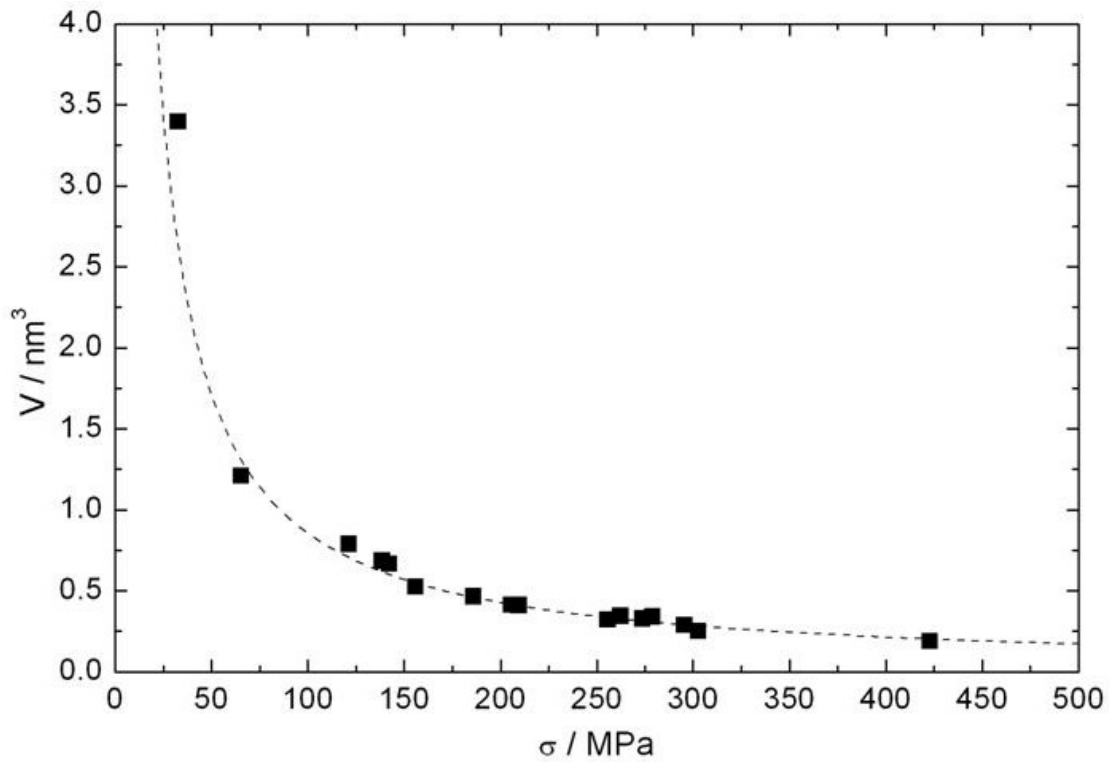
Figure 4.9: Activation volume V of \mu -Al-Mn, evaluated from stress-relaxation experiments, as a function of stress \sigma . The dashed curve follows the hyperbolic function V = 85.5 / \sigma .
