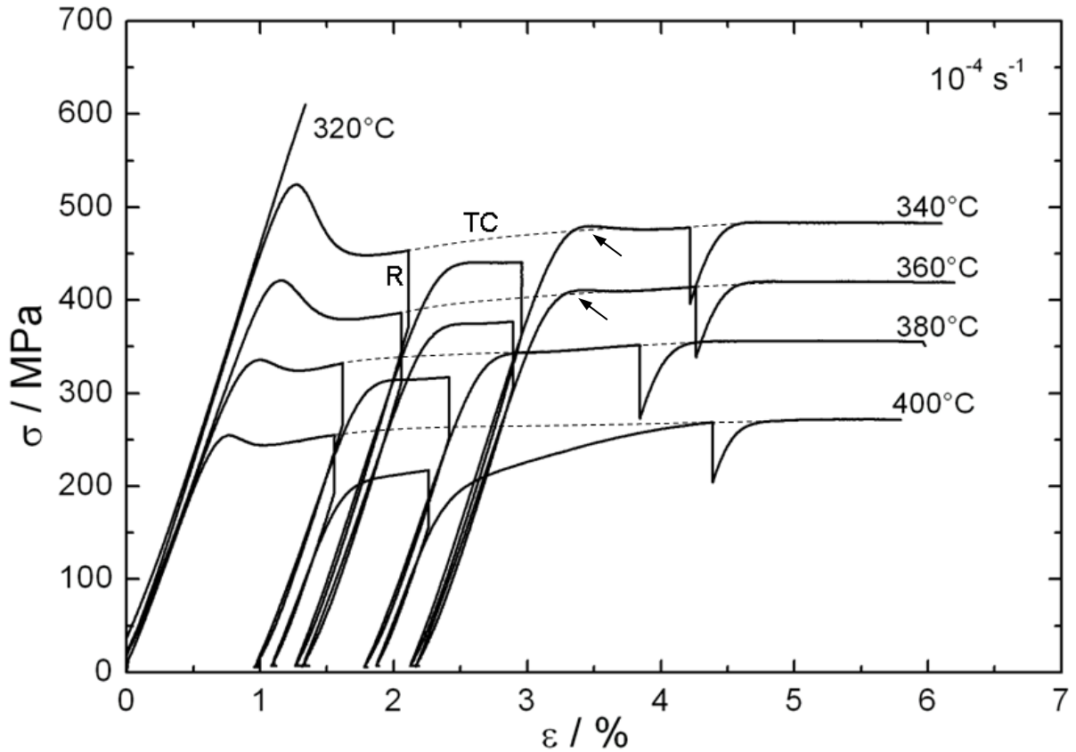
Figure 5.4: Stress-strain curves of \text{Mg}_{32}(\text{Al},\text{Zn})_{49} at temperatures between 320 and 400 °C at a strain rate of 10^{-4} \text{ s}^{-1} . A stress relaxation test and a temperature change are exemplary labelled “R” and “TC”. Interpolated courses of the stress-strain curves are shown as dashed lines. Arrows indicate small stress overshoots.
