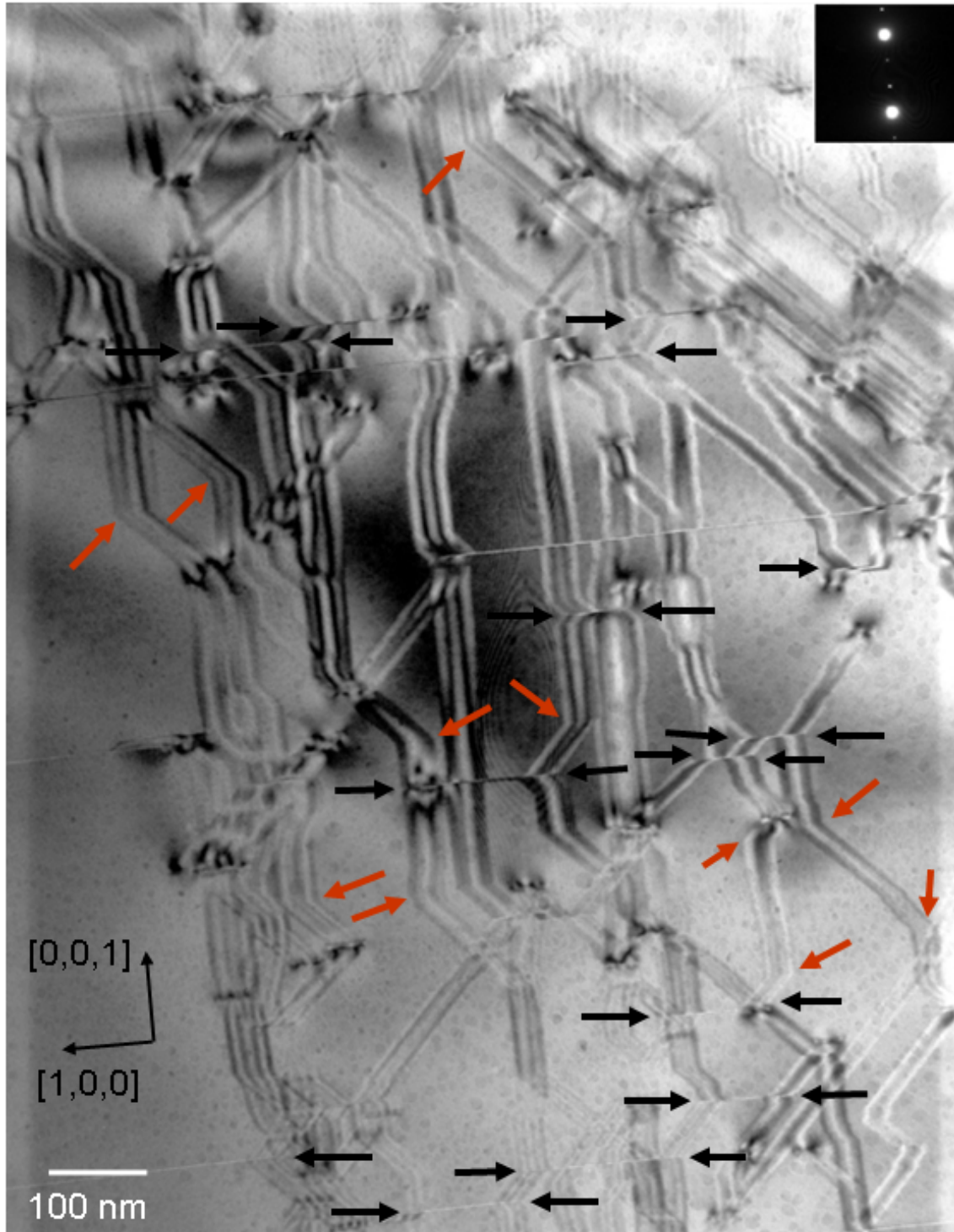
Figure 5.10: TEM micrograph with optical axis close to the [0,1,0] zone axis of the specimen. A two-beam condition corresponding to the reciprocal vector \vec{g} = (0,0,\bar{6}) was applied. Red arrows indicate sites where dislocations changed their habit planes during motion. Black arrows indicate sites where (0,0,1)-stacking faults terminate (see text).
