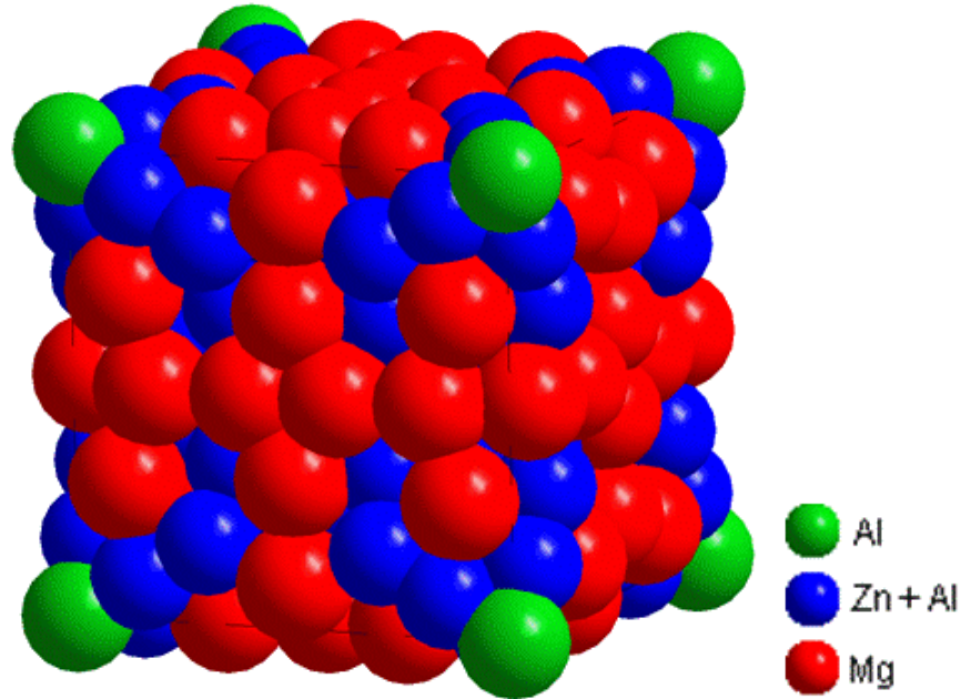
Figure 5.1: Unit cell of \text{Mg}_{32}(\text{Al,Zn})_{49} according to the model of Bergman et al. (1952).
