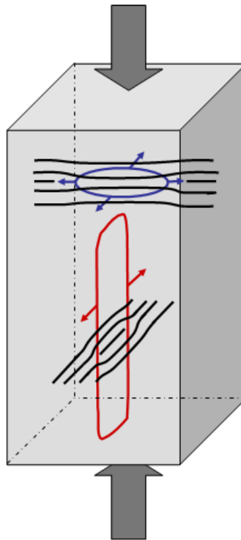
Figure 4.22: Schematic illustration of dislocations in \mu -Al-Mn. c-axis and basal-plane dislocations are indicated red and blue, respectively. The coloured arrows denote the respective climb direction. Black lines represent atomic layers. Grey arrows indicate the compression direction.
