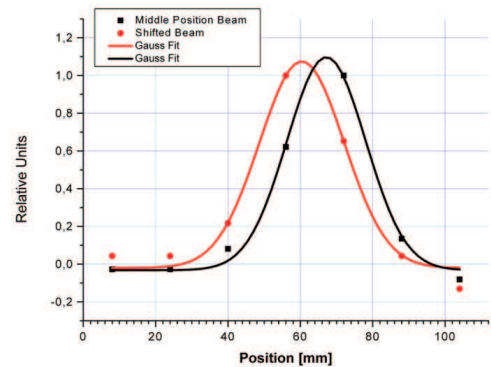
Fig. 3: Beam profiles in initial position (black) and shifted one (red).
