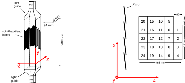
Fig. 1: In the left part a single module of the neutron detector and in the right the COSY – 11 neutron detector arrangement with VETO scintillators are depicted. Direction of the 'z' axis is the direction of the beam.
