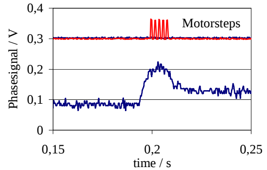
Fig. 2: Stepper motor control after a 10Hz jump of the generator frequency
