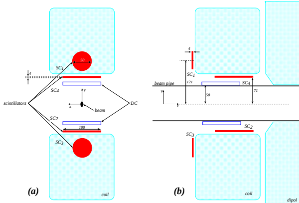
Fig. 1: Schematic view of the detection subsystem for registration of the elastically scattered events in the polarisation plane. (a) Front view. (b) Side view.
