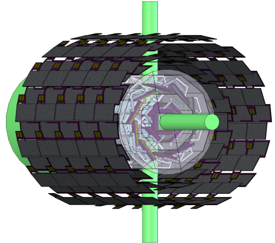
Fig. 1: Side view of the MVD without forward disks
