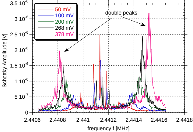
Fig. 1: Longitudinal beam spectrum at the 5 th revolution harmonic of an electron-cooled beam for different numbers of stored protons at injection energy. Besides the double peaks marked with arrows the spectrum contains also sharp lines resulting from transverse beam oscillations.
