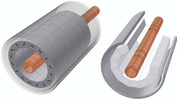
Fig. 1: Assembly of the magnetic quadrupole (left side) surrounding the Penning trap. On the right side the normal set-up with BGO detector is shown which was replaced by a permanent magnet with an inner diameter of 58 mm.
