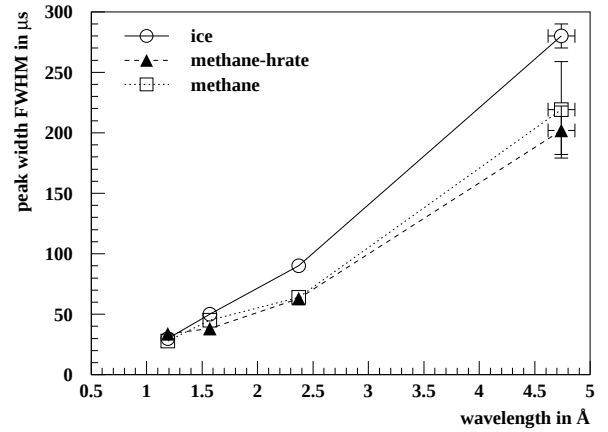
Fig. 2: Comparison of the peakwidth in FWHM for methane, ice, and methane-hydrate.
