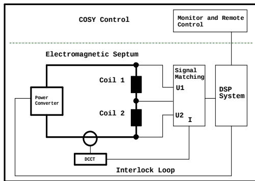
Figure 1: Schematic of the septum circuit
