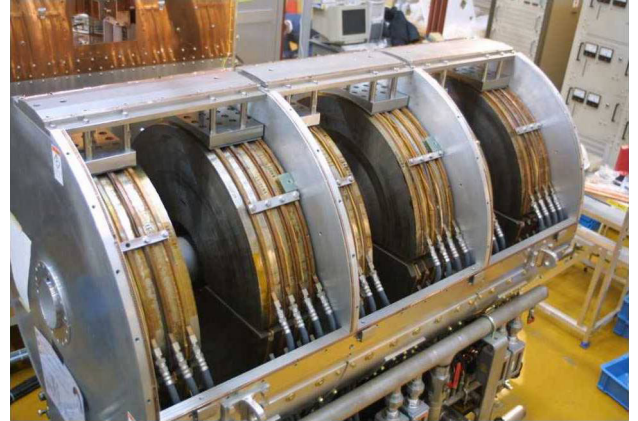
Fig.2 Assembly of a direct cooling cavity
