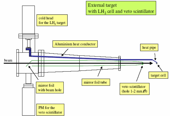
Fig.1 Schematic drawing of the LH 2 target instillation in WASA at COSY. Only the inlet for the heat conductor from the cold head has to be added to WASA.
