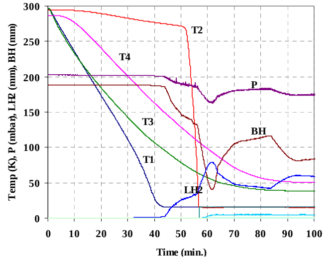
Fig. 2 Cool down time of the gold coated heat pipe and target with liquid hydrogen (without heat shield)
