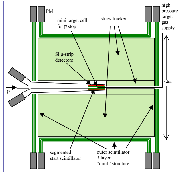
Fig. 2: Sketch of the detection set-up with two scintillator layers, the first one close to the target and the second one at a distance of about 1 m, in between tracking detectors are installed.
