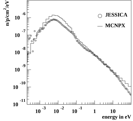
Fig. 2: Energy spectrum of an ice moderator at T=20 K measured without Pb-collimator, but with two additionally Cd-apertures in the neutron flight path.
