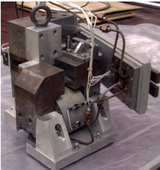
Fig. 4: Internal steering magnets at the exit of the cyclotron. The water leak had been caused by erosion of the copper tubes between the connectors and the encapsulated coil of the magnet.
