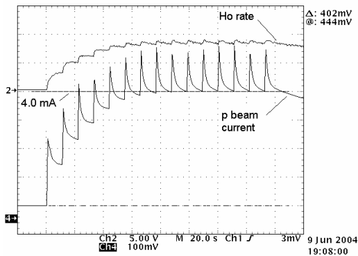
Fig. 2: Stacking by 15 repeated injections every 10 s. Equilibrium at 4.0 mA after 60 s.
