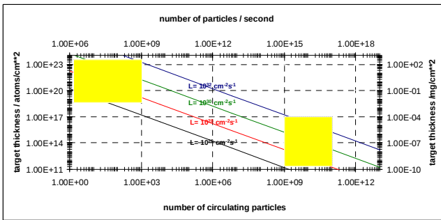
Fig. 1: Peak luminosity for internal and external experiments for typical target thicknesses at COSY. The internal luminosity is calculated for a particle revolution frequency of 1MHz in COSY (right yellow area), the external luminosity with an extraction time of 100s (left yellow area).
