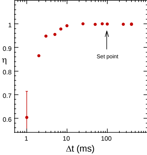
Fig. 3: The measured spin flip efficiency at 2.1 GeV/c is plotted against the rf-dipole ramp time \Delta t . The rf-dipole's frequency half-range \Delta f/2 was 6 kHz, and its \int B_{rms} dl was 0.46 Tmm.
