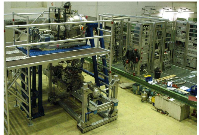
Fig. 2: The experimental setup in the "LKW-Schleuse" of the COSY hall: The ABS (vertical) in its horizontal support bridge, the LSP (horizontal) in the lower support system, and the ISTC chamber underneath the ABS. On the right-hand side the moveable platform (green) with the equipment for ABS and LSP is shown.
