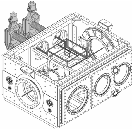
Fig. 1: Target chamber with XY-table and the frame supporting the apertures.
