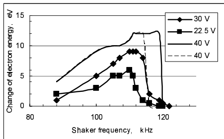
Fig. 2: Shape of the resonant peak between 90 and 120 kHz as function of the shaker voltage amplitude.
