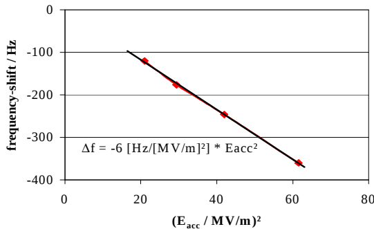
Fig. 2: Determination of the LFD-constant.
