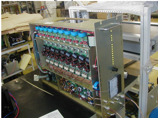
Fig.8 transistor driver 1kW designed by CERN / made in Japan.
