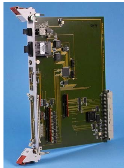
Fig. 3: Master control module with HOTLink interface
