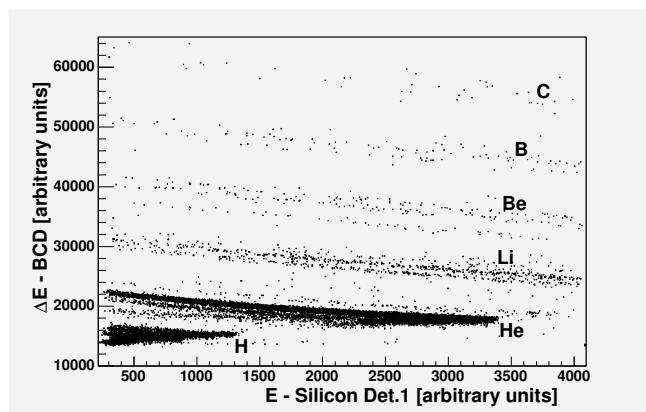
Fig. 1: \Delta E -E distributions where \Delta E is the energy deposited in the volume of Bragg Curve Detector while E is deposit of energy in the silicon detector placed behind.
