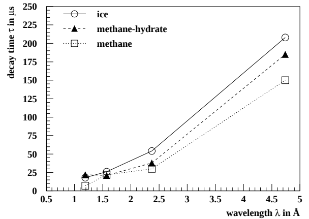
Fig. 3: Comparison of the decay time in μs for methane, ice, and methane-hydrate.
