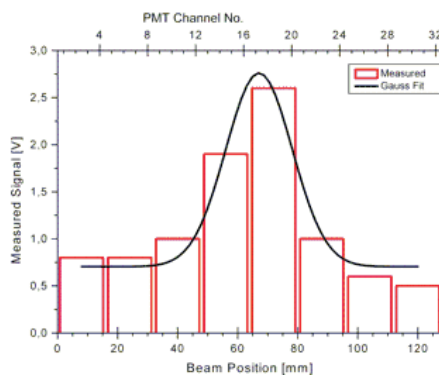
Fig. 2: Gauss fit of detected beam profile. For this experiment the 7 th and 8 th groups (right in picture) were darkened for visible light.
