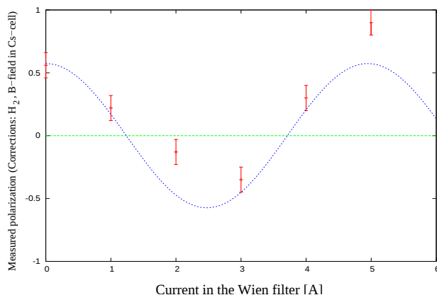
Fig. 1: The measured polarization along the beam line, when the quantization axis is rotated on the vertical magnetic field in the spinfilter.
