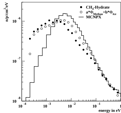
Fig. 3: Comparison of simulated and measured spectra of methane-hydrate. Additionally a synthetical methane-hydrate spectrum based on Eq. 1.
