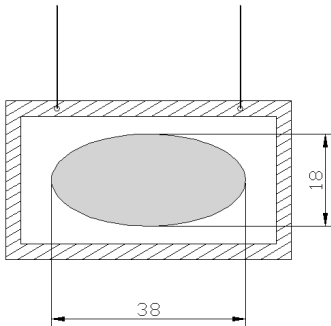
Fig. 2: COSY beam shape and dimensions at injection.
