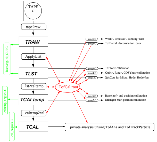
Fig. 1: Schematic view of the TofRoot data-flow. Four successive data formats are used from which standardized routines (automatically) evaluate calibration parameters.
