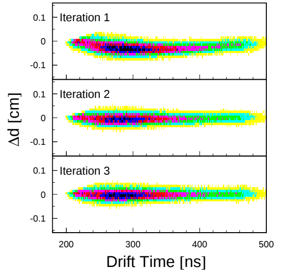
Fig. 3: Differences of the measured and fitted distances calculated as a function of the drift time for the first detection plane and the angular bin \theta \in (50^\circ, 60^\circ) in three subsequent iterations of the calibration procedure.
