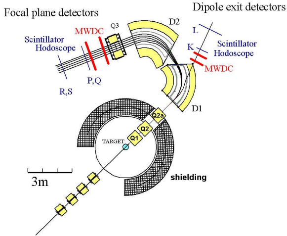
Fig. 1: BIG KARL with its detector systems for the focal plane and for the auxiliary detection plane behind dipole 1
