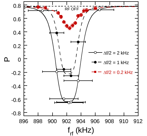
Fig. 2: The measured protons final-to-initial vector polarization ratio at 2.1 GeV/c is plotted against each ramp's frequency range \Delta f shown by a horizontal bar.
