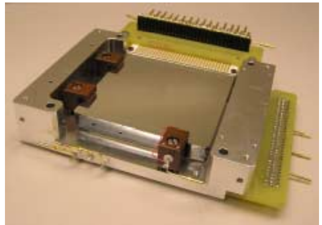
Fig. 1: The Si(Li) detector (9.7 mm thick) mounted in the LLNL holder. The testboards will be replaced by ceramic PCBs (printed circuit boards) at LLNL.
