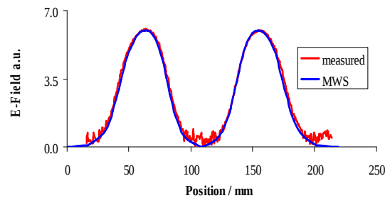
Fig.2: Comparison of measured and calculated field-profiles.
