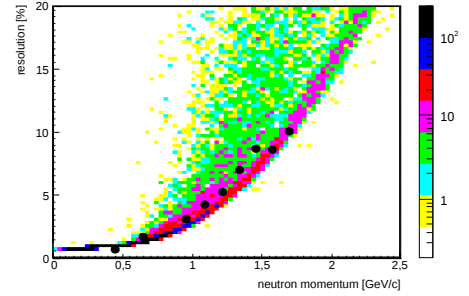
Fig. 2: Momentum resolution for the COSY – 11 neutron detector. The black filled circles are from MC studies and entries of the coloured distribution are the expected errors of the individual neutron detector signals interpreted as a neutron.
