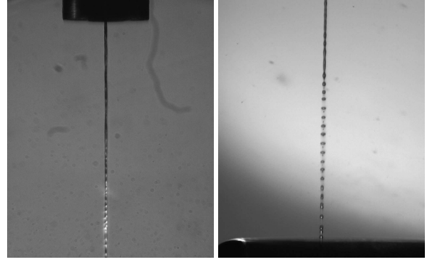
Fig. 2: Injection of an \text{H}_2 jet through a steel nozzle with l = 38 \mu\text{m} into the TPC (left). Breakup of a jet into droplets before the sluice to the first vacuum chamber (right).
