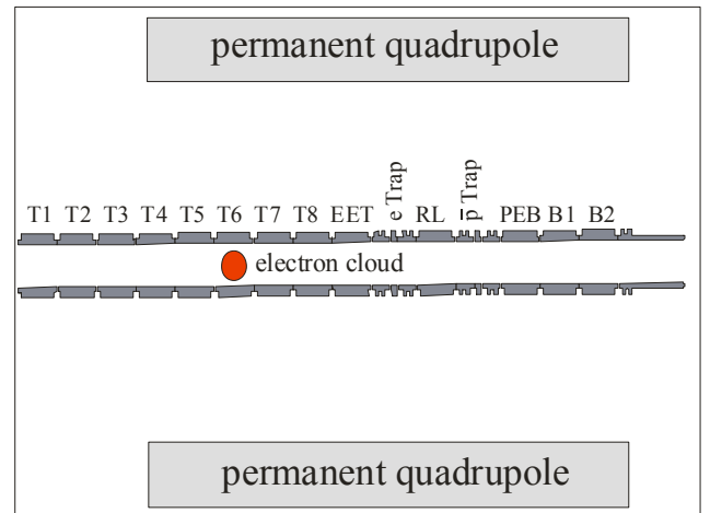
Fig. 2: Electrode structure of the lower trap part with the surrounding quadrupole and the electron cloud trapped at T6.
