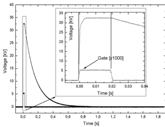
Fig. 3: Voltage pulse shape recorded at the septum test stand before installation at the cyclotron.
