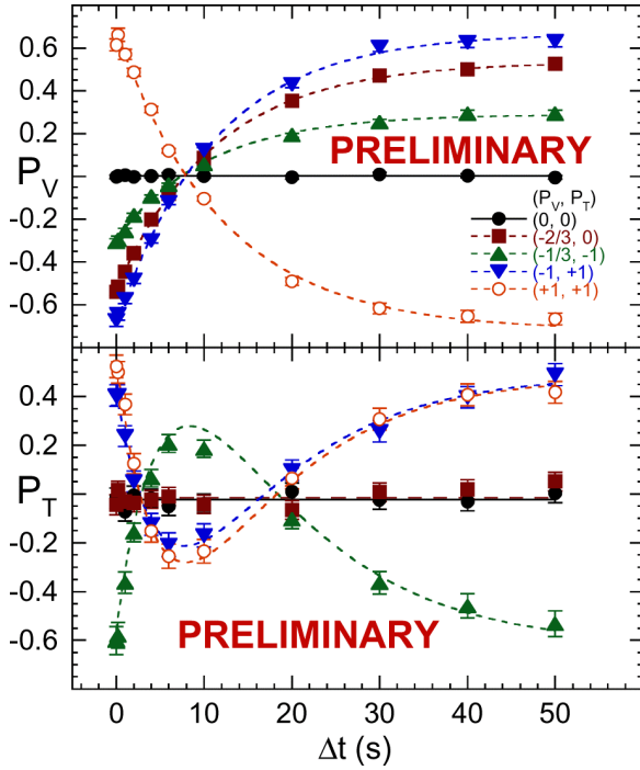
Fig. 5: The measured vector and tensor polarizations for the 5 deuteron spin states at 1.85 GeV/c is plotted vs. the rf-dipole's ramp time \Delta t , with \Delta f/2 = 100 Hz. The curves are fits using Eq. (2).
