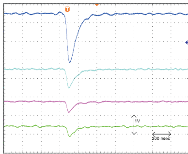
Fig. 1: Oscillogram picture of light signals registered at pressure of N_2 of 16 mbar, number of particles 5 \cdot 10^9 , energy 1.3 GeV. Bunch length \approx 100 nsec.
