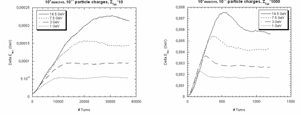
Fig. 2: r.m.s. value of \Delta E for different longitudinal impedances and energies
