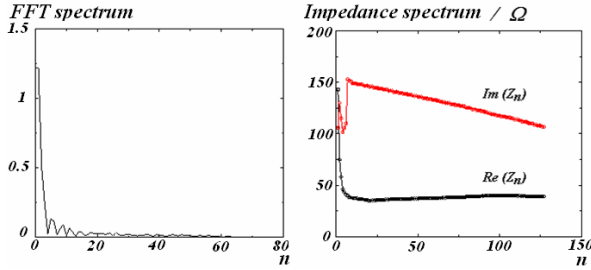
Fig. 1: Longitudinal FFT spectrum of the beam (left) and longitudinal impedance table (right)
