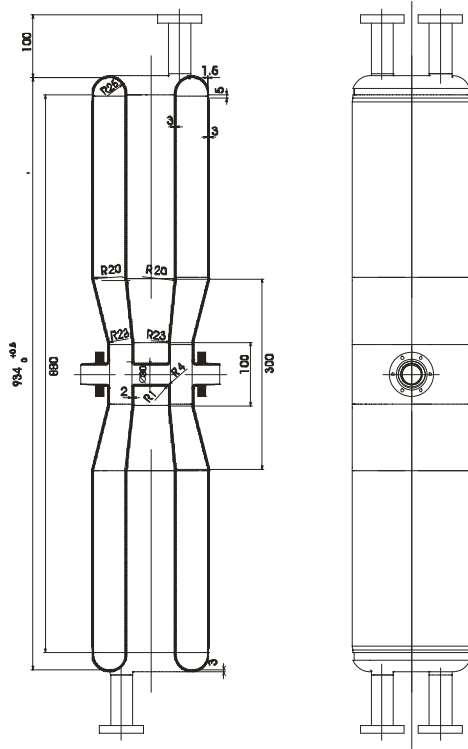
Fig. 1: Layout of the prototype cavity with round shaped top and bottom plate.
