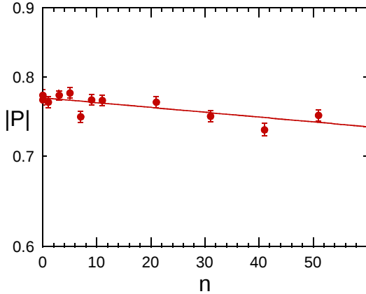
Fig. 4: The measured proton polarization at 2.1 GeV/c is plotted against the number of spin-flips. The rf-dipole's frequency ramp time \Delta t was 0.1 s; its frequency half-range \Delta f/2 was 6 kHz, and its \int B_{rms} dl was 0.34 Tmm.
