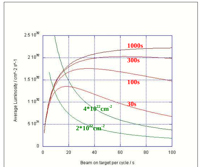
Fig. 2: Average luminosity for internal experiments with a pellet target thickness of 2.5 \cdot 10^{15} cm -2 (red lines), and external experiments with liquid target
