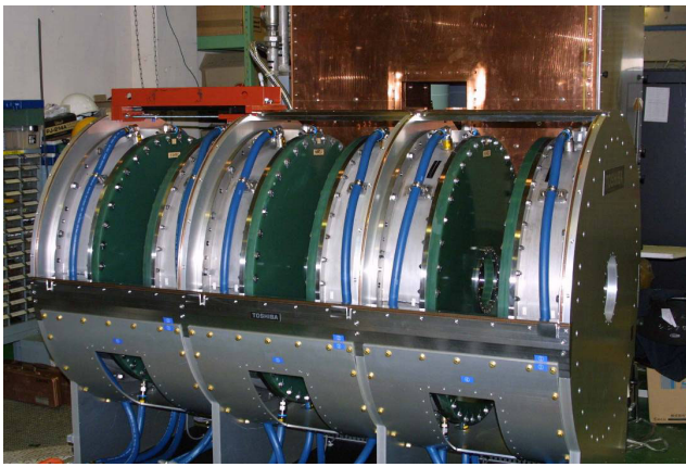
Fig.5 six tanks (3 gaps) assembled for direct cooling cavity
