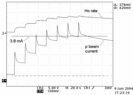
Fig. 1: Stacking of the proton beam intensity by 7 repeated injections every 20 s. Equilibrium is reached at 3.8 mA after 120 s. The time dependence of the neutral particles rate ( H^0 rate) indicates that the proton beam is fully cooled in less than 10 s. Applied electron beam current 170 mA (1 inch beam diameter). Tunes: Q_h = 3.61 , Q_v = 3.66 .
