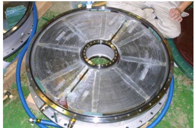
Fig.4 one tank of direct cooling cavity after assembly
