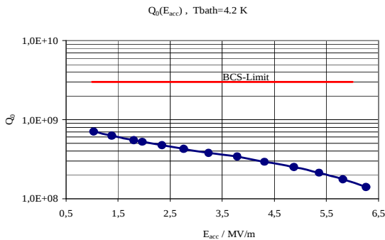
Fig.1: Q_0 - E_{acc} measurements of the HWR prototypes
