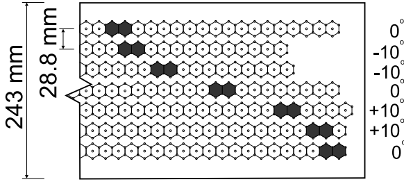
Fig. 1: Upper end-plate with indicated positions of openings for feedthrough used for mounting the wires. The shaded cells indicate the response of the chamber when one particle was registered
