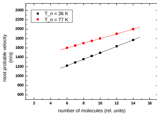
Figure 2. Most probable velocity of atomic hydrogen beam vs. number of molecules per pulse for nozzle temperatures of 36 K and 77 K.
