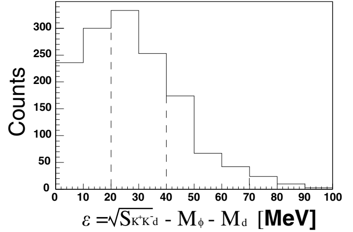
Fig. 2: The excess energy spectrum of the reaction pn \rightarrow d\phi . \sqrt{s_{K^+K^-d}} is the c.m. energy. M_\phi and M_d is the mass of the \phi -meson and the deuteron, respectively. Dashed lines separate three different excess energy regions shown in Fig.3 (a).
