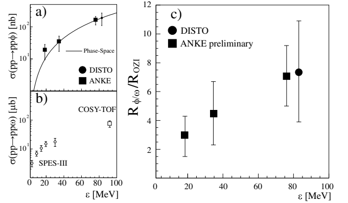
Fig. 2: (a) and (b) show the total cross section for the \phi and \omega production in pp collisions, respectively. In (c) the \phi to \omega cross section ratios normalized by R_{OZI} are shown.
