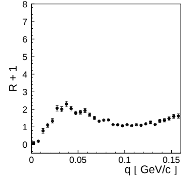
Fig. 2: The experimental two protons correlation function calculated from data [1] for the pp \rightarrow ppX reaction.
