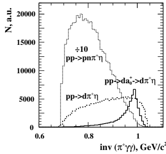
Fig. 1: Invariant mass ( \pi^+\eta ) for a_0^+(980) production in pp \rightarrow da_0^+ \rightarrow d\pi^+\eta and two background processes: direct production pp \rightarrow d\pi^+\eta and pp \rightarrow pn\pi^+\eta (divided by a factor 10).
