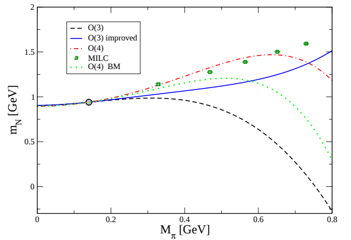
Fig. 1: Pion mass dependence of the nucleon mass. The dashed line gives the parameter-free third order result, the solid line the one with the improvement term as discussed in the text. Complete fourth order results are displayed by the dot-dashed and dotted lines for the optimal set of the LECs d_i and the values from [3], respectively. The filled circle shows the physical nucleon mass for the physical value of M_\pi . The data are from MILC [5].
