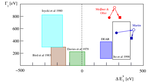
Fig. 1: Predictions of the ground-state strong shift \Delta E_1^s and width \Gamma_1 . Filled circles correspond to using the Deser formula (1), empty circles to using \mathcal{T}_{KN}^{(0)} instead of (a_0 + a_1)/2 in this formula, and filled boxes to our final formula (2) with \delta\mathcal{T}_{KN} = \delta_n^{\text{vac}} = 0
