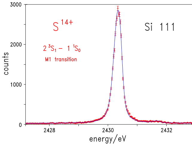
Fig. 1: The spectrum of the M1 transition from helium-like sulfur measured with a Si 111 crystal is shown together with a best fit.
