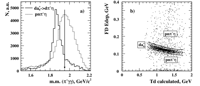
Fig. 2: (a) Reconstructed missing mass ( \pi^+\gamma\gamma ) for pp \rightarrow da_0^+ \rightarrow d\pi^+\eta and pp \rightarrow pn\pi^+\eta . The cut is indicated by the arrow. (b) Energy losses in FD vs. kinetic energy of deuterons calculated from the measured pion and two photons. The cuts are indicated by curves.
