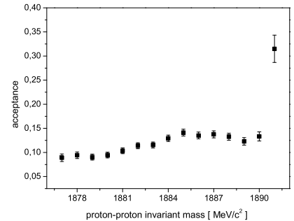
Fig. 2: Ratio of the spectra from figure 1. (see text)
