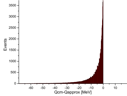
Fig. 1: Distribution of the difference between the real and approximated excess energy of the quasi-free pn \rightarrow pn\eta reaction simulated for the pd \rightarrow pn\eta p_{sp} process at the proton beam momentum of 2.075 GeV/c. For details see text.
