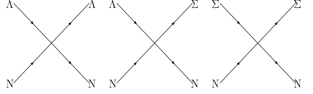
Fig. 1: Lowest order contact hyperon-nucleon interactions
