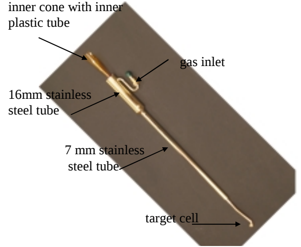
Fig. 1: Gold coated heat pipe and target appendix.
