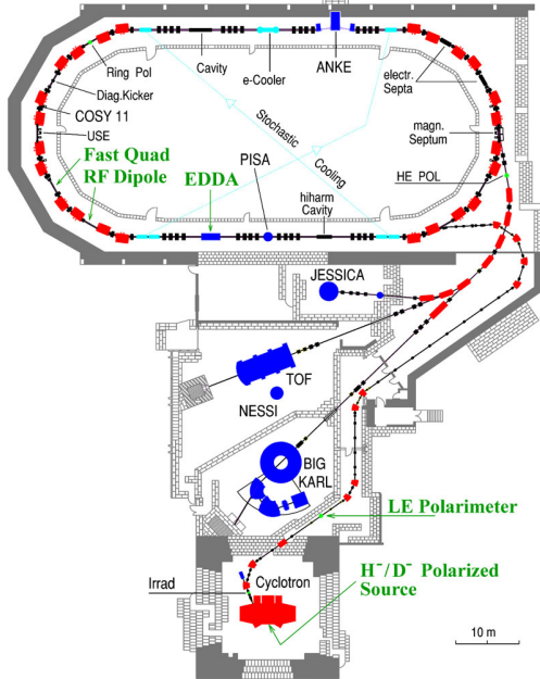
Fig. 1: Layout of the Cooler Synchrotron Storage Ring COSY, with its injector Cyclotron JULIC and polarized ion source. Also shown are, the rf dipole, the EDDA detector and the Low Energy Polarimeter.
