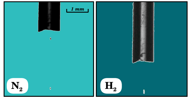
Fig. 3: \text{N}_2 and \text{H}_2 frozen pellets with l \sim 30 \mu\text{m} ( l_{\text{nozzle}} = 18 \mu\text{m} ) behind the sluice to the vacuum chamber.
