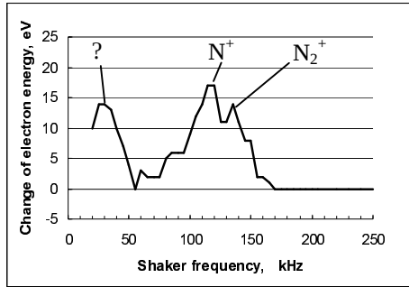
Fig.1: Spectrum of shaker frequencies. Electron beam current 170 mA (1 inch beam diameter), magnetic field in the cooling section 0.08 T, \beta = 0.299 .
