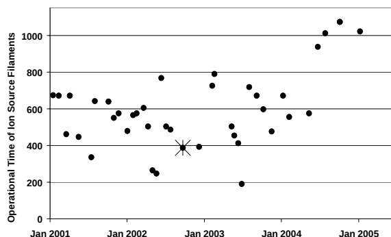
Fig. 2: Up-time of the filament driven ion sources since beginning of 2001. The asterisk marks the single failure of a filament during this period.
