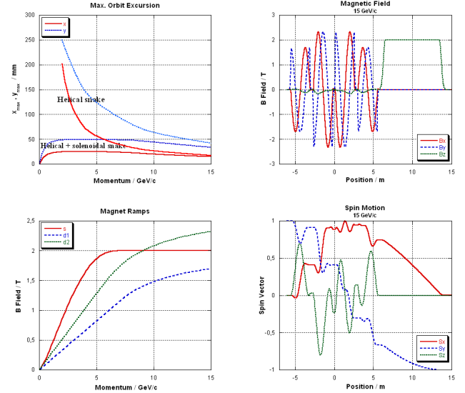
Fig. 1: Calculations for the layout of a full Siberian snake with combined magnetic fields
