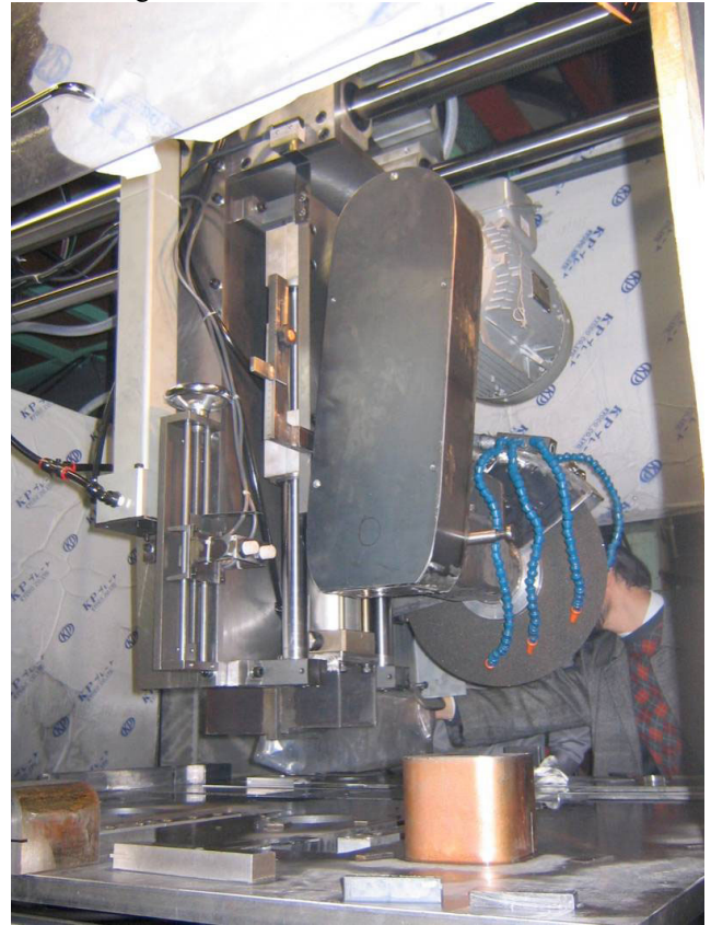
Fig.7 the grindstone cutting machine
