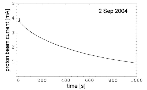
Fig. 3: Approximately exponential decay of the stacked proton beam intensity after the last injection. Electron current 170 mA. Q_h = 3.620 , Q_v = 3.645 .
