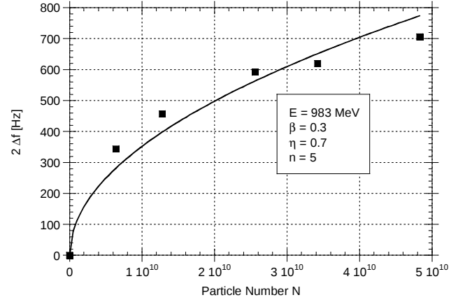
Fig. 2: Peak distance versus number of stored protons. The curve is a fit to the data according to eq. (2) assuming a pure capacitive impedance.
