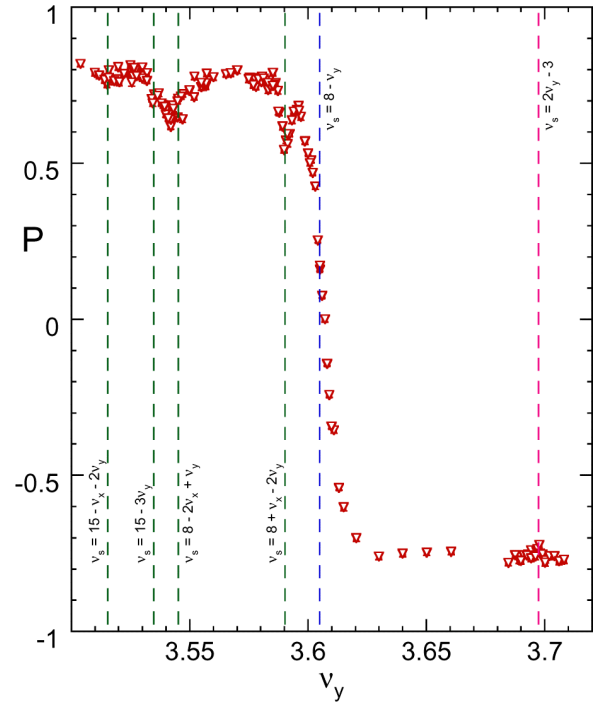
Fig. 6: The preliminary results for measured protons vector polarization 2.1 GeV/c is plotted against the vertical betatron tune of COSY. A total spin flip at the strong resonance at a tune of about 3.605 is clearly visible.
