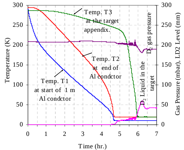
Fig. 2 Temperatures during cooling down of cold head, 1 meter aluminium heat conductor and target cell at the end of the 7 mm diameter heat pipe with deuterium filling.
