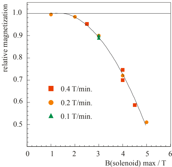
Fig. 1: Reduction of the magnetization in the permanent magnet normalized to the initial value for various field strengths of the outer solenoid field.
