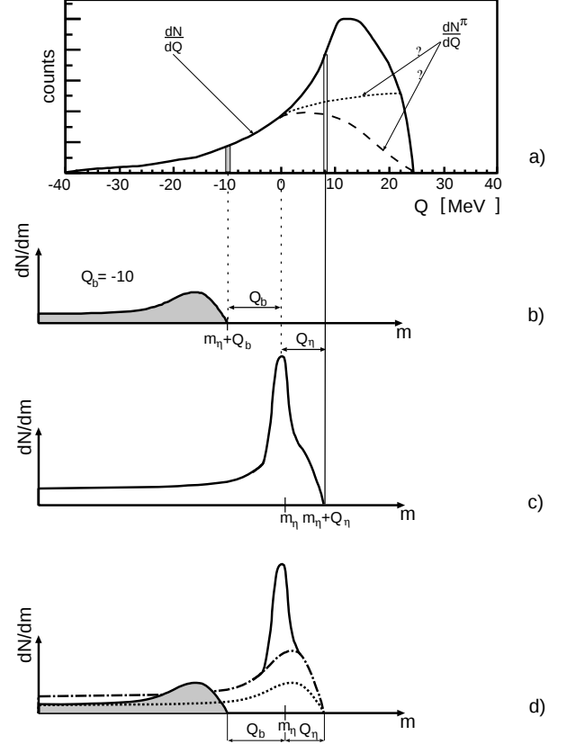
Fig. 1: a) Distribution of the excess energy with respect to the pn \rightarrow pn\eta reaction plotted schematically for the beam momentum of P_b = 2.075 \text{ GeV}/c [2]. b), c) Scheme of the missing mass spectra as derived for the negative ( Q_b ) and positive ( Q_{\eta} ) values of Q. d) The shape of the background in the mass spectrum for Q larger than zero can be constructed from the shape of the multi-pion mass distribution determined for Q less than zero.
