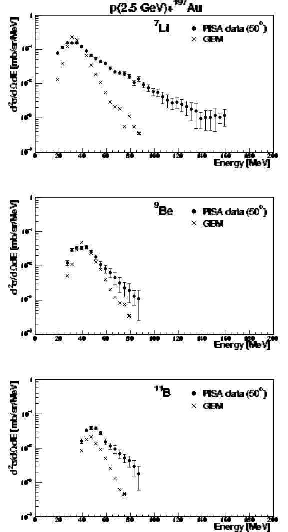
Fig. 2: Comparison between energy spectra of ^7\text{Li} , ^9\text{Be} and ^{11}\text{B} measured at 50° by PISA collaboration (full dots) and INCL4.2+GEM model calculations (crosses).
