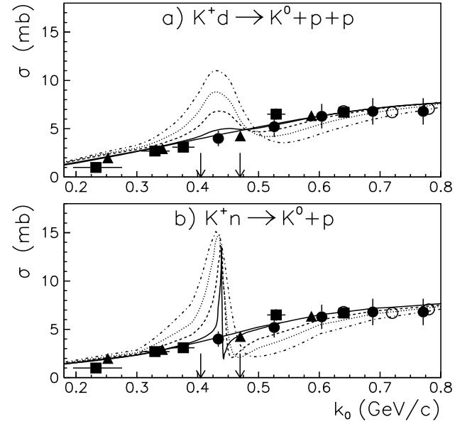
Fig. 1: Total K^+d \rightarrow K^0pp cross section as a function of the kaon momentum. The curves in a) show our full results for the original Jülich KN model without the \Theta^+ resonance (solid line) and the variants with a \Theta^+ and with different widths ( \Gamma_\Theta=1 MeV - solid with bump; 5 MeV - dashed; 10 MeV - dotted; and 20 MeV - dash-dotted). The curves in b) correspond to a calculation for the reaction K^+n \rightarrow K^0p assuming that the neutron target is at rest. The vertical arrows indicate the range of kaon momenta corresponding to the smallest and the largest values found experimentally for the mass of the \Theta^+ resonance.
