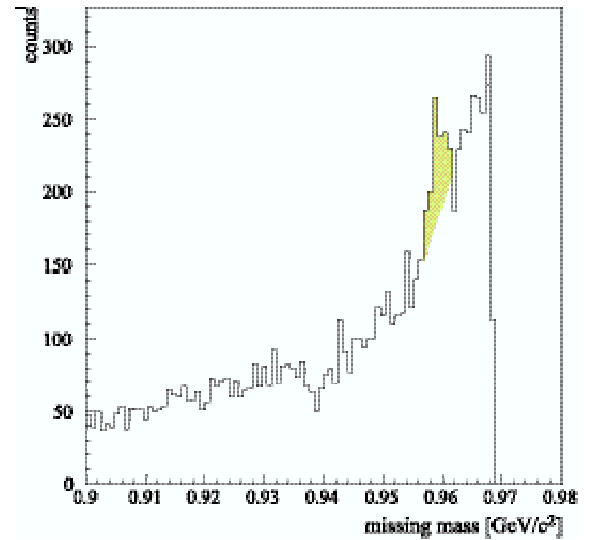
Fig. 3: Missing mass spectrum of the reaction pd \rightarrow {}^3\text{He} X , obtained at an excess energy of Q = 10 MeV and integrated over a range of cms scattering angles of -0.6 \leq \cos\Theta^* \leq 0.6 .
