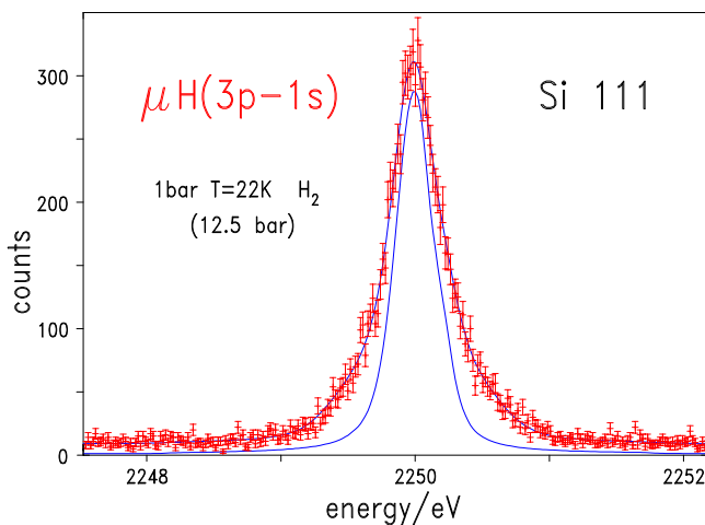
Fig. 1: The spectrum of K\beta transition in muonic hydrogen measured with a Si111 crystal is shown together with a best fit and the corresponding resolution function.
