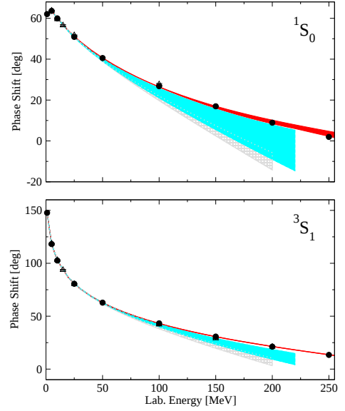
Fig. 1: S-waves at NLO (grey bands), at NNLO (blue bands) and at N^3LO (red bands). Circles (triangles): Nijmegen (VPI) PWA.
