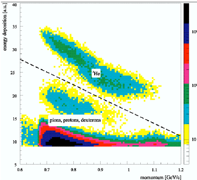
Fig. 1: Identification of {}^3\text{He} nuclei using both the reconstructed momentum and the energy loss in a scintillator hodoscope. The possibility for a clean separation from other particles is indicated by the dashes line.
