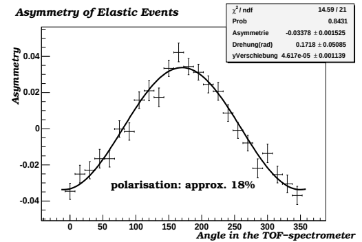
Fig. 2: The asymmetry of elastically scattered events ( \Rightarrow polarization) is evaluated with the same function, online as well as offline.
