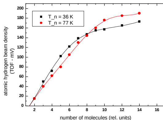
Figure 1. Atomic hydrogen beam density vs. gas flux into the dissociator in number of molecules per pulse.
