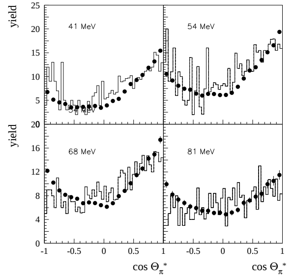
Fig. 2: \pi^- angular distributions of the reaction np \rightarrow pp\pi^- in comparison with data taken from [1].
