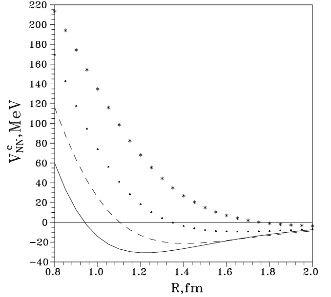
Fig. 1: Spin-isospin-independent central part of the residual NN potential in ^{40}\text{Ca} . The solid line corresponds to the free NN potential, whereas the dashed line, dotted line and stars refer to a radially aligned NN-system that is located at a distance D = 4 fm, 3 fm and 0 fm, respectively, from the center of the nucleus.
