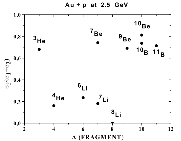
Fig. 2: Contribution of the preequilibrium mechanism to the emission of composite fragments from Au+p collisions at 2.5 GeV proton beam energy.
