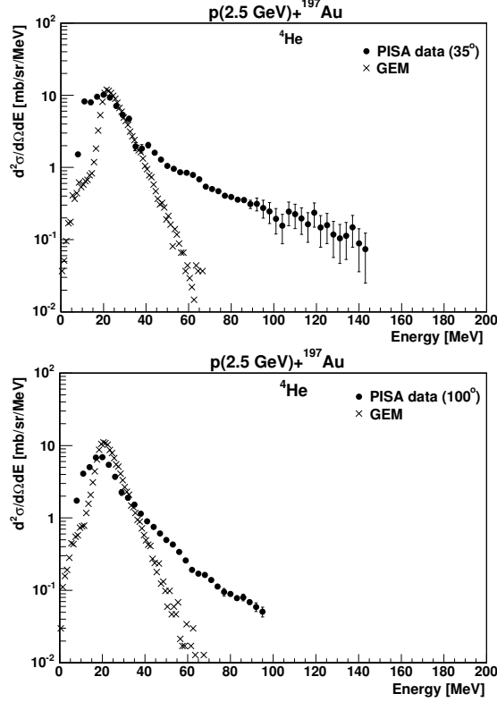
Fig. 1: Comparison between energy spectra of ^4\text{He} measured at 35° and 100° by PISA (full dots) and INCL4.2+GEM model calculations (crosses).
