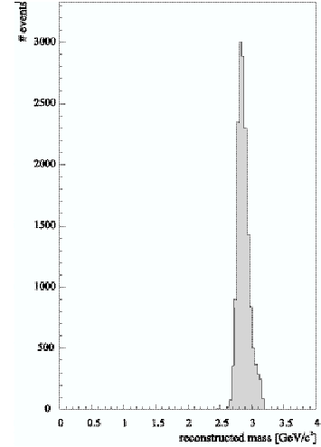
Fig. 2: Reconstructed mass of the detected {}^3\text{He} nuclei. The picture presents the selected events at Q = 10 MeV.
