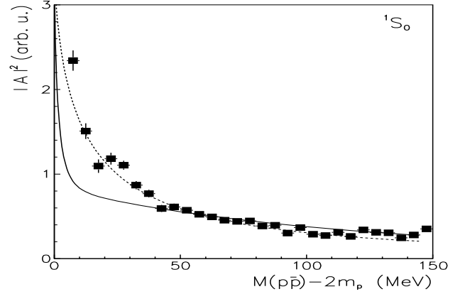
Fig. 1: Invariant J/\Psi \rightarrow \gamma p\bar{p} amplitude |A|^2 as a function of the p\bar{p} mass. The squares represent the experimental values of |A|^2 extracted from the BES data[1] via Eq.(3). The curves are the scattering amplitude squared ( |T|^2 ) predicted by the N\bar{N} model A(OBE) [4] for the ^1S_0 partial waves and the I=0 (solid) and I=1 (dashed) channels, respectively.
