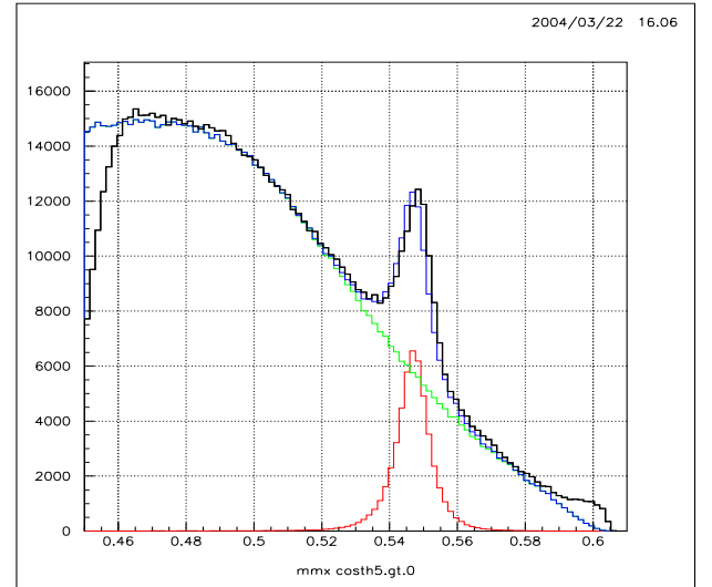
Fig. 2: Missing mass distribution [ \text{GeV}/c^2 ]. Only events of the forward cm angles of the \eta are shown. The black curve shows the measured data, the green curve the simulated pion background, the red curve the simulated \eta events, to fit the measured curve. The blue curve is the sum of the simulated pion and \eta events. The deviation below m_x = 0.46 \text{ GeV}/c^2 is due to a cut in the data to enrich the \eta events.
