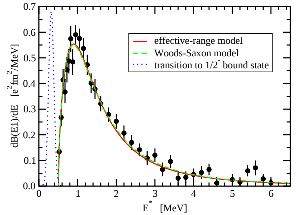
Fig. 1: Reduced transition probability as a function of the excitation energy E^* compared to experimental data extracted from the Coulomb breakup of ^{11}\text{Be} . For further explanation see [1]
