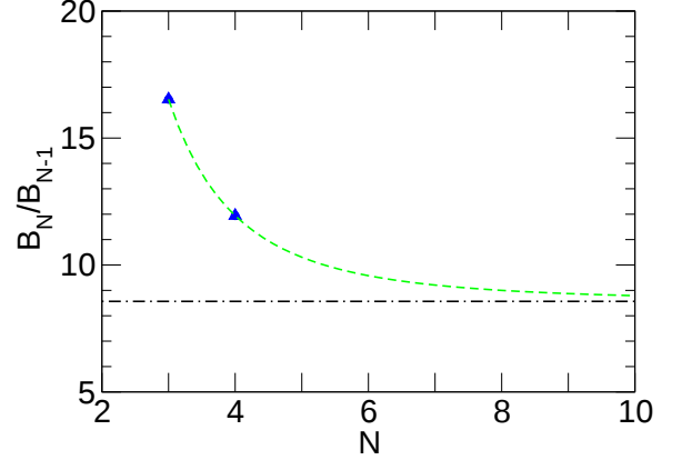
Fig. 1: B_N/B_{N-1} as a function of N . The dot-dashed line shows the asymptotic value of 8.567. The dashed line is an estimate of how the large- N value is approached.
