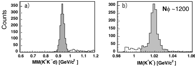
Fig. 1: a) Missing proton mass spectrum for the reaction pd \rightarrow dK^+K^-p_s . The shadowed region shows the cut for the missing proton. b) shows the K^+K^- invariant mass spectrum. The shadow region shows the \phi -meson cut.
