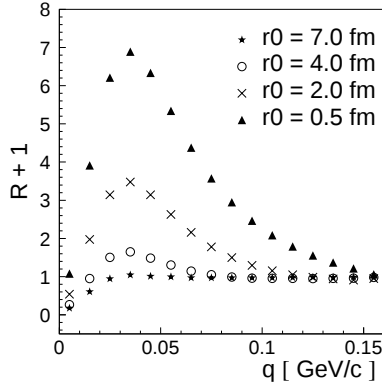
Fig. 1: Theoretical correlation functions of two protons for r_0 = 0.5, 2.0, 4.0 and 7.0 fm.
