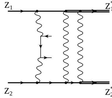
Fig. 1: One of the diagrams which describes mutual giant dipole resonance excitation and electron pair production
