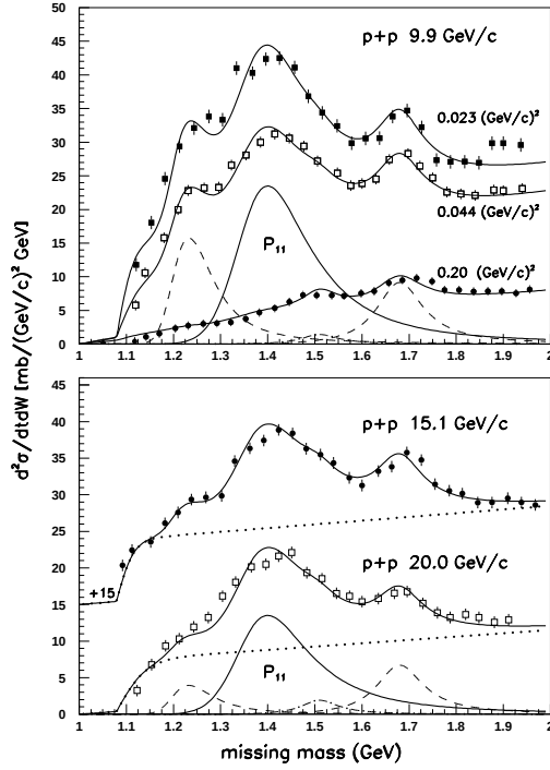
Fig. 1: Missing mass spectra of p + p \rightarrow p x at different beam momenta in comparison with our resonance fits. The resonance at 1400 MeV is the strongest N^* observed.
