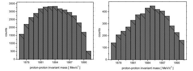
Fig. 1: Proton-proton invariant mass spectra. (left) generated, (right) reconstructed from signals in the detector. For the reconstruction only events with the invariant mass of the \gamma\gamma system larger than 800 MeV were taken into account.
