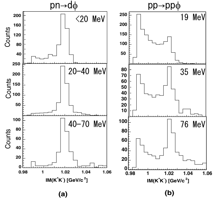
Fig. 3: (a) K^+K^- invariant mass spectra of the reaction pn \rightarrow d\phi at three excess energy regions. (b) K^+K^- invariant mass spectra of the reaction pp \rightarrow pp\phi at three fixed excess energies. The excess energies are indicated in the figures.
