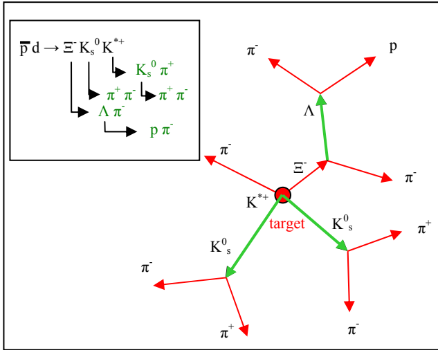
Fig. 1: Sketch of a suitable reaction channel to study the production of \Xi . The primary produced K^{*+} decays within a few fermi into a K_s^0 and a \pi^+ resulting in three delayed decays which allows to create a very clean trigger signal via multiplicity increase.
