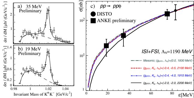
Fig. 1: (a) and (b) show the efficiency corrected K^+K^- invariant mass distribution at excess energies of 35 MeV and 19 MeV. The dashed curves are the non-resonant contributions based on four-body phase space. The solid line is the sum of non-resonant contribution and \phi -meson production including the detector resolution. In (c) the total \phi cross sections from ANKE are shown together with the DISTO point. The error bars indicate the systematical uncertainties. The lines are predictions from Ref. [5].
