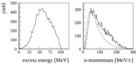
Fig. 1: left: range of excess energies extracted event-by-event from the data; right: Fermi momentum distribution of the bound neutron (histogram) in comparison with the one derived from an analytic parametrization of the deuteron wave function (Hulthen function).
