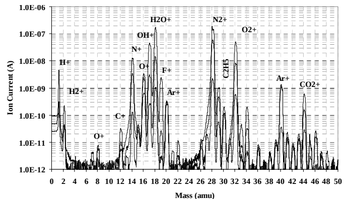
Fig. 2 The residual gases and all outgassing spectrum during fast heating and cleaning the full gas hydrogen target in the small TOF tank after 21 days from starting the vacuum system.
