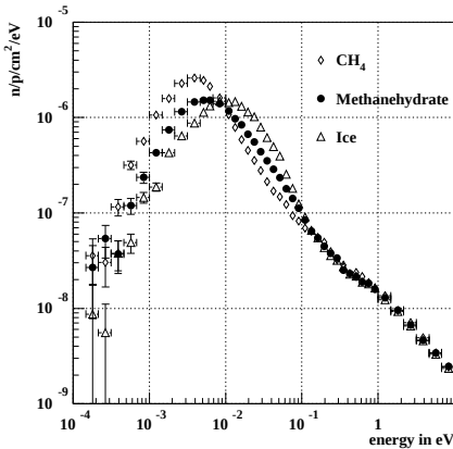
Fig. 2: MCNPX simulations of the energy spectra for ice, methane, and methane-hydrate.
