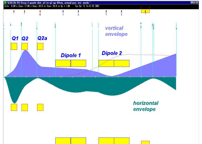
Fig. 3: Envelope structure in the spectrograph in the standard high-resolution mode
