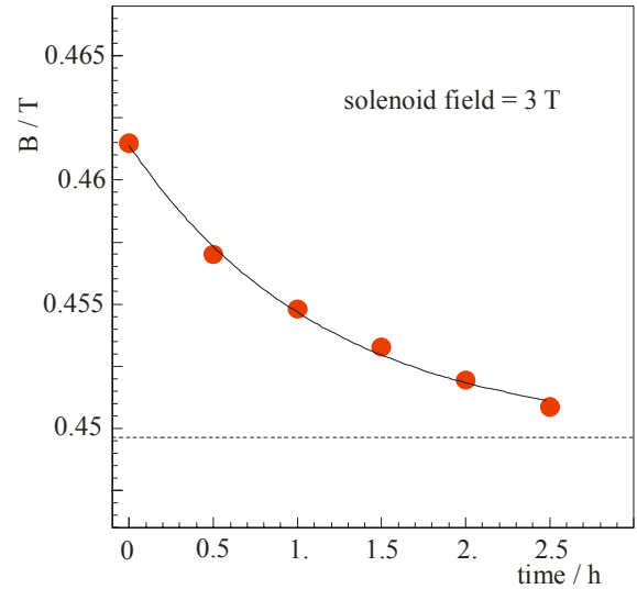
Fig. 2: Time dependence of the de-magnetisation of a test piece exposed to a solenoid field of 3T.
