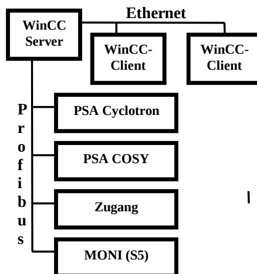
Figure 3: overview of the personal safety and radiation survey systems
