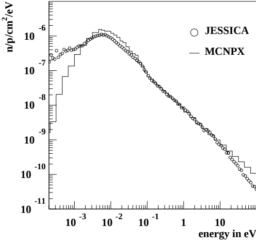
Fig. 1: Energy spectrum of an ice moderator at T=20 K measured without Pb-collimator and without additionally Cd-apertures in the neutron flight path.
