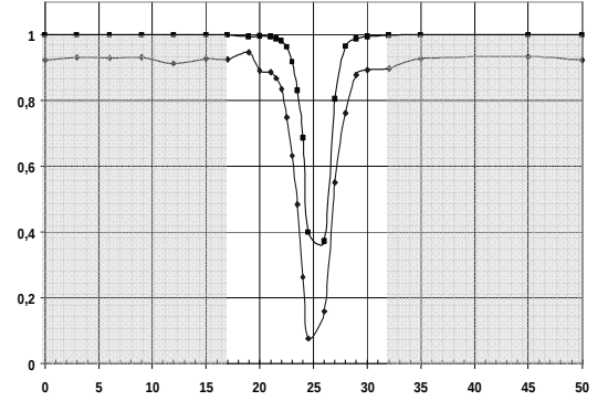
Fig. 3a: horizontal beam dimension scan.
