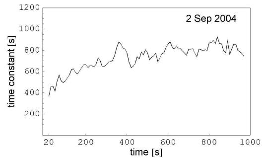
Fig. 4: Instantaneous time constant of the decay curve shown in Fig.3. The 1/e lifetime is shorter at higher proton intensities. The fluctuations are mainly caused by the numerical evaluation, Eq.(1).
