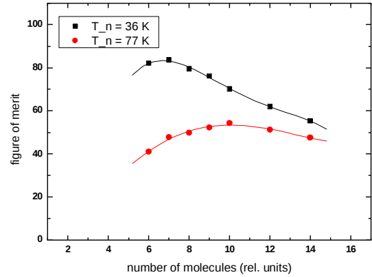
Figure 3. Figure of merit for atomic hydrogen beam for nozzle temperatures of 36 K and 77 K vs. number of molecules per pulse
