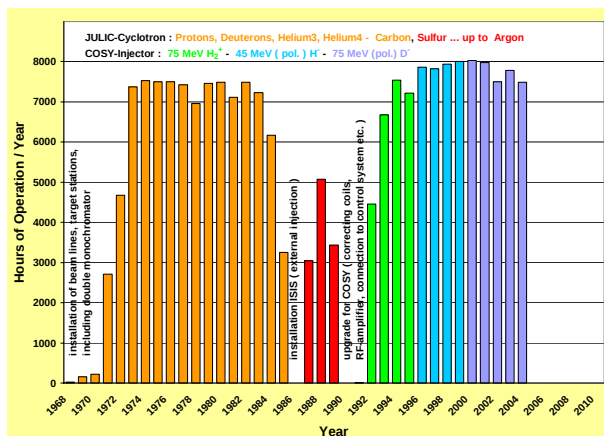
Fig. 1: Operation of the Cyclotron. At the end of 2004 the total operating time reached 206,148 hours.
