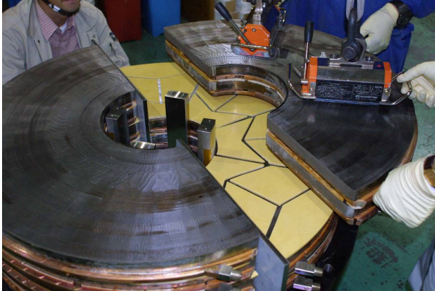
Fig.1 Stacking FineMet cores for the indirect cooled cavity
