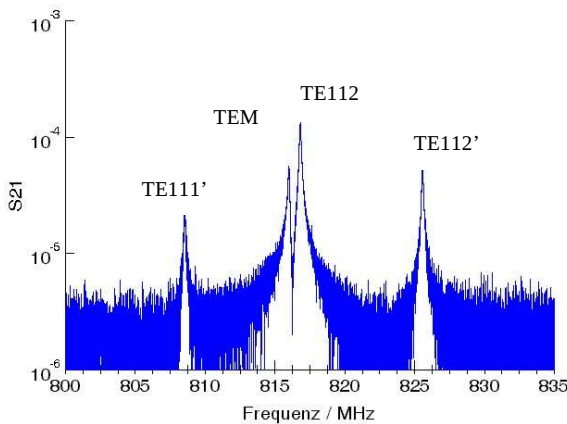
Fig. 2: 6 th -9 th Eigenmodes of the HWR-Prototype Type II.
