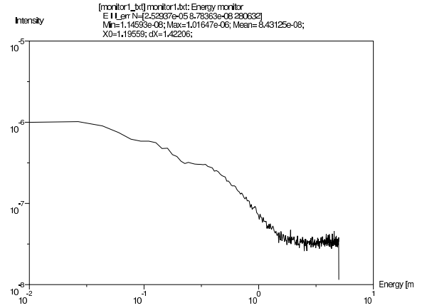
Fig. 3: Energy spectrum transported.
