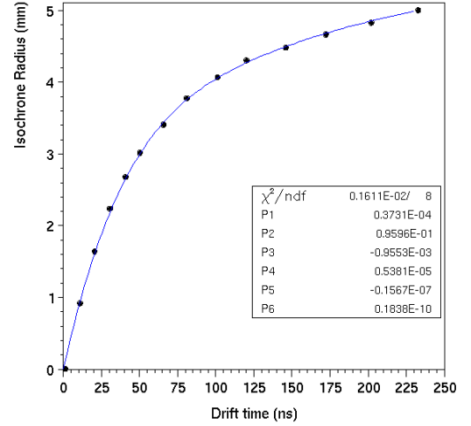
Fig. 1: Isochrones radius - drift time relation, parameterised using a polynomial of fifth order (parameters P 1 -P 6 ).
