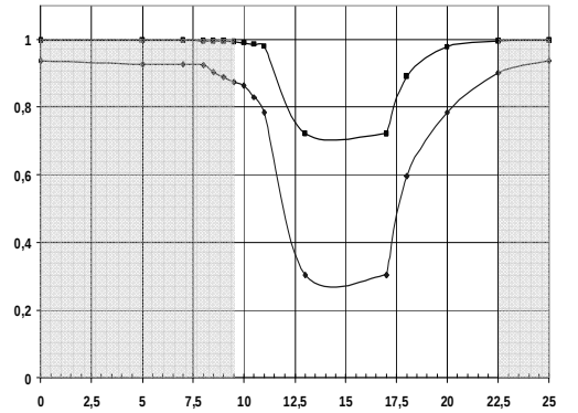
Fig. 3b: vertical beam dimension scan.
