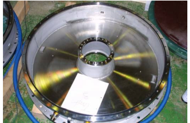
Fig.3 one tank of direct cooling cavity before assembly
