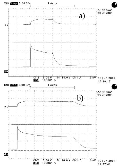
Fig. 3: Proton beam current (lower curve) and H^0 count rate (upper curve) versus time when no feedback is applied to stabilize the beam: a) Shaker off or nonresonant excitation, b) Excitation with the resonant frequency of 114 kHz. 100 mV/div correspond to 1 mA beam current
