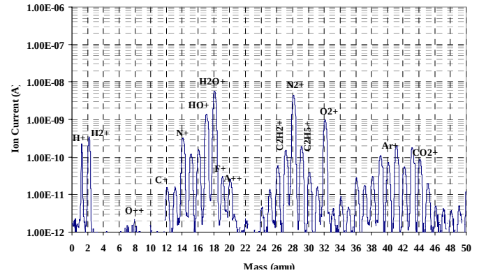
Fig. 1 The residual gases in the small TOF tank after 21 days from starting the vacuum system with full liquid hydrogen target.
