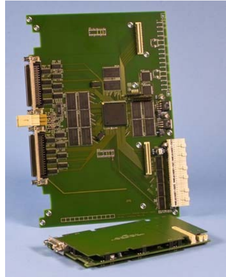
Fig. 2: LVDS-Sequencer with ADC piggy-pack
