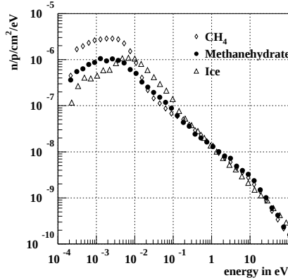
Fig. 1: Measured energy spectra for ice, methane, and methane-hydrate.
