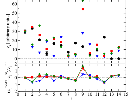
Fig. 1: Comparison of the extracted |z_i| (black circles) with corresponding predictions of the Jülich model [2]; the squares (inverted triangles) refer to model-results with inclusion (omission) of the \Delta isobar. For the diamonds only \Delta excitations before the pion emission are included. The upper panel shows the results for the various amplitudes, normalized to the s -wave and the lower panel shows the relative deviations from the extracted values.
