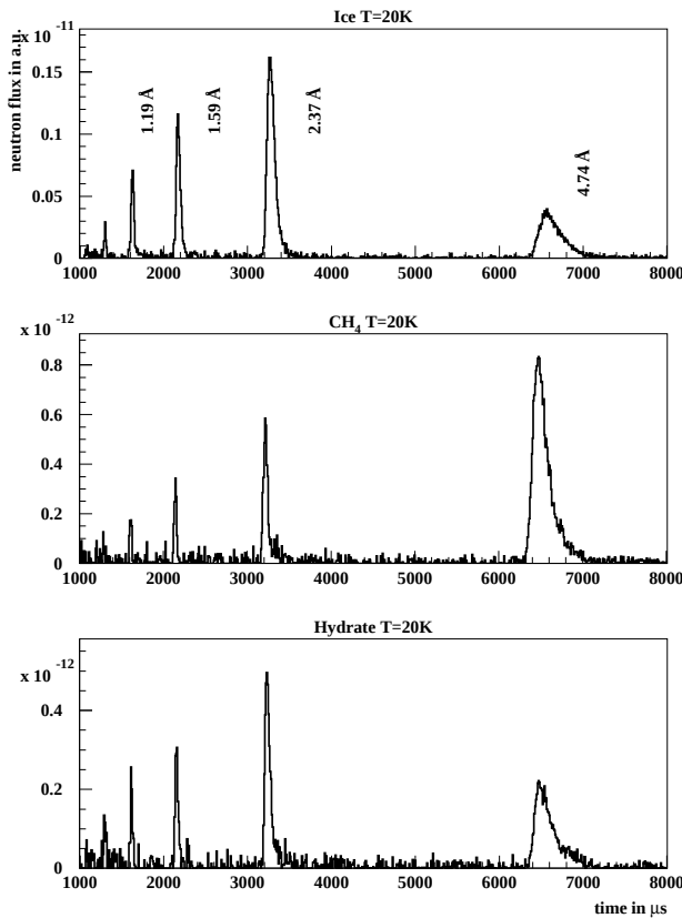
Fig. 1: Comparison of wavelength dependent TOF-spectra of ice, methane, and methane-hydrate at a temperatur of T=20 K.
