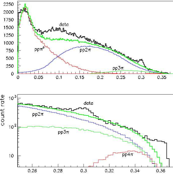
Fig. 1: Squared missing mass distribution [ \text{GeV}^2/c^4 ]. The upper figure shows the full range, in the lower figure the distribution in the missing mass range around the \eta is plotted in a logarithmic scale.
