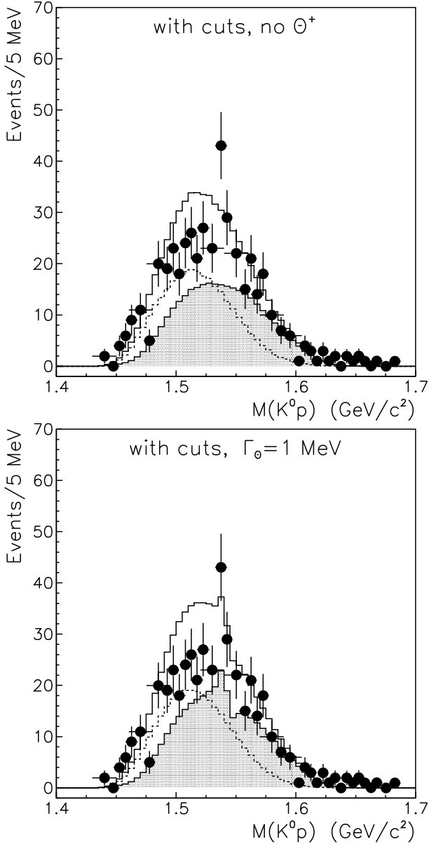
Fig. 1: The K^0 p invariant mass spectrum from the K^+ \text{Xe} reaction. The circles are the data (with cuts) from Ref. [2]. The hatched histograms show our results for the spectrum from direct K^+ n \rightarrow K^0 p production on a bound target neutron, while for the dashed curve an additional single rescattering of the proton was taken into account. The solid curve is their sum.
