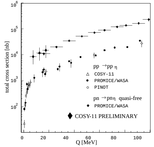
Fig. 2: Preliminary results of the total cross section for the \eta meson production in the quasi-free p - n scattering. Diamonds indicate COSY-11 preliminary results, and the other points show the data from [1, 5].
