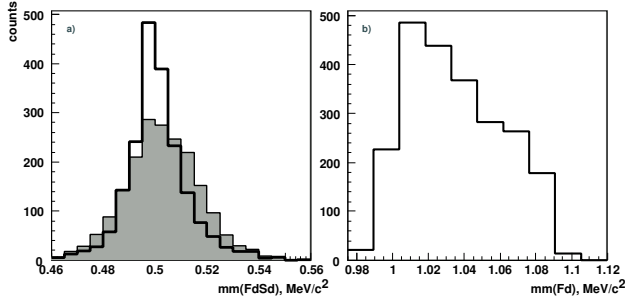
Fig. 1: a) dK^+ missing mass using two momentum reconstruction methods, polynomial (shaded histogram) and Runge-Kutta (solid line). b) Deuteron missing mass obtained with the Runge-Kutta algorithm.
