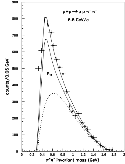
Fig. 2: Invariant \pi^+\pi^- mass spectrum from ref. [5] in comparison with a resonance fit consistent with Fig. 1. The multi-pion background is given by the dotted line.
