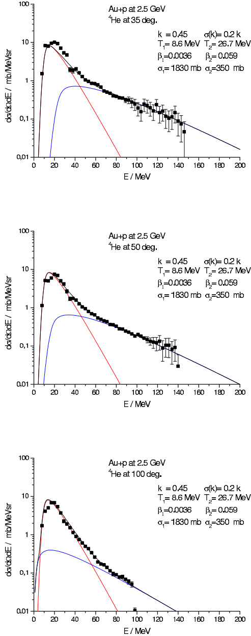
Fig. 1: Energy spectra of {}^4\text{He} fitted with the sum of two Maxwell functions. The red and blue curves represent the contributions of these two moving sources, and black solid line is their sum.
