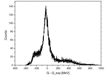
Fig. 3: Distribution of the difference between generated and reconstructed excess energy.
