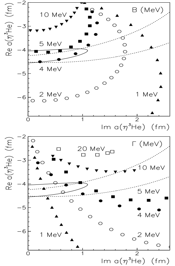
Fig. 1: The \eta^3\text{He} binding energy B (upper panel) and width \Gamma (lower panel) as functions of the imaginary and real parts of the \eta^3\text{He} scattering length. Results are presented for B and \Gamma of 1 MeV (triangles), 2 MeV (open circles), 4 MeV (close circles), 5 MeV (close squares), 10 MeV (inverse triangles) and 20 MeV (open squares). The solid and dashed contours show our \chi^2+1 solutions for the \eta^3\text{He} scattering length [1].
