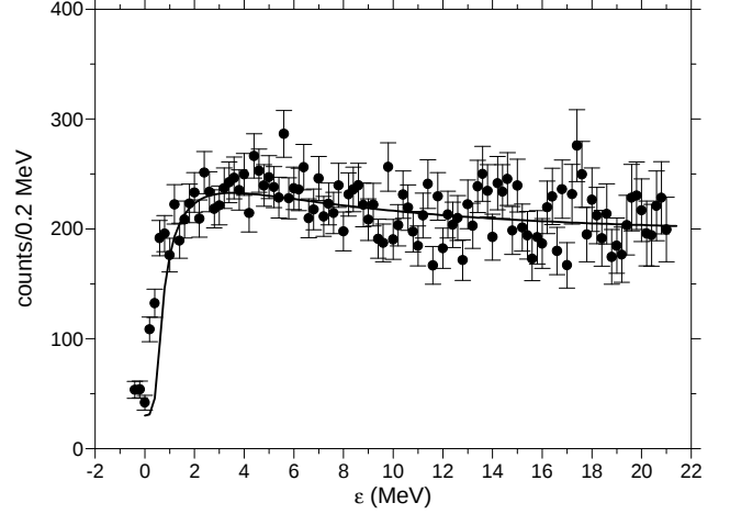
Fig. 1: Comparison of the data (histogram) with the fitted triplet plus singlet state.
