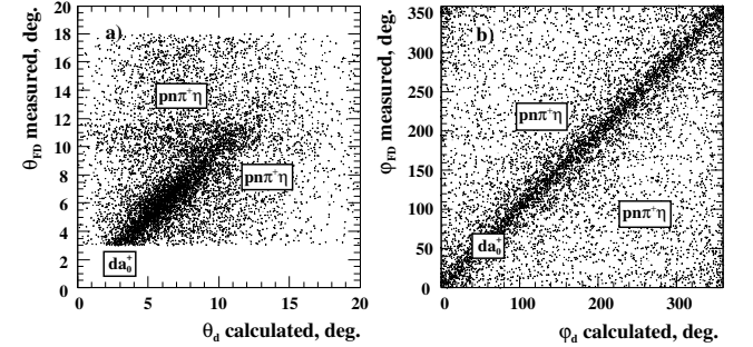
Fig. 3: (a,b) Measured forward angles vs. angles calculated for deuterons. The cuts are shown by lines.
