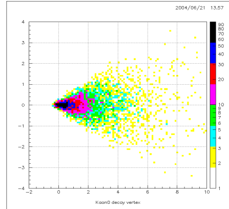
Fig. 1: Spatial distribution of the K^0 decay vertex (longitudinal versus transversal component) [cm]
