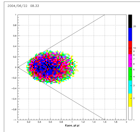
Fig. 2: K^0 longitudinal versus transversal momentum in GeV/c. The black lines indicate the limits due to the target window
