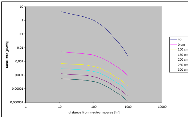
Figure 1: Dose rate in dependence of the distance r from the neutron source and different thicknesses d of the top shielding made from 100cm concrete plus the given numbers of earth-shielding in cm. The dark blue line (no) shows the dose rate without any shielding.
