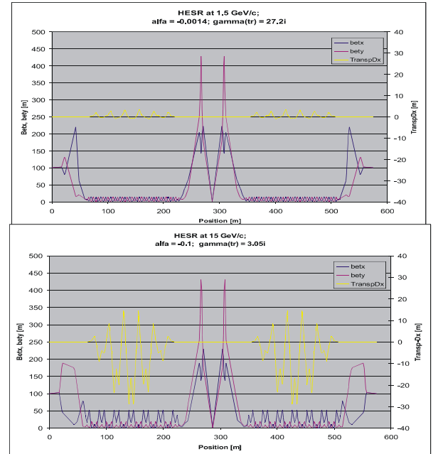
Fig. 43: \beta -functions and dispersion function for a low energy (upper) and a high energy (lower) HESR lattice. The target is located at 287 m. The HESR will operate with an imaginary gamma-transition value over the entire momentum range.
