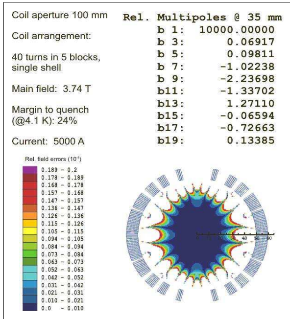
Fig. 44: Coil arrangement and calculated 2D-field quality for the superconducting HESR dipole magnets designed as a shortened version of the original RHIC-D0 magnet.
