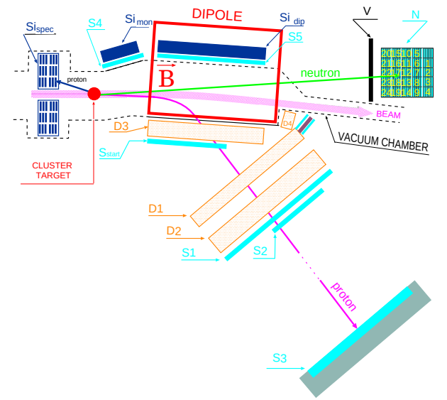
Fig. 2: Schematic view of the COSY-11 setup.
