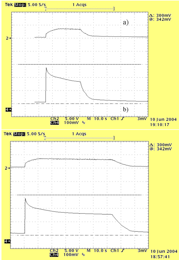
Fig. 37: Proton beam current (lower curves) and H^0 count rate (upper curves) versus time: a) Shaker is off or non-resonant excitation, One division corresponds to 1 mA beam current. b) Excitation with resonant frequency of 114 kHz.. One division corresponds to 1 mA beam current.
