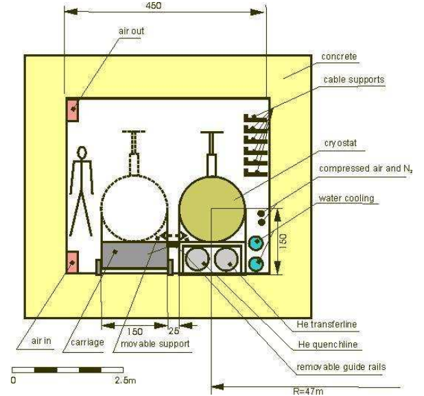
Fig. 45: Possible cross section of the tunnel with cryostat segment in operating position. The transport position is indicated.
