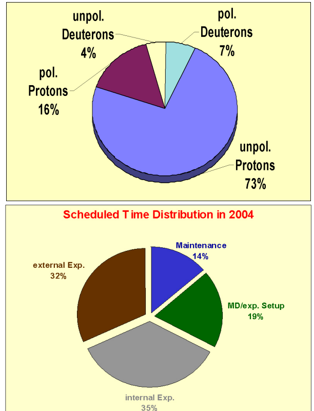
Fig. 36: Upper: Particle beams delivered in 2004. Lower: Beams for experimental groups were equally shared between external and internal target stations. The remaining time was split between machine development and maintenance.
