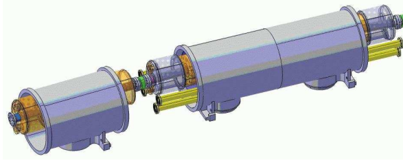
Fig. 47: A detailed study for minimizing the inter magnet distance. The long cryostat segment contains the superconducting dipole magnet, the shorter cryostat segment houses the superconducting quadrupole magnet. The beam pipe for antiprotons is shown in dark blue. The yellow pipes transport the He.
