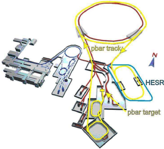
Fig. 41: The antiproton part of the FAIR facility is highlighted in yellow. After production at 3 GeV, antiprotons are accumulated, cooled down, and finally accelerated in the SIS100 (top) to the desired energy. The HESR is the final link in this chain. There the beam properties are refined and data is taken with PANDA.
