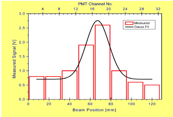
Fig. 40: Gauss fit of beam profile measured by looking at the light from the residual gas.
