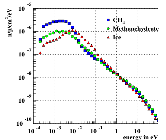
Fig. 25: Comparison of the energy spectra of methane, ice, and methane-hydrate at T=20 K.
