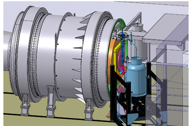
Fig. 59: The new COSY-TOF setup which will include the polarized target.
