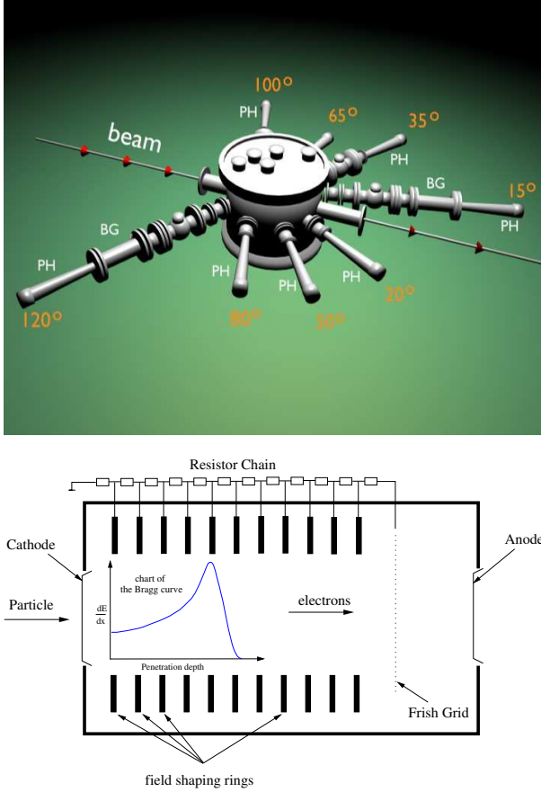
Fig. 5: Upper: Scattering chamber of PISA with the two full detector arms mounted at 15° and 120° equipped with Bragg curve-detectors (BG), channelplate- (inside chamber) and phoswich- detectors. Lower: Schematic layout of the Bragg Curve Detector.
