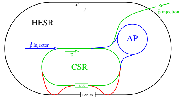
Fig. 55: The proposed accelerator set-up at the HESR (black), with the equipment used by the PAX collaboration in Phase I: CSR (green), AP, beam transfer lines and polarized proton injector (all blue). In Phase II, by adding two transfer lines (red), an asymmetric collider is set up. It should be noted that, in this phase, also fixed target operation at PAX is possible.
