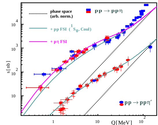
Fig. 12: Excitation functions of the reactions pp \rightarrow pp\eta and pp \rightarrow pp\eta' . Red data points denote COSY-11 results.
