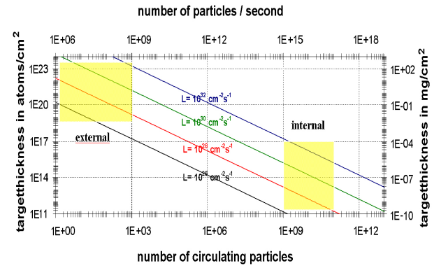
Fig. 39: Peak luminosity for internal and external experiments for different effective target thickness at COSY. Useful Areas are marked in yellow.
