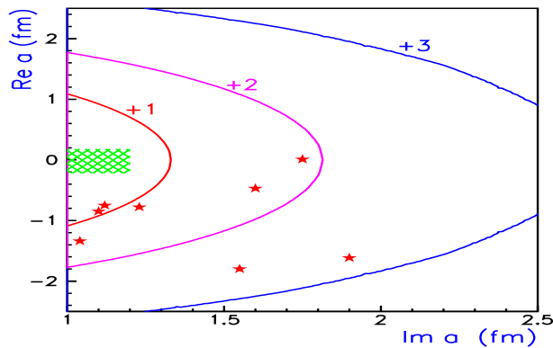
Fig. 15: Real vs. imaginary part of the dK^0 scattering length. The contour lines ( \chi^2 + 1, +2, +3 ) show a fit to pp \rightarrow dK^+K^0 data from ANKE for Q = 46 MeV. The best fit is indicated by the green area. Red stars denote results from model calculations found elsewhere in literature.
