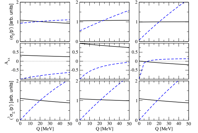
Fig. 31: Model results for \sigma_0 , A_{xx} and the spin triplet cross section ^3\sigma_{\Sigma} for the reaction pp \rightarrow \Theta^+\Sigma^+ . The first, second and third column shows the results for a model where the production mechanism is a pure K -exchange, a pure K^* -exchange and a mixture of both, respectively. Solid lines denote the results for a negative parity pentaquark and dashed lines for a positive parity pentaquark.
