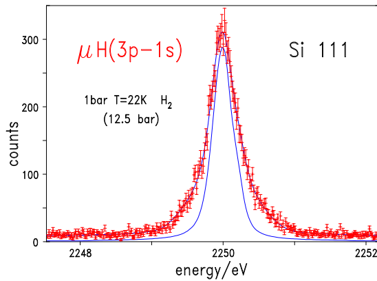
Fig. 29: \mu\text{H}(3\text{p}-1\text{s}) transition measured with the 111 reflection of a spherically curved Si crystal. The narrow line represents the resolution as determined from ECRIT measurements. Its asymmetry is due to the 2 hyperfine components.
