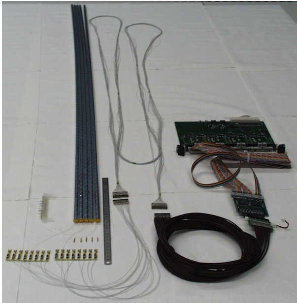
Fig. 52: A photograph of the first 1.5 m straw tube prototype with double sided readout
