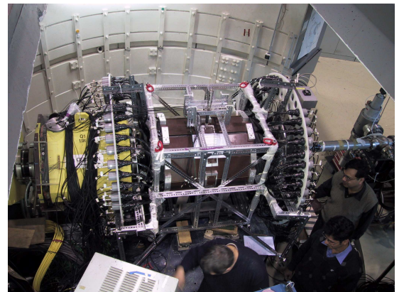
Fig. 7: The ENSTAR detector installed at the target position. The beam enters from the right.
