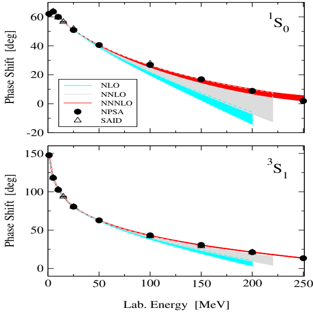
Fig. 32: The S-waves in np scattering. Shown are the theoretical results at NLO (blue band), NNLO (grey band) and N^3\text{LO} (red band) in comparison to the Nijmegen phase shift analysis (circles) and the SAID PSA (triangles).
