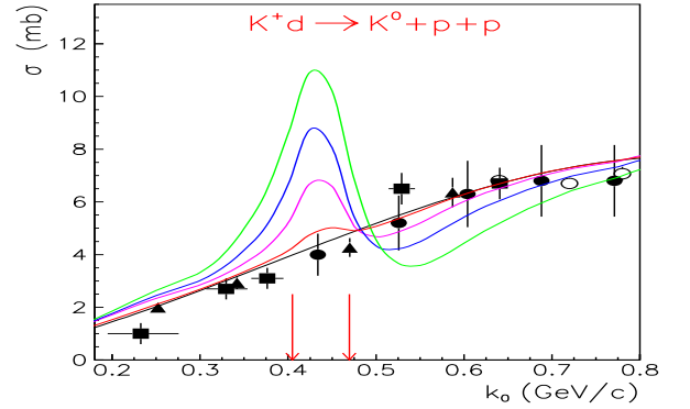
Fig. 30: Total K^+d \rightarrow K^0 pp cross section as a function of the kaon momentum. The curves show our full results for the original Jülich KN model without the \Theta^+ resonance (black line) and the variants with a \Theta^+ and with different widths ( \Gamma_\Theta = 1 MeV - orange; 5 MeV - red; 10 MeV - blue; and 20 MeV - green). The vertical arrows indicate the range of kaon momenta corresponding to the smallest and the largest values found experimentally for the mass of the \Theta^+ resonance.
