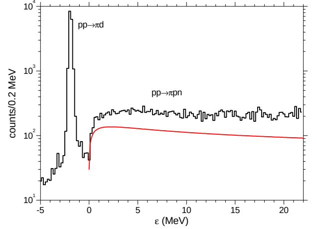
Fig. 23: The results from the GEM experiment (histogram) compared with the prediction (curve) of the S-wave FSI theory (see text).
