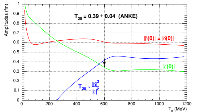
Fig. 22: Predictions for the moduli of the two independent np \rightarrow pn scattering amplitudes at t = 0 , taken from the SAID database, along with the associated prediction of T_{20} for \bar{d}p \rightarrow (pp)_{1S_0}n in impulse approximation. The latter is compared to our preliminary value of T_{20} = 0.39 \pm 0.04 at \frac{1}{2}T_d = 600 MeV.
