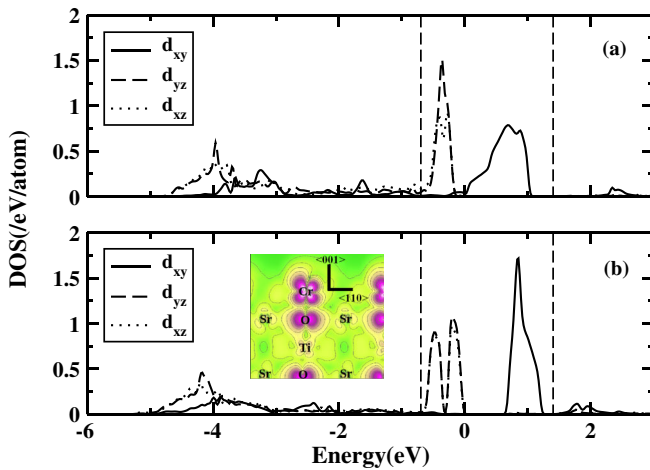
FIG. 2 (color online). The majority spin d_{xz} , d_{yz} , and d_{xy} projected partial density of states for a Cr atom (a) in bulklike geometry and (b) in the optimized ferroelectric geometry for two MLs of SrCrO_3 films on SrTiO_3 . The charge density associated with the antibonding states with d_{xz} and d_{yz} character is shown in inset of (b). Vertical dashed lines indicate the valence band maximum and conduction band minimum of SrTiO_3 . The zero of energy indicates the Fermi energy.
