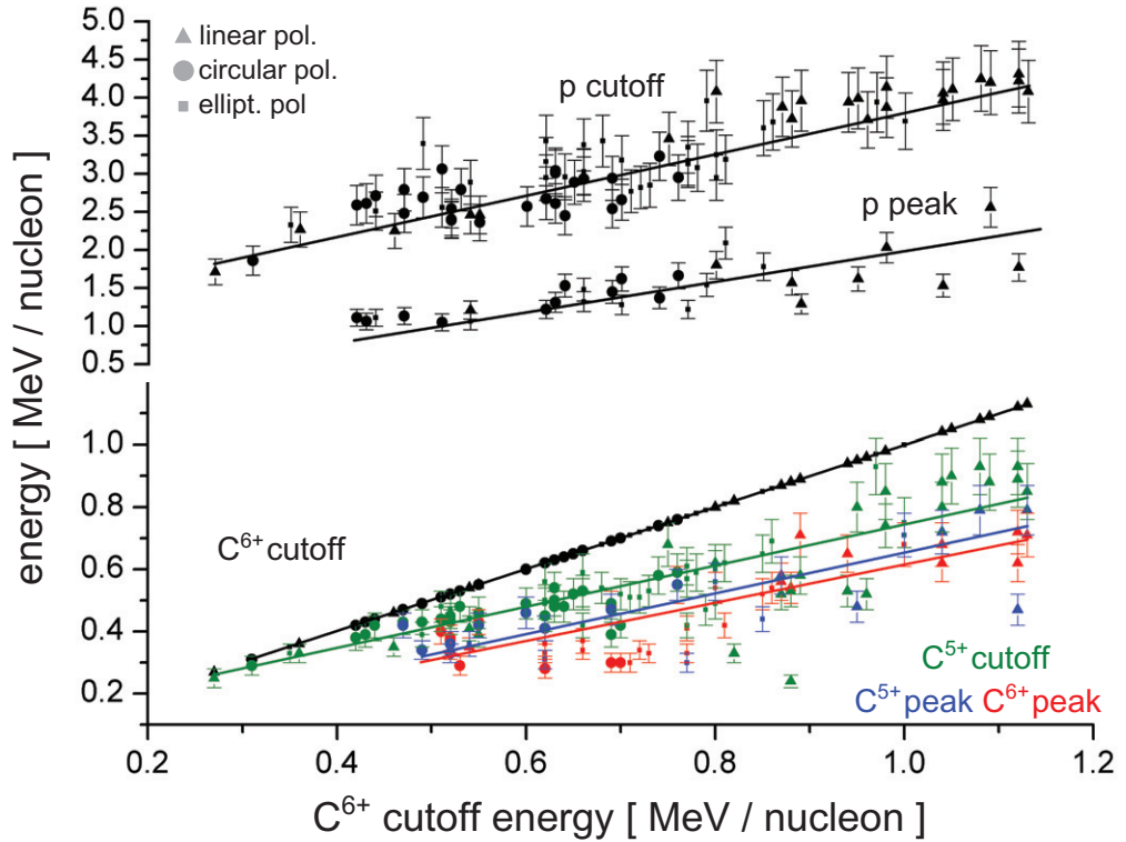
Figure 3. Peak and cutoff energies for protons, C 5+ and C 6+ ions, plotted as a function of the C 6+ cutoff energy for a total number of 111 shot. This presentation also implicitly includes the shot-to-shot variation of the peak intensity. The lowest C 6+ cutoff energy of 0.27 MeV u -1 corresponds to a calculated intensity of 2 \times 10^{18} W cm -2 , the highest value of 1.13 MeV u -1 to the highest intensity of 6 \times 10^{19} W cm -2 . A linear dependence is found for all species. Peak energies for the C 5+ and C 6+ ions have the same dependence and are nearly identical. The ellipticity of the laser pulses showed no effect on the appearance of quasi-monoenergetic peaks even at moderate relativistic intensities, but linear polarization led to higher energies compared to circular polarization. The error bars are determined by the resolution of the spectrometer.
