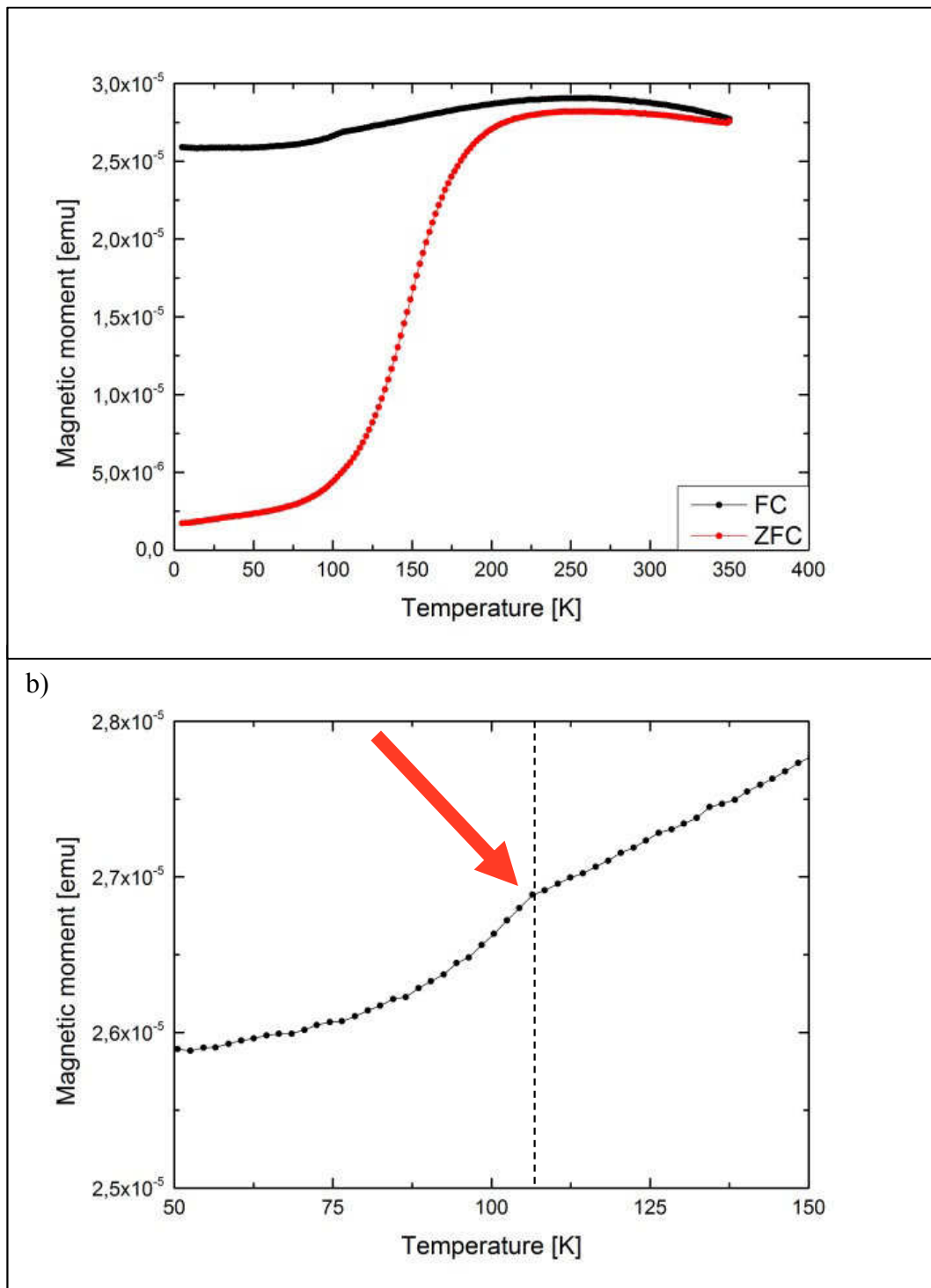
Figure 4.28: a) ZFC (red) and FC (black) curve of a sample diluted with toluene at a ratio of 1:30 that was treated with oxygen plasma for 30 min prior to the deposition of 20 nm of platinum by magnetron sputtering. The measurements were performed in a field of 50 Oe. The transformation of maghemite is enhanced compared to a plasma treatment for 10 min. b) Magnification of the FC curve to show the Verwey transition.
