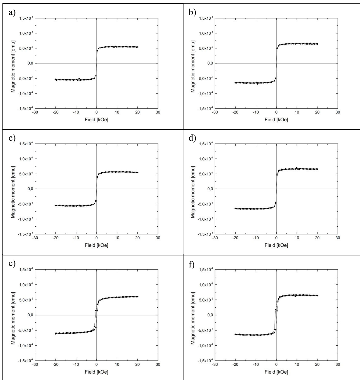
Figure 4.33: Hysteresis curves of samples diluted with toluene at a ratio of 1:30 and treated with oxygen plasma for a,c,e) 10 min or b,d,f) 30 min prior to the deposition of 20 nm gold by magnetron sputtering. The measurements were performed at a,b) 300 K, c,d) 100 K or e,f) 5 K, respectively. They show superparamagnetic behavior and the curves obtained below the blocking temperature are shifted to the left due to exchange bias (Appendix C). They are similar to those obtained for platinum.
