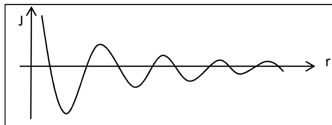
Figure 2.16: Oscillating behavior of RKKY exchange: The exchange integral changes from positive to negative depending on the distance.
