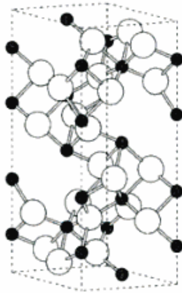
Figure 2.1: Unit cell of hematite: White spheres represent oxygen- and black spheres iron-atoms. Image taken from [53].
