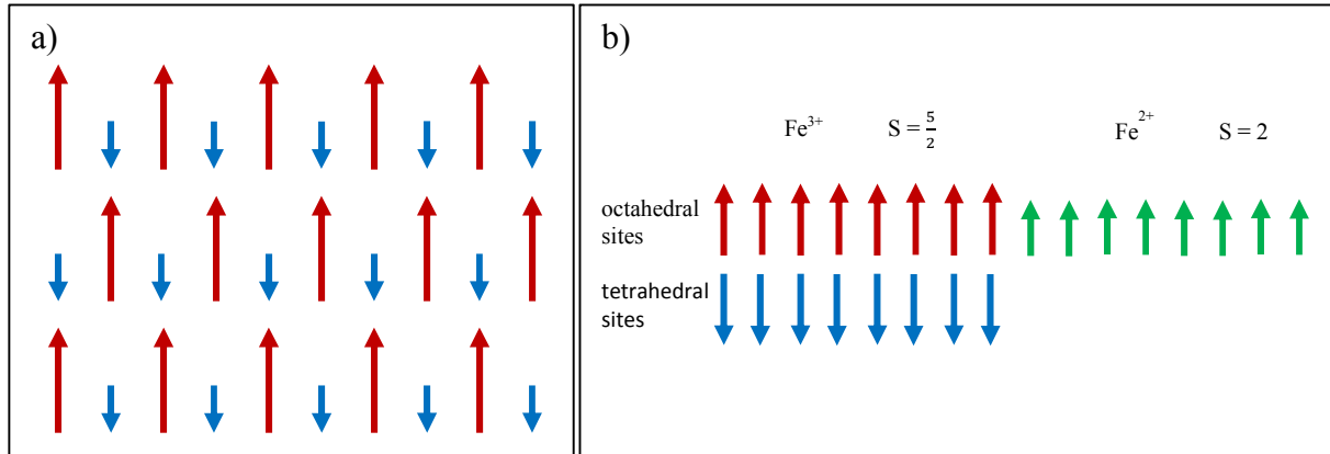
Figure 2.10: a) Ferrimagnetic order. b) Ferrimagnetic order in Magnetite: The red arrows refer to the upward spins of \text{Fe}^{3+} on octahedral sites, blue ones represent downward spins of \text{Fe}^{3+} on tetrahedral sites. Green arrows are upward spins of \text{Fe}^{2+} on octahedral sites.
