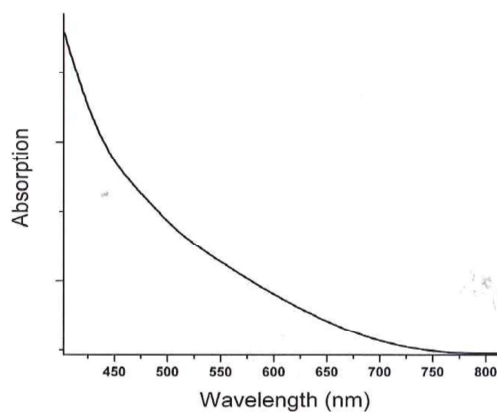
Absorption Spectra
