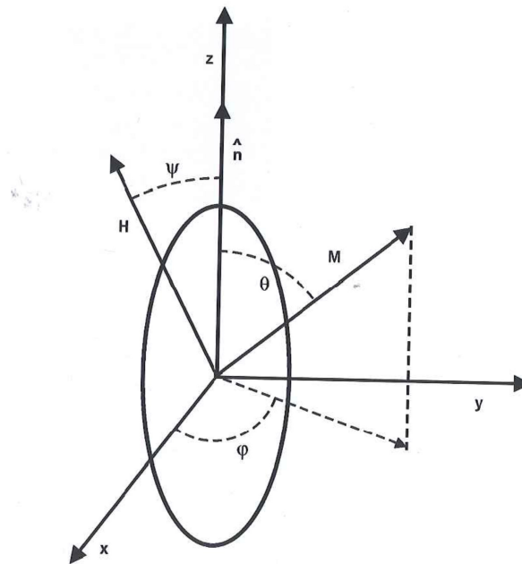
Figure 2.18: Ellipsoidal particle in a magnetic field: The easy axis \hat{n} is in z-direction. \psi is the angle between the external magnetic field H and the easy axis. \theta is the angle between the magnetization M and the easy axis. \varphi is the angle between the projection of \vec{M} into the XY-plane and the x-axis. Image taken from [22].
