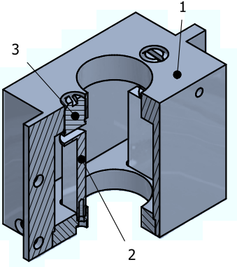
FIG. 9. Three-quarter-section view of the rf cavity of the SFT unit for deuterium (1: the two resonant-field creating conductors, 2: the adjustable capacitor plates, 3: Cu cavity). The inner dimensions of the cavity are 56 mm along B_{\text{stat}} , 36 mm orthogonal to it and 36 mm height. The cross section of the conductors is 14 \times 4 \text{ mm}^2 .
