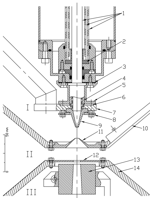
FIG. 5. Technical drawing including the lower end of the heat bridge and the dissociator, the nozzle surroundings, and the first sextupole magnet (in scale, 1: discharge and coolant-guiding tubes, 2: coolant-reversal piece, 3: heat flow reducing Teflon washer, 4: sliding heat connection, 5: stainless steel support, 6: groove for nozzle-heating element, 7: lower end of the Cu heat bridge, 8: nozzle fixture, 9: nozzle, 10: baffle, separating the chambers I and II, with a viewport, 11: stainless steel beam skimmer, 12: Cu diaphragm, 13: first sextupole magnet, and 14: baffle separating the chambers II and III.
