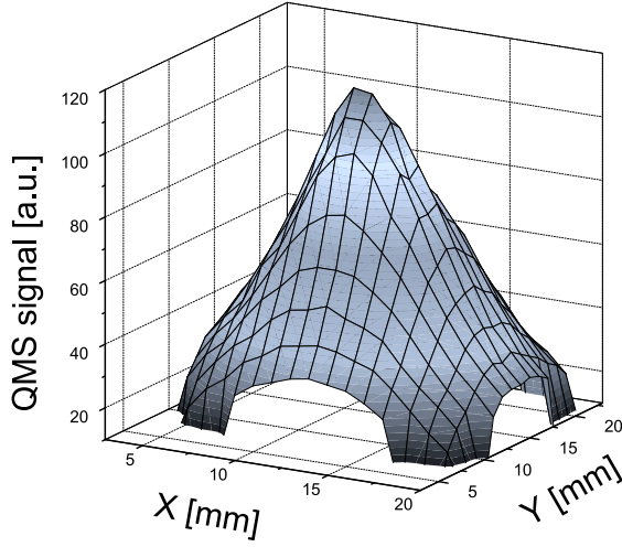
FIG. 21. The distribution corresponding to that of Fig. 20 after nozzle-to-skimmer adjustment resulting in azimuthal symmetry.
