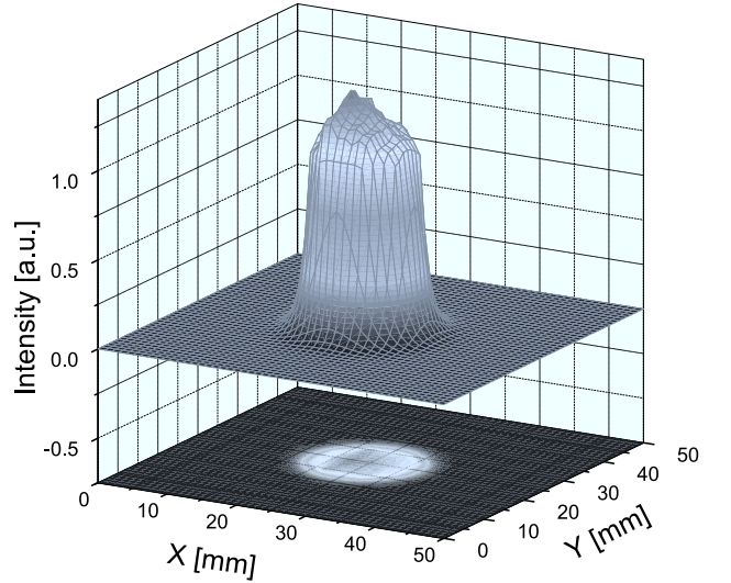
FIG. 10. Two-dimensional profile of the atomic hydrogen beam 10 mm from the nozzle, deduced from recombination heating of gold-plated tungsten wires of 5 \mu\text{m} in a 8 \times 8 wire grid.
