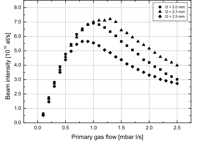
FIG. 15. Intensity of the hydrogen beam (states |1> and |2>) injected into the compression tube as function of the primary molecular gas flow for different nozzle diameters D (nozzle temperature 60 \text{ K} , dissociator power 300 \text{ W} ).
