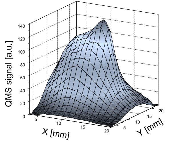
FIG. 20. Two-dimensional distribution of the atomic hydrogen component of the beam at z = 567 mm before the nozzle-to-skimmer adjustment, showing a distinct deviation from azimuthal symmetry.
