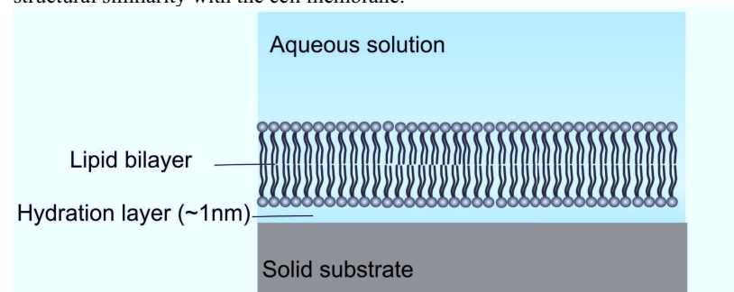
Figure 1.11: Supported lipid bilayer is a double layer of lipid molecules formed on a solid surface, separated from it by a thin aqueous layer and covered by aqueous solution.
