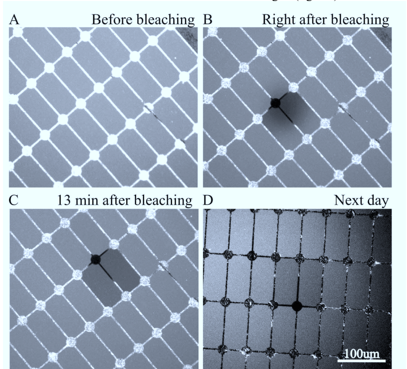
Figure 7.3: Bleaching of the SLB formed on glass patterned with the Cr. The bleached spot falls into two rectangles (B). These rectangles are darker than others in the image made 13 min after bleaching due to diffusion (C). The Cr lines are bright in the first three images (A-C) due to adsorption of liposomes. In the last image (D), made on the next day after bleaching, the lines are black as the liposomes were washed away.
