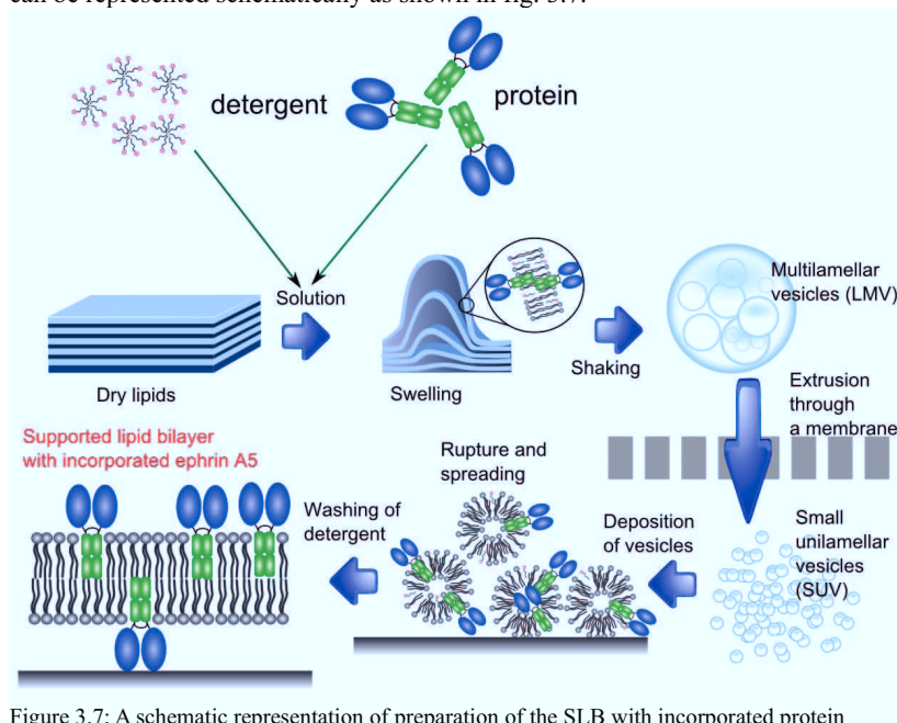
Figure 3.7: A schematic representation of preparation of the SLB with incorporated protein
