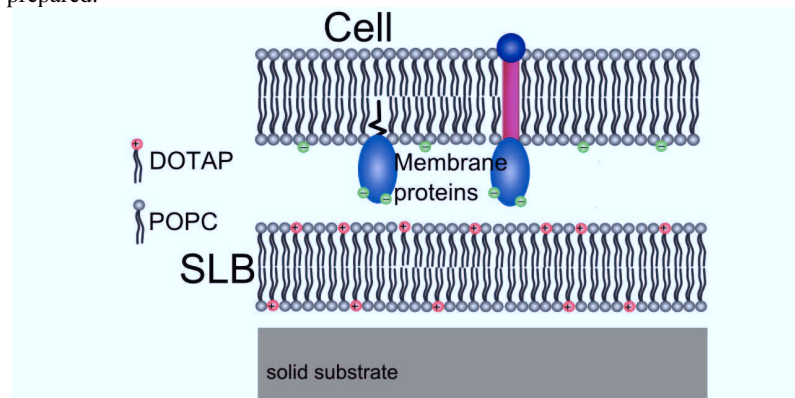
Figure 2.2: Illustration of the principle of providing cell adhesion to the SLB by electrostatic interaction. Positively charged lipid (DOTAP) is added to the SLB made of zwitterionic lipid (POPC). Cell membrane is negatively charged due to surface carbohydrates, proteins and some lipids. Interaction of these charges with the positive charge of the SLB can provide cell adhesion.
