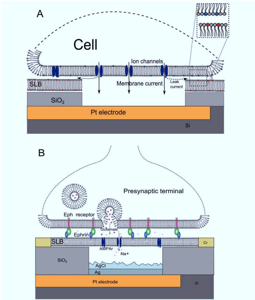
Figure 8.1: (A) A schematic representation of the SLB enhanced MEA: Positively charged SLB is formed on the surface of the chip (the area of the electrode stays free as liposomes can not fuse on metal). Due to electrostatic interaction of negatively charged cell membrane with the SLB the cell adheres to it tightly, reducing the gap between the cell membrane and the surface making the leak current lower. (B) The concept of an artificial synapse using SLB: a lipid bilayer is suspended over a planar AgCl electrode (AgCl is used to measure currents) of a MEA. Synapse adhesion protein (Ephrin) promotes formation of the synapse. Receptors, incorporated into the SLB (AMPAr in the present scheme) sense synaptic vesicle release and pass ions upon neurotransmitter binding.
