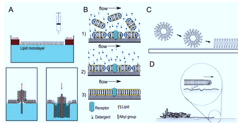
Figure 1.13: Methods of SLB preparation: (A) Langmuir-Blodgett technique [83], (B) deposition from detergent solution [82], (C) vesicle deposition, (D) spreading from a lipid reservoir [81].
