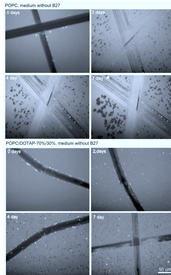
Figure 5.8: Formation of holes in SLBs kept in cell culture medium. Series of images taken on different days for SLB made of pure POPC and 70%-30% POPC-DOTAP mixture. The scale bar is the same for all images.
