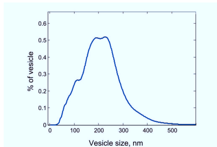
Figure 4.1: Distribution of size of POPC vesicles produced by extrusion through 100 nm membrane as measured by particle tracking analysis. Total number of measured vesicles was 2653.
