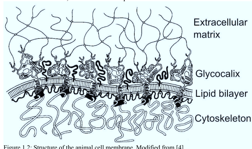
Figure 1.2: Structure of the animal cell membrane. Modified from [4].
