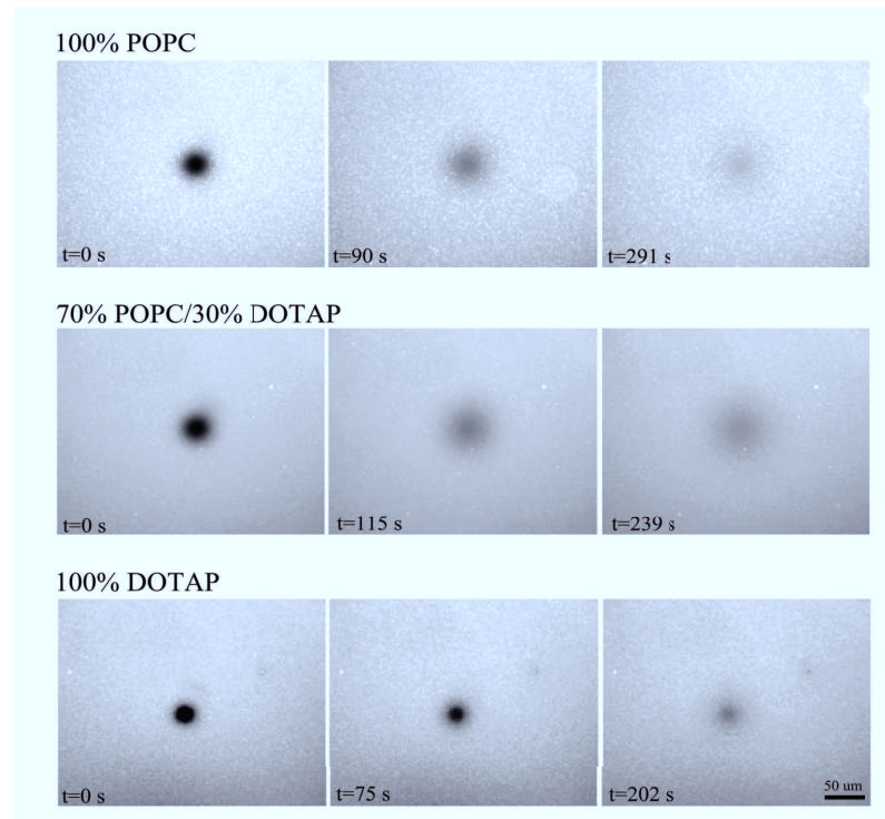
Figure 4.4: Time series of micrographs showing fluorescence recovery after photobleaching (FRAP) for a spot bleached in SLBs of different types. The scale bar is identical for all images.
