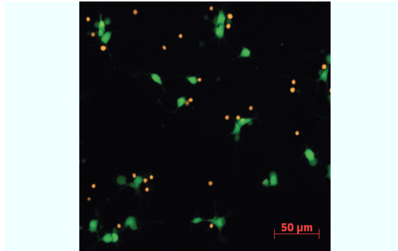
Figure 3.12: An example of staining of live cells with calcein-AM (green fluorescence) and dead cells with ethidium homodimer (red fluorescence). Neurons of DIV1 are shown.
