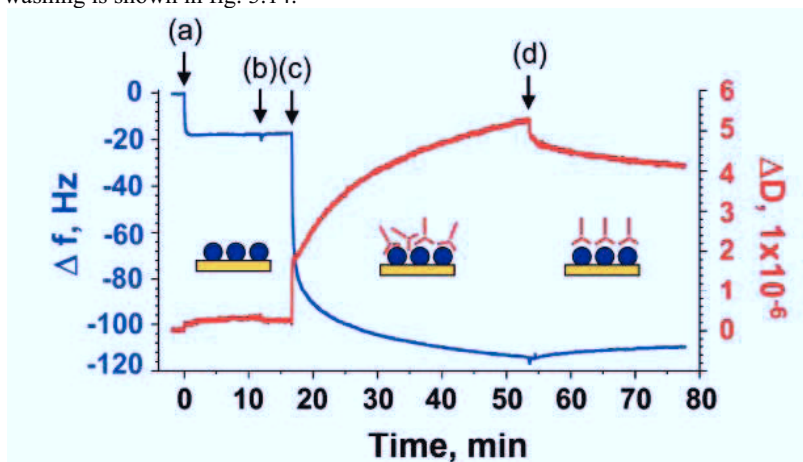
Figure 3.14: The adsorption of human serum albumin (a) and an antibody for human serum albumin (c). Steps b and d correspond to buffer rinses. Frequency changes ( \Delta f ) are shown in blue, and dissipation changes ( \Delta D ) are shown in red. The frequency change of step (a) and lack of dissipation change indicating the rigid characteristics of the human serum albumin film as it adsorbs on the surface. In contrast, the adsorption of the antibody at (c) gives a large frequency and dissipation change, indicating both mass adsorbed and increased viscoelastic characteristics due to the incorporation of water [139].
