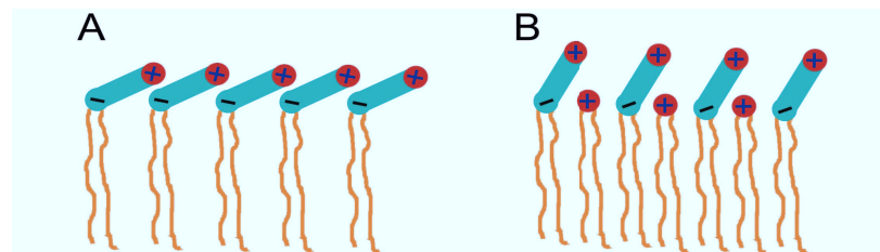
Figure 4.6: (A) The SLB made of zwitterionic lipids and (B) the SLB made of mixture of zwitterionic and positively charged lipids. Positively charged lipid molecules make the heads of the zwitterionic molecules stand vertically and occupy less space in the bilayer. This leads to denser packaging of the molecules. Modified from Zhang et al. [171]
