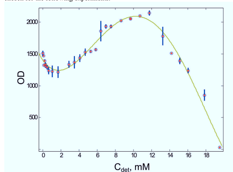
Figure 6.1: The dependence of optical density (OD) of suspension of lipid vesicles made of POPC on the concentration of detergent ( n -octyl- \beta -D-glucoside). The measurements were done at \lambda=500 nm.
