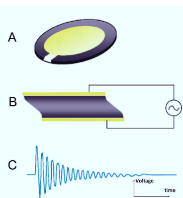
Figure 3.13: (A) A circular piece of quartz is sandwiched between two metal electrodes used for QCM-D. (B) A schematic representation of mechanical oscillations in the quartz crystal by application of variable voltage. (C) The decay of the amplitude of the oscillations over time after switching of voltage.
