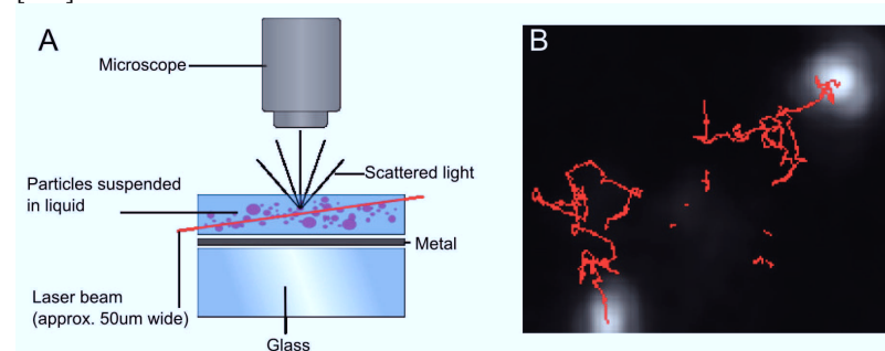
Figure 3.15: (A) A schematic representation of the set up for Nanoparticle Tracking Analysis [142]. (B) An enlarged image of typical tracks of particles moving under Brownian motion. Note: the particles are not being imaged, structural information, such as shape of the particle is below the resolving power of the optical microscope used [143].
