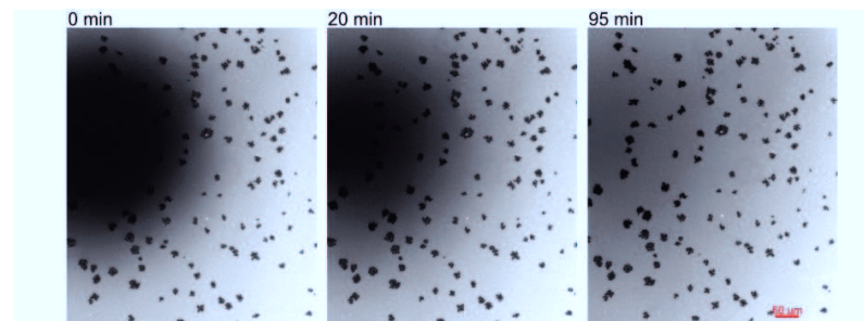
Figure 5.10: A FRAP experiment showing the recovery of fluorescence in the POPC SLB of 7 days old kept in cell culture medium without B27 supplement. The scale bar is the same for all images.
