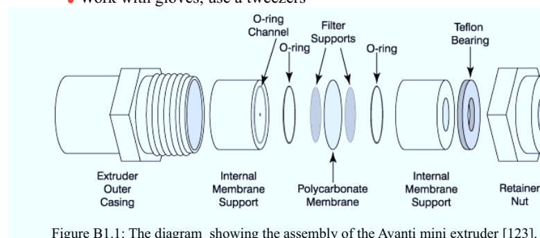
Figure B1.1: The diagram showing the assembly of the Avanti mini extruder [123].
