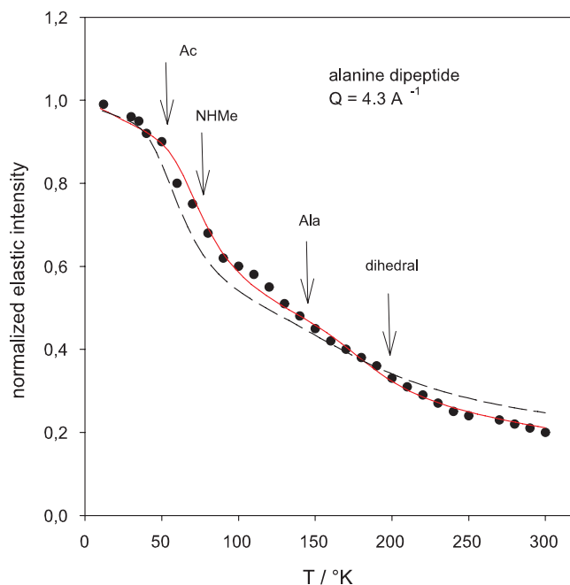
FIG. 11. Normalized elastic scattering intensity I_{\text{el}}^{\text{NG}}(Q = 4.3 \text{ \AA}^{-1}, \tau_{\text{res}} = 137 \text{ ps}) of alanine dipeptide crystal powder (back-scattering spectrometer IN13, ILL, Grenoble) and a 4-component fit (Eq. (34), red line) accounting for the fast C-(Ac) and N-(NHMe) terminal blocking methyl groups ( T_{\text{on}} \cong 50 K), the side chain methyl(Ala) ( T_{\text{on}} \cong 150 K), and the dihedral transitions ( T_{\text{on}} \cong 210 K). To show the sensitivity of the fit, the dashed line accounts for Ac and the Ala methyls only. The arrows indicate the location of the respective T_{\text{on}} values.
