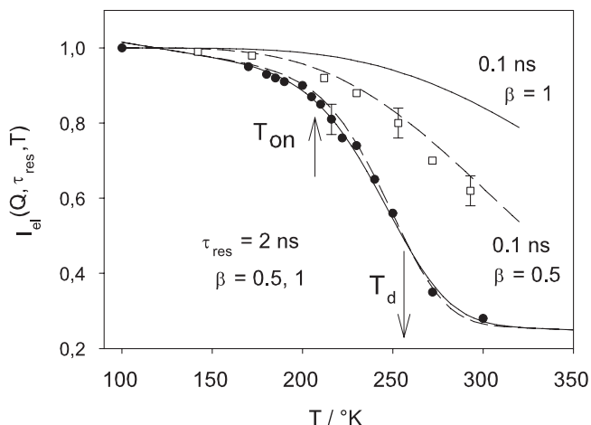
FIG. 7. Elastic scans of protein hydration water at Q = 1 \text{ \AA}^{-1} : full circles: C-PC with 0.3 g/g \text{H}_2\text{O} (full circles) at a resolution of \tau_{\text{res}} \approx 2 \text{ ns} (SPHERES), normalized at T_0 = 100 \text{ K} , open squares: \text{H}_2\text{O} -hydrated myoglobin at a resolution of 0.1 ns (IN13), lines: fits to the stretched exponential model of Eq. (27) including a vibrational Debye Waller factor at \beta = 0.5 (full line) and 1.0 (dashed). The temperatures T_{\text{on}} and T_{\text{d}} are indicated by arrows. The parameters are given in the text.
