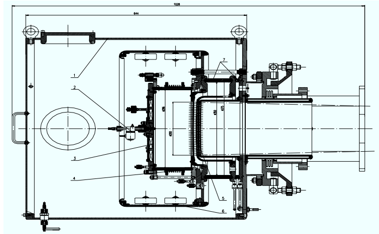
Fig.6. Ion source with an RF-discharge plasma box: 1- metal case, 2 – pulse gas valve and trigger unit, 3 – RF-plasma box, 4 – RF-coil, 5 – grids, 6 – internal magnetic and electrostatic shield, 7 – ceramic insulator.
