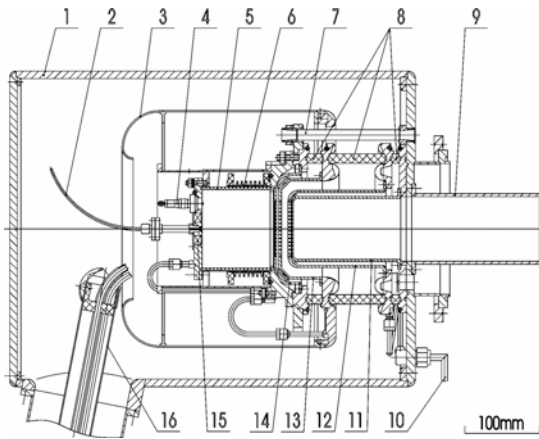
FIG. 3. RF ion source: 1 soft metal case; 2 gas feeding capillary tube; 3 inner magnetic shield; 4 trigger; 5 ceramic wall; 6 RF coil; 7 pull stud (insulator); 8 ceramic spacers; 9 beam duct; 10 water inlet manifold; 11 grounded grid; 12 accelerating grid; 13 extracting grid; 14 plasma grid; 15 magnets; 16 co-axial feedthrough.
