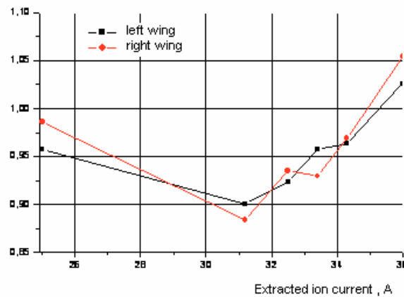
Fig.8 Beam divergence inferred from the beam power density profile measured on calorimeter wings
