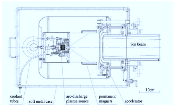
FIG. 1. Schematic view of ion source with an arc-discharge plasma box.
