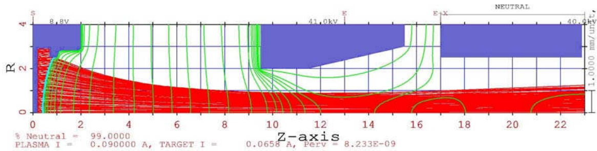
Fig.7 Plot of ion trajectories and equipotentials in elementary cell.
