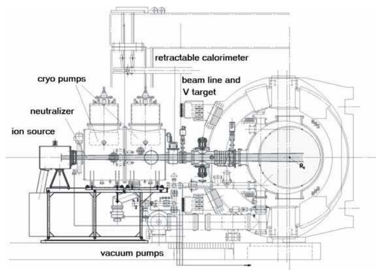
FIG. 2. Diagnostic neutral beam injector setup at TEXTOR.
