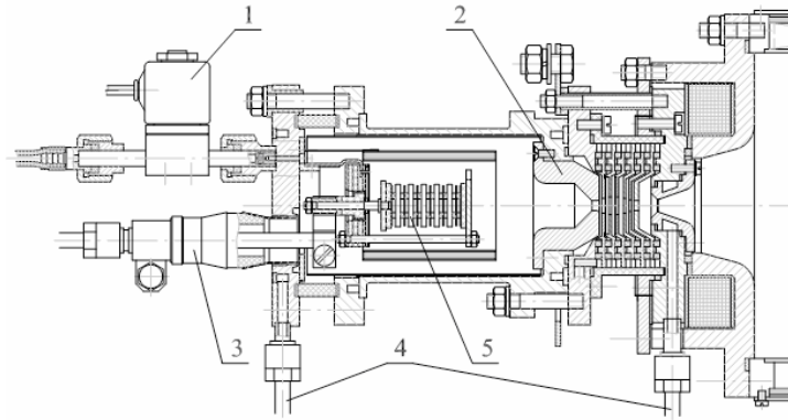
Fig. 5 General view of cathode assembly and electron emitter: 1 – cathode gas valve; 2 – cathode insert; 3 – heater feedthrough; 4 – water manifolds; 5 – electron emitter.
