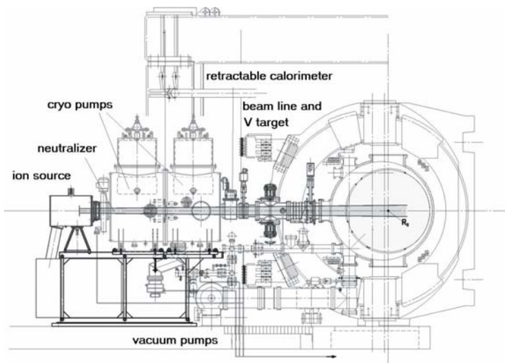
FIG. 2. Diagnostic neutral beam injector setup at TEXTOR.
