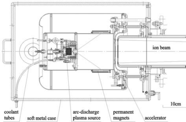
FIG. 1. Schematic view of ion source with an arc-discharge plasma box.
