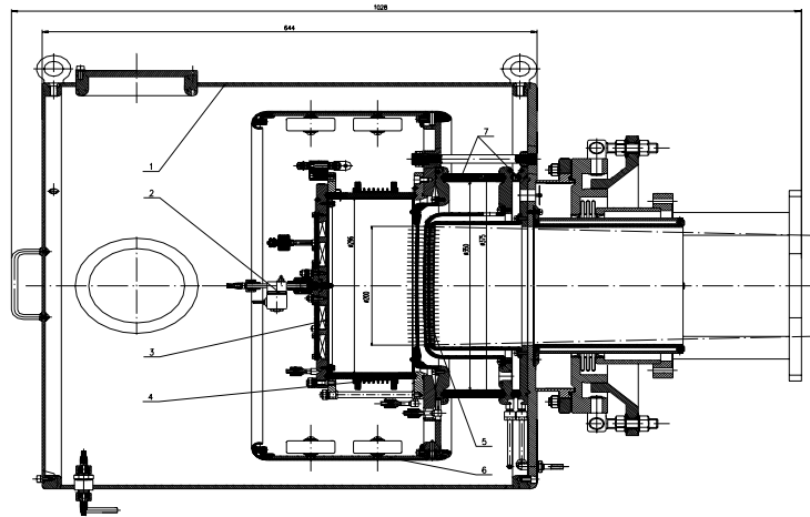
Fig.6. Ion source with an RF-discharge plasma box: 1- metal case, 2 – pulse gas valve and trigger unit, 3 – RF-plasma box, 4 – RF-coil, 5 – grids, 6 – internal magnetic and electrostatic shield, 7 – ceramic insulator.
