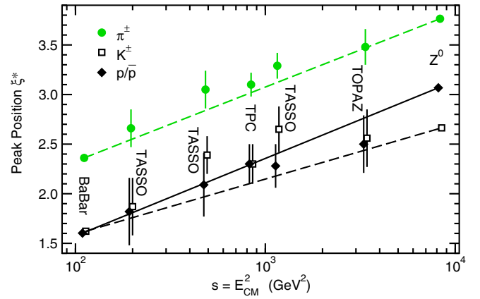
FIG. 16 (color online). Peak positions \xi^* vs CM energy for pions (circles), kaons (squares) and protons (diamonds) on a logarithmic horizontal scale. The lines join our points with those from the averages of the Z^0 experiments.
