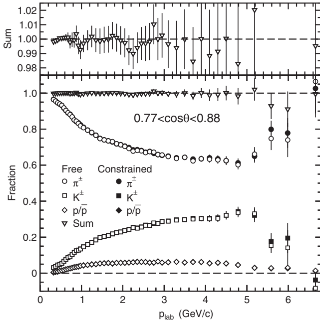
FIG. 4. Raw \pi^\pm (circles), K^\pm (squares) and p/\bar{p} (diamonds) fractions measured in \theta 6 , the most forward \cos \theta_{\text{lab}} region. The solid (open) symbols represent the results with (without) the constraint that they sum to unity in each p_{\text{lab}} bin. They are indistinguishable in most cases. The sums of unconstrained fractions are shown as the triangles, and in an expanded view in the upper plot. The error bars include statistics and the systematic uncertainties arising from the calibration of the particle identification efficiencies.
