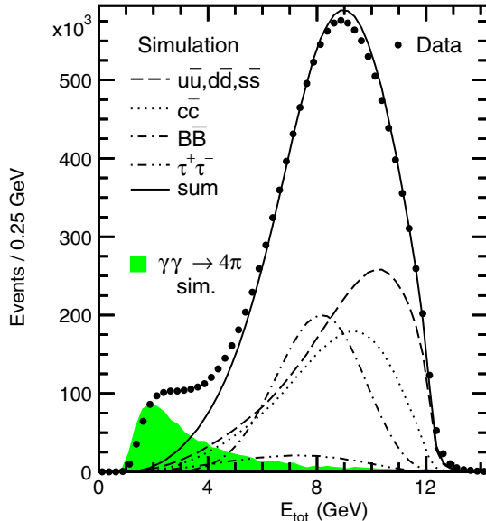
FIG. 1 (color online). Distributions of the total visible energy per event, after all other selection criteria have been applied, in the on-resonance data and simulation. The sum of the hadronic and \tau -pair simulations is normalized to the data in the region above 5 GeV, and the \gamma\gamma simulation is normalized arbitrarily.
