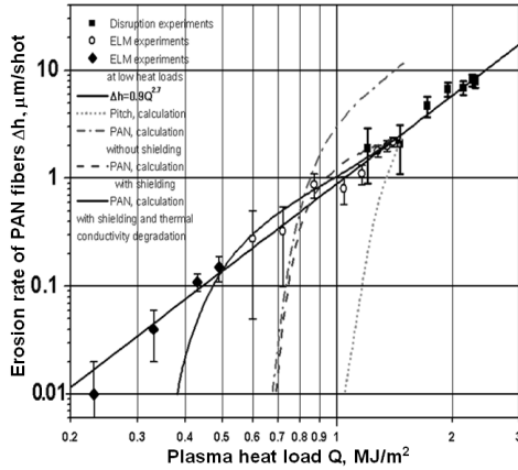
Figure 1. Experimental and numerical estimation of the erosion rate of PAN fibres [Klimov10, Riccardi10 & references therein]
