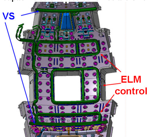
Figure 5.a. Layout of the proposed in-vessel coils for vertical stability and ELM control in ITER.
