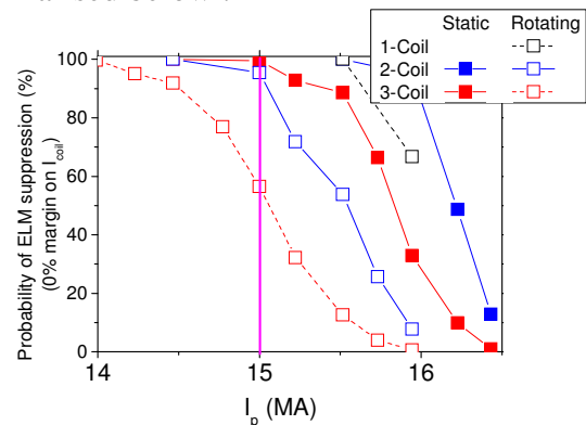
Figure 5.b. Cumulative probability for ELM suppression for n (1, 2, 3) malfunctioning coils in ITER versus plasma current for static and rotating perturbations
