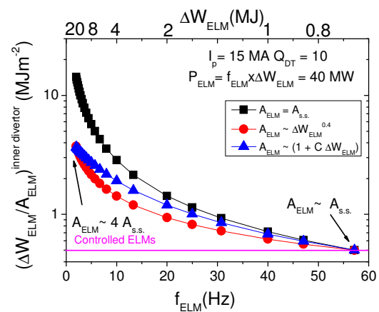
Figure 3. Expected ELM energy flux at the inner divertor ( \Delta W_{ELM}/A_{ELM} ) in ITER versus ELM frequency ( f_{ELM} ) or ELM size ( \Delta W_{ELM} ) for various assumptions regarding the dependence of the effective area for ELM energy deposition ( A_{ELM} ) on \Delta W_{ELM} .
