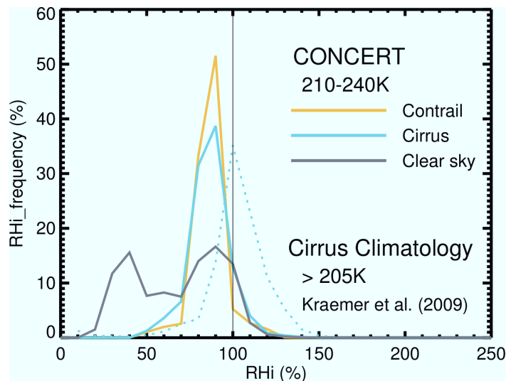
Fig. 2. Left panel: Frequency of occurrence of RH_{ice} in contrails, cirrus and clear sky during CONCERT (solid lines) and for a broad range of cirrus conditions (dotted line, from Krämer et al., 2009, 5.6 h observation time, 28 flights). CONCERT sampling times: clear sky 0.9 h, cirrus 2.3 h, contrails 1.7 h, flight dates: 29 October (1 flight), 17 November (2 flights), 19 November (2 flights), 20 November (1 flight). Right panel: large ice crystals observed inside of the cirrus and contrails during CONCERT.
