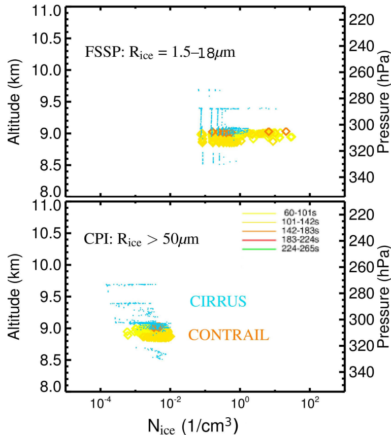
Fig. 6. Vertical profiles of the ice crystal number N_{\text{ice}} for different size intervals in the 2. cirrus (turquoise) period of the 1st flight on 17 November 2008, including the A343 contrail (coloured by age, see legend in bottom panel). Cloud particle instrumentation: FSSP – Forward Scattering Spectrometer Probe and CPI – Cloud Particle Imager, for more information see Sect. 2.
