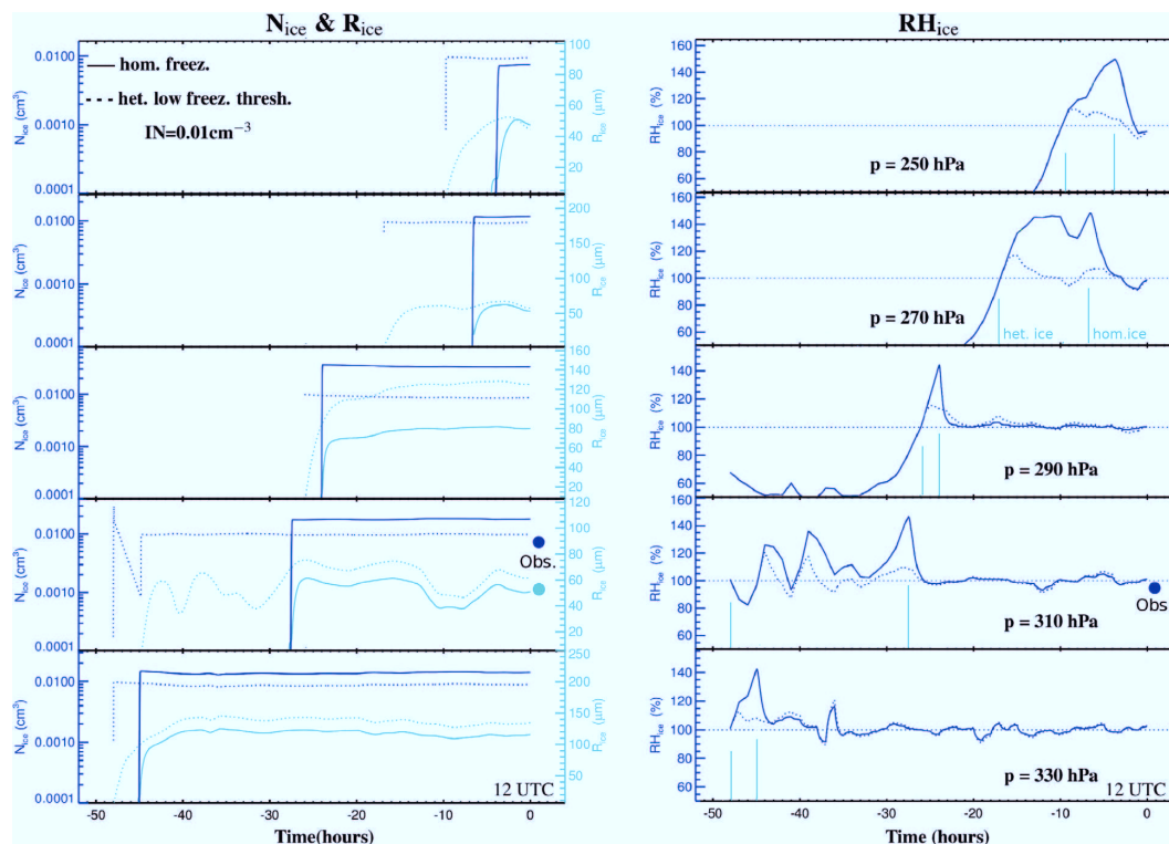
Fig. 10. MAID simulations along the trajectories shown in Figs. 8 and 9 (solid line: homogeneous freezing, dotted line: heterogeneous freezing); N_{\text{ice,MAID}} : number, R_{\text{ice,MAID}} : mean mass size of ice crystals. In the 310 hPa panels, big dots denotes the observations ( N_{\text{ice,obs}} : peak number, R_{\text{ice,obs}} : approximate size of ice crystals, see Fig. 6, bottom panel; RH_{\text{ice}} see Fig. 5).
