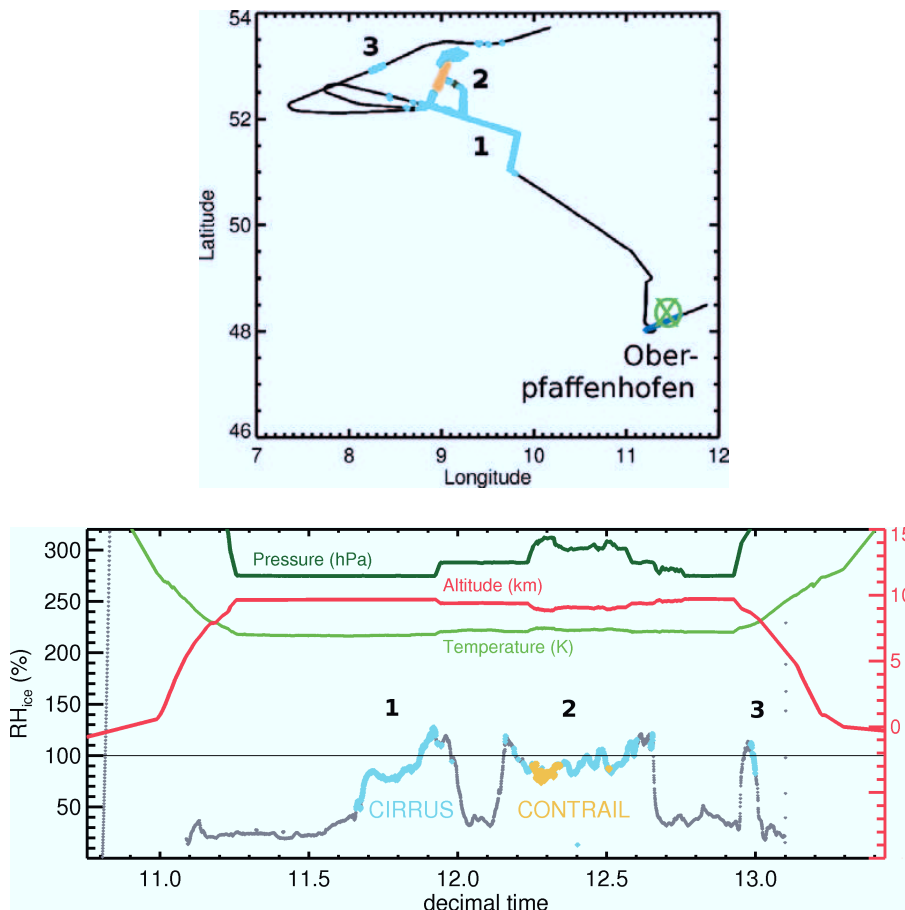
Fig. 4. Survey of DLR Falcon's 1st flight on 17 November 2008, 11:00 to 13:20 UTC. Top panel: flight path, turquoise/orange indicate cirrus/contrails. Bottom panel: temperature, pressure, altitude and RH_{ice} along the flight path. DLR Falcon crossed three cirrus sections, labeled 1–3 in the following.
