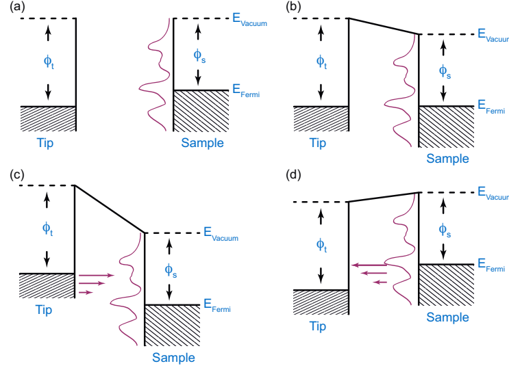
Figure III.4: Sketch of the energy diagrams for a tunneling system. The sample DOS is indicated as a magenta line, whereas the DOS of the tip is considered to be featureless (constant). (a) Tip and sample in high distance from each other: No interaction. (b) Tip and sample in tunneling contact. Electrons are tunneling until both Fermi levels are in equilibrium. (c) Positive bias voltage at the sample. Electrons are tunneling from the tip to the sample, which results in probing the unoccupied sample states. (d) Negative bias at the sample. Electrons are tunneling from the sample to the tip, which results in probing the occupied sample states (as in [41]).
