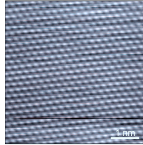
Figure IV.7: Atomic resolution STM image of a HOPG surface taken after in-situ cleaving. The image exhibits a clean surface without defects or adsorbates. [ I_T = 1 nA, V_{\text{Bias}} = 0.2 V, z-color scale: black ( z=0 pm) to white ( z=180 pm)]
