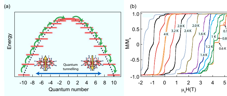
Figure II.1.: (a) Schematic representation of the potential barrier separating the two spin ground states of an SMM. Magnetization reversal can occur due to quantum tunneling of the magnetization or by thermal excitation, respectively. (b) Hysteresis loops for the \{Mn_{12}\} SMM complex at various temperatures between 4 and 0.1 K. The characteristic steps generated by quantum tunneling of the magnetization are observed at resonant fields. (taken from [7])
