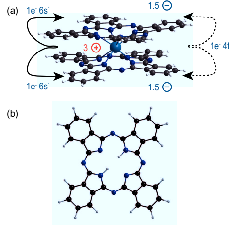
Figure II.2: (a) \text{NdPc}_2 double-decker phthalocyanine molecule. The bonding of the molecule is mainly of electrostatic character. The central Nd atom transfers three electrons to the two phthalocyanine rings. (b) phthalocyanine molecule with two hydrogen atoms in the center. The molecule consists of four isoindole rings linked by nitrogen atoms. Atomic representation: hydrogen (white), carbon (grey), nitrogen (dark blue) and neodymium (blue).
