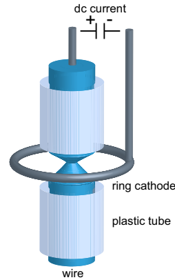
Figure IV.2: Setup for electrochemical wet etching of STM tips. A constant current is applied between the ring cathode and the tip. Plastic tubes prevent the tip from being etched in unwanted regions.
