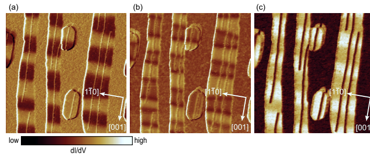
Figure VII.6.: dI/dV maps of the second AL of Fe on W(110) showing distinct out-of-plane spin contrast. Images recorded at (a) V_{\text{bias}} = -0.3 V, I_T = 2.5 nA, (b) V_{\text{bias}} = -0.1 V, I_T = 1.6 nA and (c) V_{\text{bias}} = 0.7 V, I_T = 3 nA. For V_{\text{bias}} = -0.1 V a contrast reversal compared to the other images is observed. Color code is individually scaled. (Image sizes: 180 \times 180 nm 2 )
