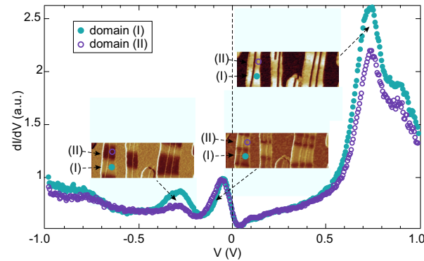
Figure VII.7: dI/dV spectra recorded above the two different out-of-plane domains of the second AL of Fe on W(110). The domains (I) and (II) are marked in the dI/dV maps shown as insets. Both, dI/dV spectra and maps exhibit the contrast reversal around V_{\text{bias}} = -0.1 V. (Tip stabilized at V_{\text{bias}} = -1 V, I_T = 1 nA, V_{\text{mod}} = 20 mV rms.)
