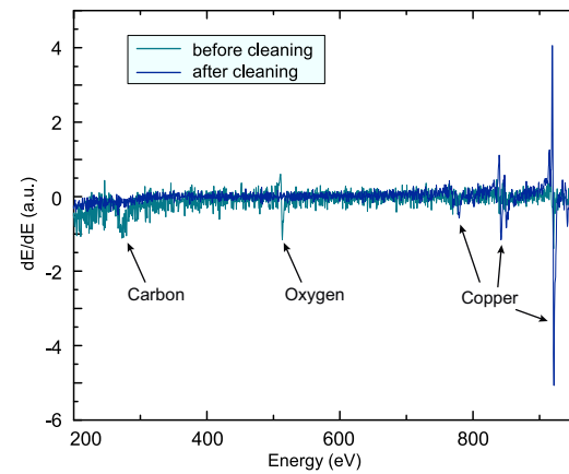
Figure IV.6: Auger spectrum of the Cu(100) surface before and after the cleaning process. (Derivative shown for better visualization) After the oxygen annealing and high temperature heating, the features corresponding to carbon and oxygen almost completely disappeared, indicating a clean surface.
