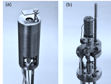
Figure IV.9: (a) Evaporator for molecule deposition. (b) After removing the heat shielding, the Cu screw with the drilled cavity and the attached filament is visible.
