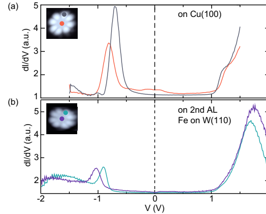
Figure VIII.2: dI/dV spectra obtained above the center and the organic ligand of the NdPc 2 molecule adsorbed on (a) Cu(100) and (b) Fe on W(110). [ f_{\text{mod}} = 2.7 \text{ kHz} , V_{\text{mod}} = 30 \text{ meV rms} ; (a) tip stabilized at I_T = 1 \text{ nA} and V_{\text{bias}} = -1 \text{ V} and (b) tip stabilized at I_T = 2 \text{ nA} and V_{\text{bias}} = 2 \text{ V} ]
