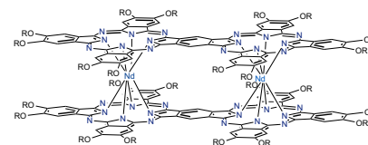
Figure IX.2: Possible molecular structure comprising two magnetic centers [118].
