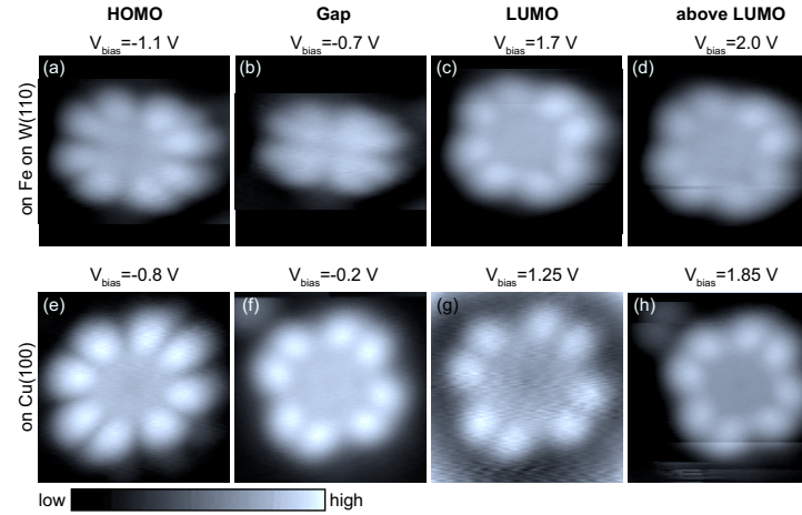
Figure VIII.3: Comparison of constant current topography images of the NdPc 2 molecule adsorbed on Fe on W(110) (upper row) and Cu(100) (lower row) for the HOMO, the gap, the LUMO and bias voltages above the LUMO. Bias voltages as indicated in the Figure and tunneling currents are: (a) I_T = 1 nA, (b) I_T = 1 nA, (c) I_T = 2 nA, (d) I_T = 2 nA, (e) I_T = 1 nA, (f) I_T = 1 nA, (g) I_T = 1 nA, (h) I_T = 1 nA, (i) I_T = 1 nA. Color code is individually scaled. (Image sizes: 2.7 \times 2.7 nm 2 )
