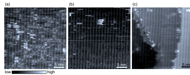
Figure V.5.: (a) Overview image of the Au(100) surface after evaporation of the NdPc 2 molecules. The 5 \times 1 surface reconstruction of the substrate is visible and no molecules are observed. Smaller adsorbate sit at the step edges and on the surface and prohibit stable tunneling. (b) After three times scanning along the same surface region, less adsorbates are observed and the tunneling is more stable as compared to (a). (c) Adsorbates associated to isoindole or phthalonitrile molecules, are located at the step edges of the crystal. [(a), (b) V_{\text{bias}} = 1 \text{ V} and I_{\text{T}} = 0.5 \text{ nA} and (c) V_{\text{bias}} = -1 \text{ V} and I_{\text{T}} = 0.5 \text{ nA} ]
