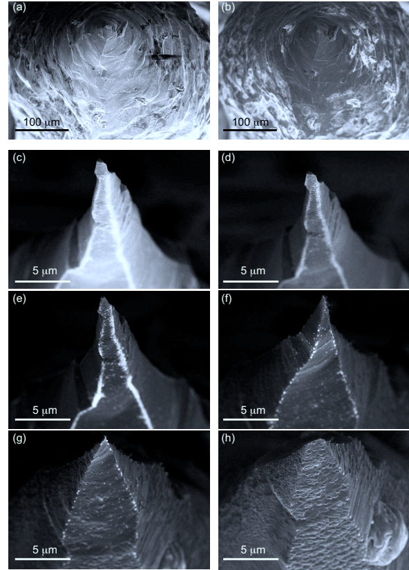
Figure IV.5.: SEM images of Cr-tips, showing the influence of the electron bombardment. In (a) and (b) a tip is shown before and after a flash for 30s at a power of 1.75 VA. The bright contaminations on the upper part of the tip are removed. (c)-(h) show the evolution of the un-flashed tip in (c) after five heating circles. Amount and kind of contaminations are changed together with a strong modification of the tip shape. (d) 10s at 1 AV, (e) 10s at 2 AV, (f) 20s at 2 AV, (g) 30s at 2 AV, (h) 30s at 1.5 AV
