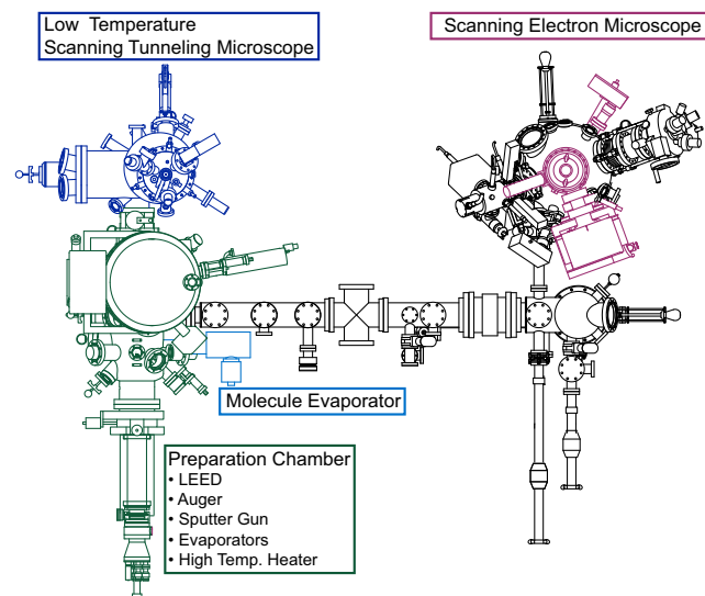
Figure IV.1.: Schematic drawing of the NanoSpintronicsClusterTool.
