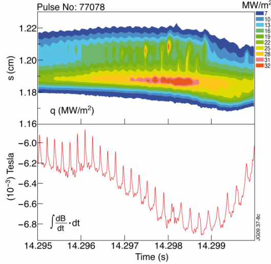
Fig. 6: heat flux contours at outer strike, measured with IR, and integrated magnetic signal showing correlation of heat pulses with rotation of current structure. Reprinted figure with permission from E.R. Solano et al., Phys. Rev. Lett. 104, 185003 (2010)
