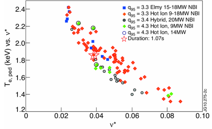
Fig. 5: T_{e,ped} vs. pedestal collisionality v^* at the onset of the MH-OMs.
