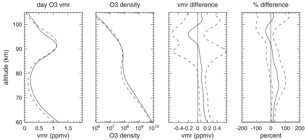
Figure 2. Profiles of ozone vmr (first panel; units ppmv) and ozone density (second panel; units \text{cm}^{-3} ) from SABER 9.6 \mu\text{m} (solid) and 1.27 \mu\text{m} (dashed) retrievals averaged over all seasons and latitudes for January 2002–July 2012. The difference profiles show absolute difference (third panel; ppmv) and relative difference (fourth panel; %) for the 9.6 \mu\text{m} ozone minus the 1.27 \mu\text{m} ozone. The dashed lines give \pm the de-biased standard deviation.
