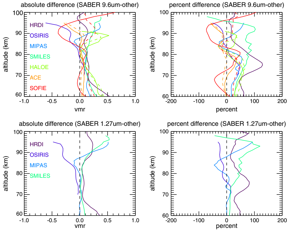
Figure 6. Top shows profiles of the absolute (left, units ppmv) and percentage (right) differences (SABER 9.6 \mu\text{m} ozone minus the other instrument) for SABER and seven other instruments from the coincident measurements shown in Figures 4 and 5. For the solar occultation cases (HALOE, ACE-FTS, and SOFIE), solid lines are for sunrise and dashed lines are for sunset. Bottom shows profiles of the absolute (left) and percentage (right) differences between SABER 1.27 \mu\text{m} ozone and four other instruments from the coincident measurements shown in Figure 4.
