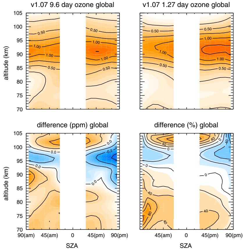
Figure 3. SABER daytime ozone as a function of solar zenith angle and altitude. In each panel, morning is on the left and afternoon on the right. Top left is 9.6 \mu\text{m} ozone; top right is 1.27 \mu\text{m} ozone; bottom left is absolute difference (9.6 \mu\text{m} ozone minus 1.27 \mu\text{m} ozone) and bottom right is percent difference.
