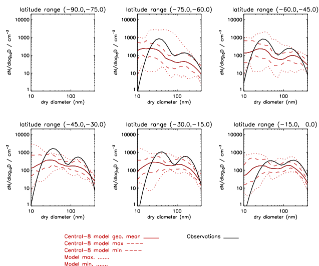
Figure 19. Southern Hemisphere annual-mean central-model simulated size distributions in the marine boundary layer averaged into 15^\circ latitude ranges to compare against the compilation of 30 yr of cruise DMPS/APS measurements from Heintzenberg et al. (2000). The solid line shows the geometric mean of the central-8 models, dashed lines indicate the maximum and minimum of the central-8, while dotted lines indicate the maximum and minimum over all 12 models.
