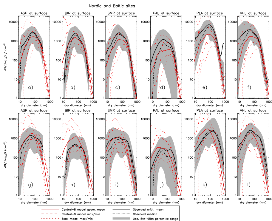
Figure 15. Summer (a–f) and winter (g–l) multi-model simulated size distributions against DMPS/SMPS measurements at the six Nordic/Baltic EUSAAR sites: Aspvreten (ASP), Birkenes (BIR), Hyytiälä (SMR), Pallas (PAL), Preila (PLA) and Vavihill (VHL). Shown are the central-8 model geometric means (red solid), central-8 model maximum/minimum (red dashed) and all-12 model minimum/maximum (red dotted) of the June–July–August (arithmetic) mean size distributions at each site. Observed values (black solid line) are arithmetic means over the hourly measurement data (A. Asmi, personal communication, 2012). The published (Asmi et al., 2011) median (black dot-dashed) and 5th to 95th percentile range (grey shading) over the hourly measurement data are also shown for reference.
