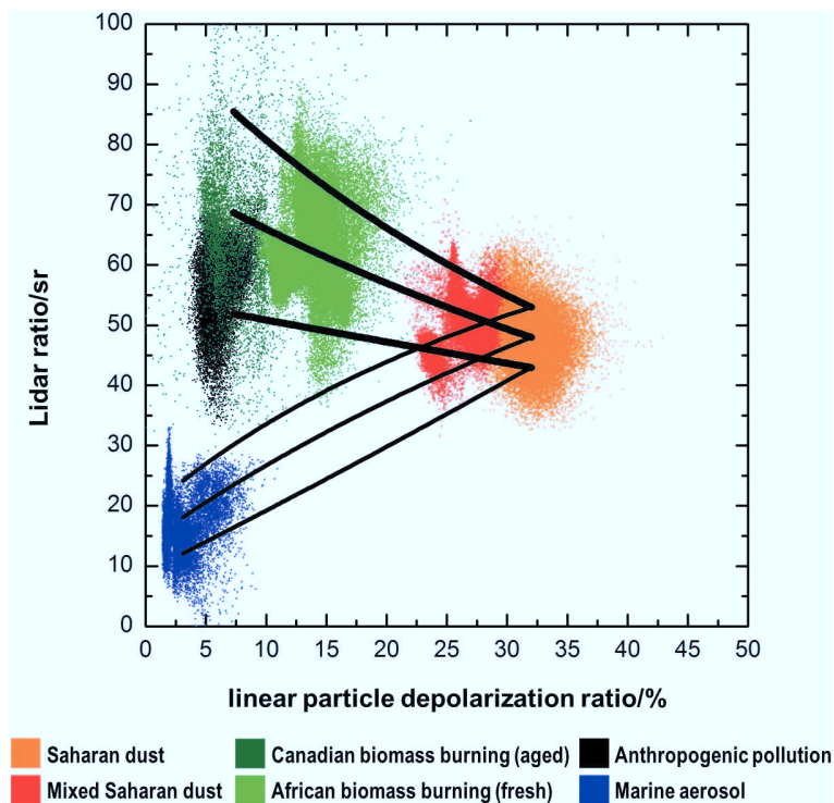
Fig. 6. Aerosol lidar ratio vs. particle linear depolarization ratio for various atmospheric aerosol types and mixing lines for Saharan dust and Canadian Biomass Burning Aerosol (thick lines), and for Saharan dust and Marine aerosol (thin lines). The central line in each case corresponds to the mean values as input for the calculation; the outer lines depict the maximum and minimum range when regarding the uncertainties of the input values.
