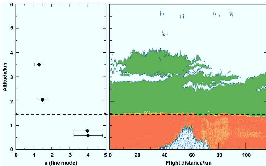
Fig. 10. Measurement example during SAMUM-2 on 25 January 2008. The left panel shows results of the in-situ measurements of the Angström exponent of absorption, the right panel shows the lidar signal, color-coded for the observed aerosol type (green for African biomass burning, orange for mixed Saharan dust).
