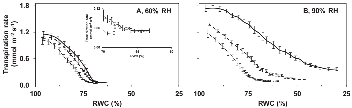
Fig. 2. Transpiration rate as a function of relative water content (RWC) during leaflet desiccation of pot rose 'Mandarin' grown at moderate (60%, A) or high (90%, B) relative air humidity (RH) under different soil water deficit treatments. Control plants at each RH were maintained well-watered based on evapotranspiration (continuous line). Soil water deficit treatments were realized by adjusting the irrigation to 1/4 (fine dashed line) or 1/2 (dashed line) of evapotranspiration throughout growth (see soil water potential in Fig. 1). Leaflets were left to desiccate for 4 h. The insert represents the same data as the main figure, using a different scale. Values are means of 12 leaflets \pm SEM.
