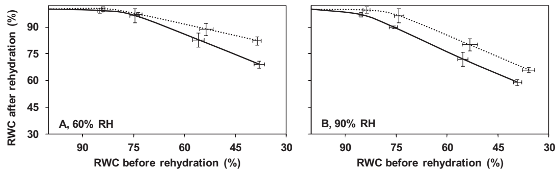
Fig. 4. Leaflet relative water content (RWC) following overnight (12 h) rehydration, as a function of RWC before rehydration of pot rose 'Mandarina' grown at moderate (60%, A) or high (90%, B) relative air humidity (RH) under different soil water deficit treatments. Control plants at each RH were maintained well-watered based on evapotranspiration (continuous line). The soil water deficit treatment was obtained by adjusting the irrigation to 1/4 of evapotranspiration throughout growth (fine dashed line; see soil water potential in Fig. 1). The rehydration method used was independent of the stomatal component. Values are means of 15 leaflets \pm SEM.
