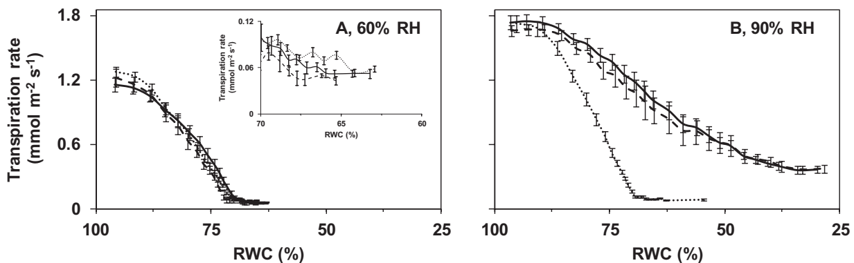
Fig. 3. Transpiration rate as a function of relative water content (RWC) during leaflet desiccation of pot rose 'Mandarin' grown at moderate (60%, A) or high (90%, B) relative air humidity (RH), and subjected to grafting. Control plants were grown on their own ('Mandarin') roots (continuous line). 'Mandarin' scions were grafted onto 'Mandarin' rootstock (self-grafting; dashed line) or onto the pot rose 'Apache' rootstock (fine dashed line). Plants on their own roots and grafted plants were maintained well-watered based on evapotranspiration throughout growth. Leaflets were left to desiccate for 4 h. The insert represents the same data as the main figure, using a different scale. Values are means of 12 leaflets \pm SEM.
