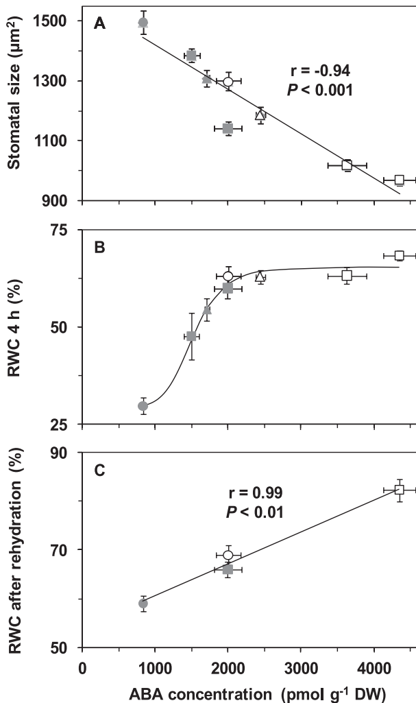
Fig. 5. Stomatal size (A; data in Supplementary Tables S1, S2 at JXB online), relative water content (RWC) following 4 h of leaflet desiccation (B; data of Figs 2, 3), and RWC following overnight rehydration from 30 \pm 1.4\% (C; data of Fig. 4) as a function of endogenous leaflet ABA concentration, expressed on a dry weight (dw) basis, of pot rose 'Mandarina' (data in Tables 1, 12). Plants were grown at moderate (60%, open symbols) or high (90%, filled symbols) relative air humidity, and exposed to different soil water potentials (squares indicate soil water deficit) or subjected to grafting (triangles). The RWC after 4 h of desiccation versus [ABA] data was fitted
