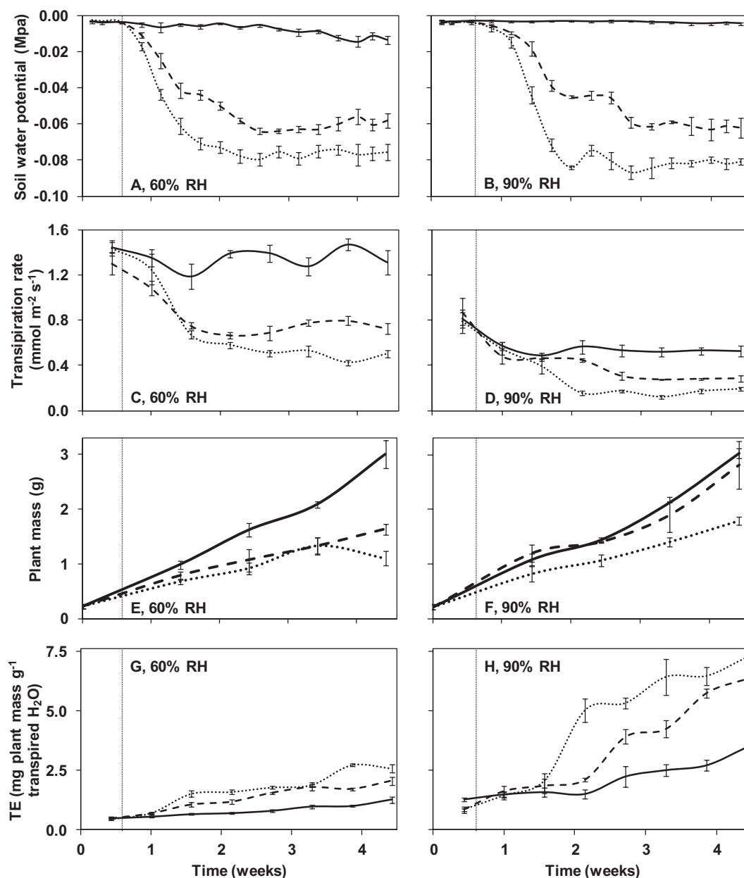
Fig. 1. Soil water potential (A, B), transpiration rate (C, D), plant (shoot plus root) mass (E, F), and transpiration efficiency (TE; G, H) during growth at moderate (60%) or high (90%) relative air humidity (RH) of pot rose ‘Mandarin’. Control plants at each RH were maintained well-watered based on evapotranspiration (continuous line). Soil water deficit treatments were realized by adjusting the irrigation to 1/4 (fine dashed line) or 1/2 (dashed line) of evapotranspiration at day 4 (indicated by the vertical line). Soil water potential ( n=4 ) and transpiration rate ( n=12 ) were assessed daily. Plant mass was determined in eight (0, 10, and 17 d) or 12 (24 and 31 d) plants per treatment. Error bars indicate the SEM.
