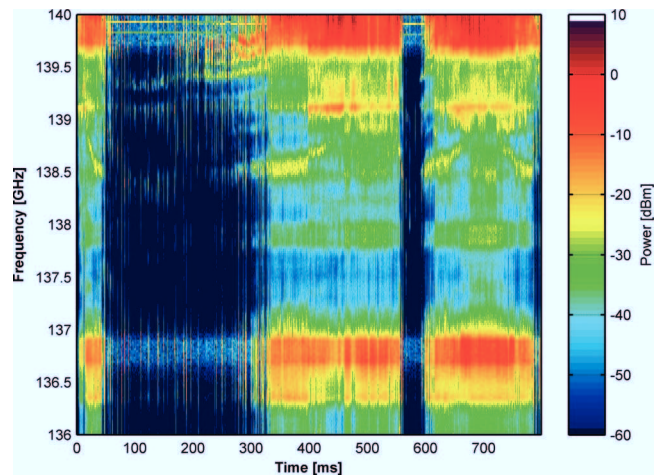
FIG. 7. (Color) Calibrated plot (see Fig. 5) of time-resolved frequency spectra of millimeter-wave radiation in the TEXTOR tokamak, shot No. 108086. The DED is used to move the magnetic island slightly back and forth through the observation region with a frequency of about 2 Hz. The thin green lines in the 139.8 GHz range are the reflections on the plasma of the gyrotron and one of its harmonics. The gyrotron signals are being suppressed below 120 dB. The frequency resolution is 4 MHz with a time resolution of 1 ms. The dynamic range of signal power exceeds 60 dB.
