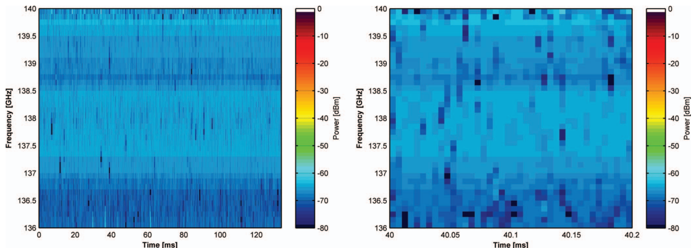
FIG. 3. (Color) Left: uncalibrated spectrogram of a measurement without any input signals, showing that 80-sample waveforms are acquired at a rate of 200 kHz, giving spectra with a frequency resolution of 100 MHz. The noise floor is at -63 dBm. Right: detail of the spectrogram, zoomed in at the time interval of 40.00–40.20 ms, showing 40 spectra.
