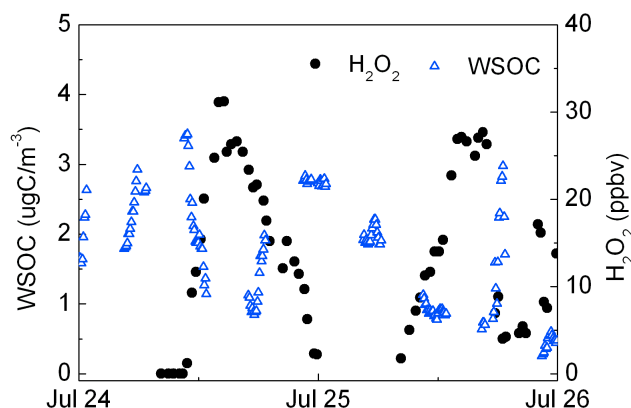
Fig. 8. Diurnal profiles of \text{H}_2\text{O}_2 and WSOC measured on 24 and 25 July.
