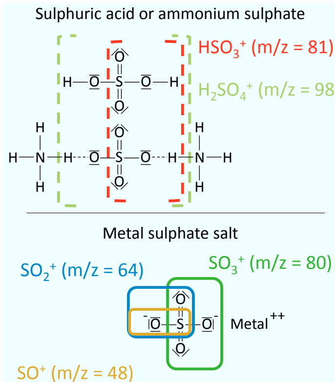
Fig. 7. Comparison between the possible fragments attributed to sulphate depending on the compound the sulphate is part of. For ammonium sulphate and sulphuric acid, hydrogen containing fragments are produced in the vaporisation and ionisation process while metal sulphate salts cannot produce such fragments.
