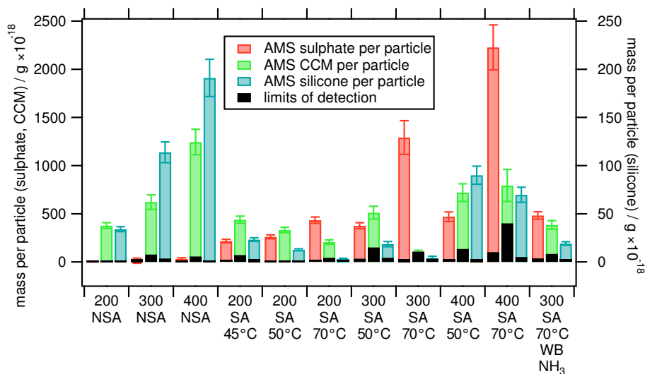
Fig. 6a. Summary of the mass per particle for the FROST1 campaign. First number of each category → particle diameter in nm, NSA → no sulphuric acid, SA → sulphuric acid and \text{NH}_3 → addition of ammonia. The temperature shown is the bath temperature for the respective coating substance. Note that the silicone axis is enhanced by a factor of 10 for clarity.
