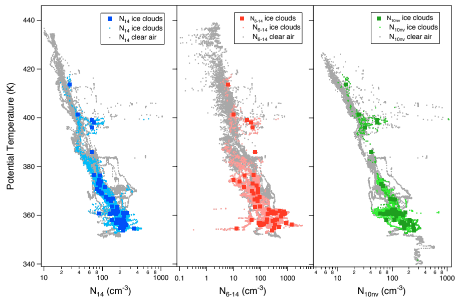
Fig. 8. Profiles of the total, ultrafine and non-volatile aerosol number concentration for in (coloured dots) and out of cloud (grey dots) measurements. The markers indicate the average interstitial aerosol number concentration within the selected ice clouds.
