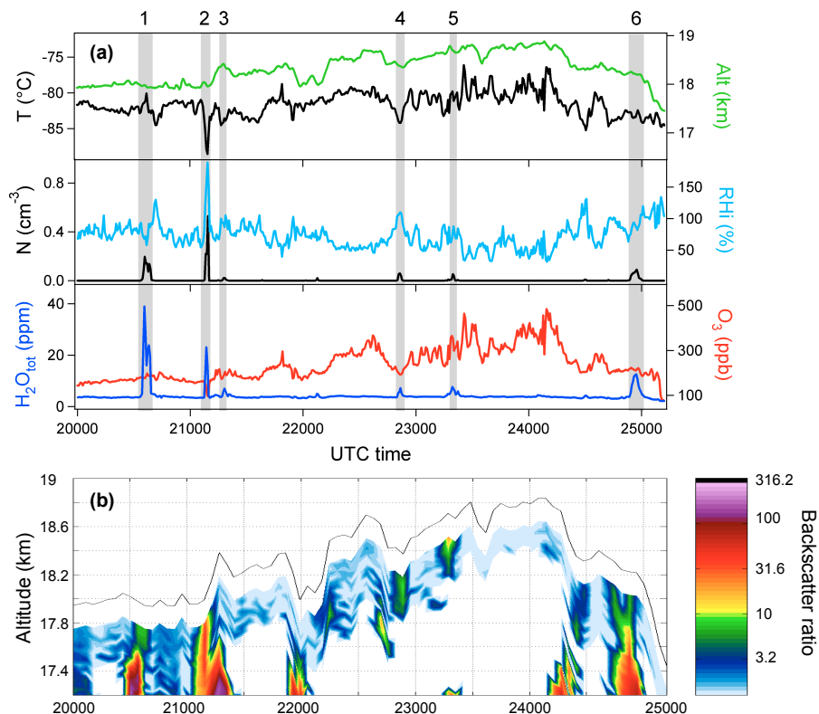
Fig. 6. (a) Ten second averaged values of the temperature, altitude, relative humidity, ice crystal number concentration ( N ), total water content ( H_2O_{tot} ) and O_3 mixing ratio during the stratospheric part of the flight on 30 November 2005. (b) Backscatter ratio below the aircraft as measured by the downward looking lidar. The black solid curve is the flight altitude.
