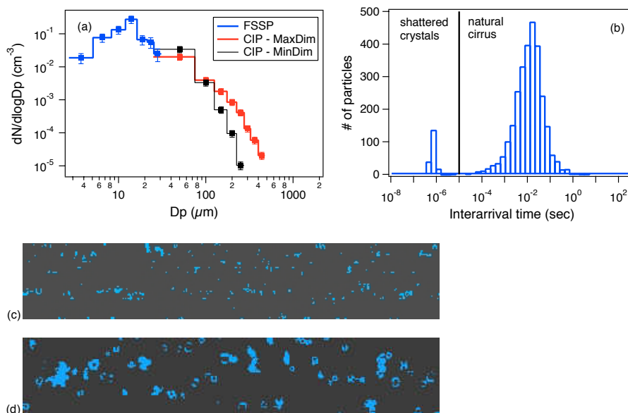
Fig. 1. (a) Ice crystal size distribution observed in the tropical stratosphere, 0.7 km above the local tropopause, over the Tiwi islands on 30 November 2005 (event 1 in Fig. 6). The ice crystal size distribution has been composed from FSSP and CIP data. For the CIP data the maximum and minimum dimension are shown. (b) Interarrival time distribution for the ice crystals observed by the CIP for this time period, indicating the crystals which are produced by shattering and therefore have been removed from the data set. (c) Ice crystal images recorded by the CIP instrument for this time period. (d) Example of larger ice crystals observed on 28 November 2005 at 10 km altitude.
