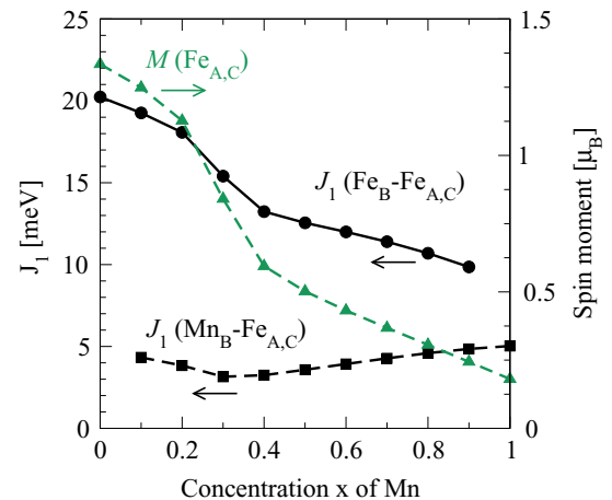
FIG. 9. (Color online) Nearest-neighbor exchange interactions J_1 between \text{Fe}_\text{B} and \text{Fe}_{\text{A,C}} atoms and between \text{Mn}_\text{B} and \text{Fe}_{\text{A,C}} atoms, as calculated by the Liechtenstein formula (3). The \text{Fe}_{\text{A,C}} moments, M(\text{Fe}_{\text{A,C}}) , are also shown, to demonstrate the correlation between the decrease of J_1 and M(\text{Fe}_{\text{A,C}}) .
