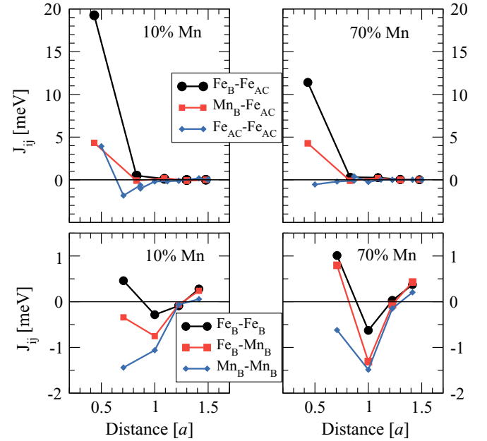
FIG. 8. (Color online) Pair exchange constants as a function of the interatomic distance. Left: 10% Mn concentration. Right: 70% Mn concentration. Note the different energy scale in the upper and lower panels. The lines are guides to the eye.
