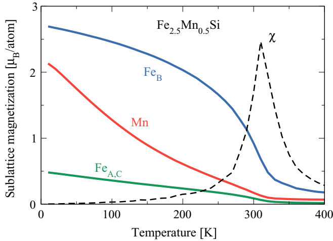
FIG. 11. (Color online) Monte Carlo simulation of the magnetization and susceptibility \chi vs temperature for \text{Fe}_{2.5}\text{Mn}_{0.5}\text{Si} . It is evident that the Mn sublattice magnetization drops much faster than the Fe magnetization. The susceptibility peak signals the Curie temperature.
