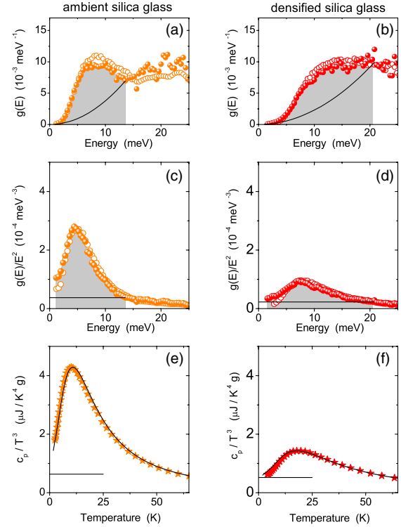
FIG. 1 (color online). The density of states (a)–(b) and the reduced density of states (c)–(d) of ambient and densified silica glass. The solid and the open circles refer to the NRAIXS and IXS data, respectively. The solid lines show the Debye levels for the DOS (a)–(b) and reduced DOS (c)–(d). The area of the filled region of the DOS above the Debye parabola in (a)–(b) gives the number of the excess states. The entire area of the filled region in (a)–(b) gives the number of all states within the same energy ranges. The filled areas in (c)–(d) show the same energy regions for the reduced DOS. (e)–(f) The measured specific heat (symbols) and the specific heat calculated from the corresponding DOS (solid lines). The horizontal lines in (e)–(f) show the Debye levels for the specific heat.
