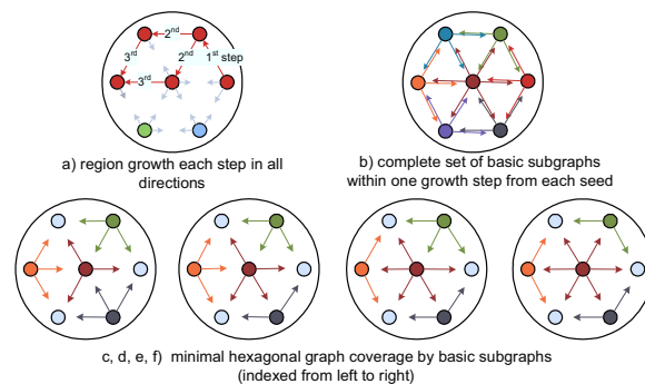
Figure 23: Hexagonal graph coverage for parallel structural coding
