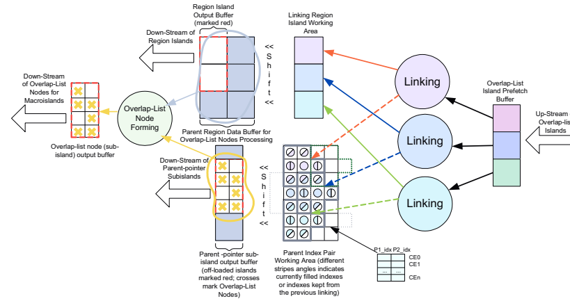
Figure 15: Linking Unit pipeline
