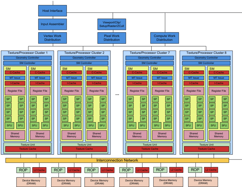
Figure 5: nVidia G80 architecture
