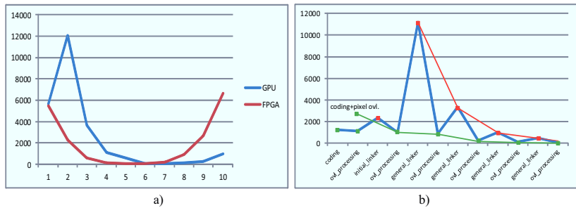
Figure 47: Typical level processing time profiles for FPGA and GPU implementations (sampled for 1024 2 image size, y-axis is time in micro sec.) a) FPGA and GPU combined profile; b) GSC GPU stage detailed profile
