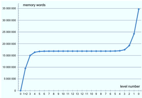
Figure 22: Accumulated traffic per GSC level (in memory words for 4096 2 image resolution)
