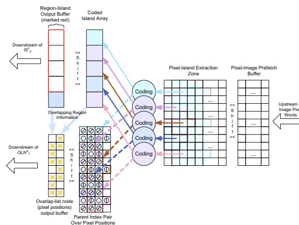
Figure 16: Coding Unit pipeline
