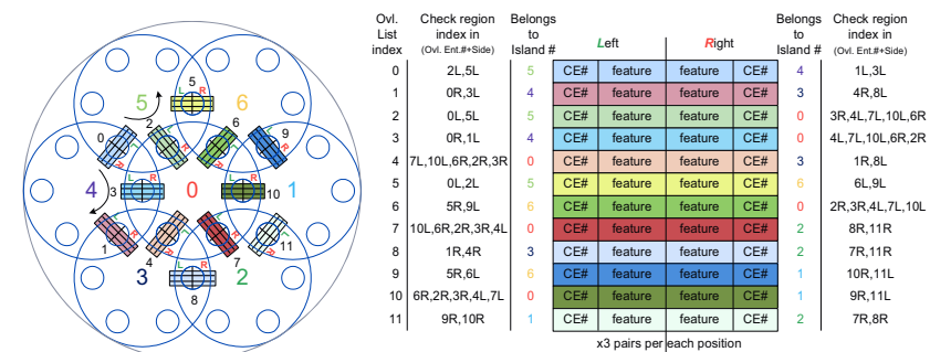
Figure 25: Overlap-list topology relationship
