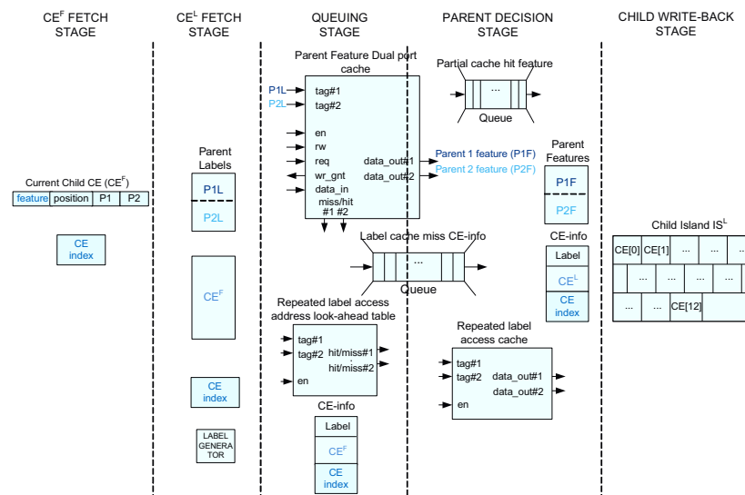
Figure 35: Labelling pipeline with out-of-order execution
