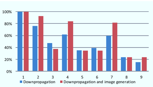
Figure 45: Relative performance graph of Downpropagation kernel implementations DP1-DP9
