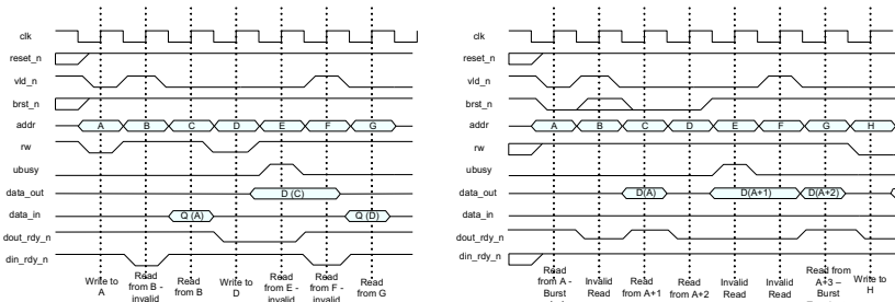
Figure 28: ZBT controller interface cycle diagram
