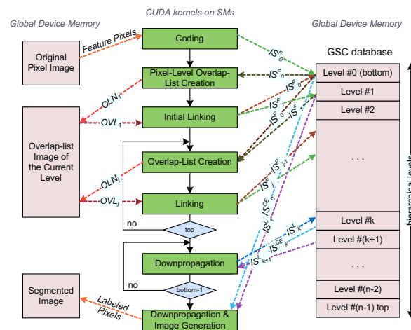
Figure 36: GPU GSC application structure
