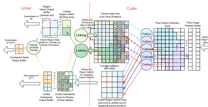
Figure 21: Initial Linker Unit structural scheme
