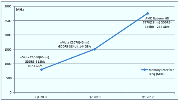
Figure 51: Bandwidth trend of GPU-board memory interfaces
