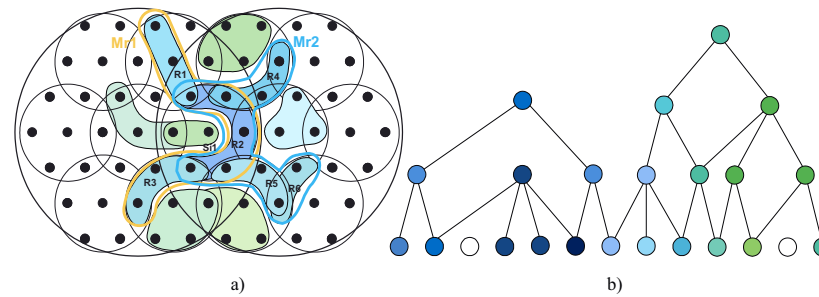
Figure 3: Region forming and region relationship tree a) Region forming example: R1, R2, R3 and R4, R5, R6 form two macro-regions Mr1 and Mr2 respectively, as they have common overlapping points, satisfy a threshold condition and are covered by common hierarchical islands; the macro regions Mr1 and Mr2 have a chance to be linked at the next hierarchical islands if they are covered by a common macro-island as they have a common sub-region R2 and seem to be similar. b) Hierarchical relationship of regions represented as a region relationship tree
