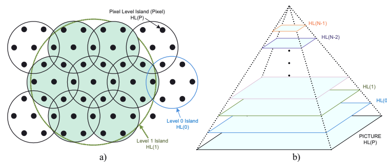
Figure 2: Pyramidal hierarchical-layer structure ( HL(i) – hierarchical level, i – level index) a) Island hierarchy relationship; b) GSC relationship pyramid
