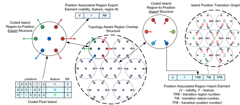
Figure 24: Pixel-region macroisland overlap structure
