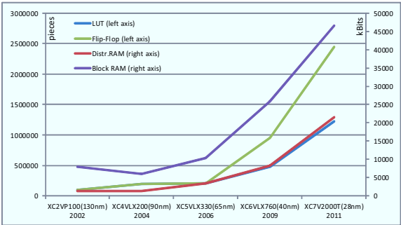
Figure 50: FPGA technological trends (Virtex FPGA family evolution)
