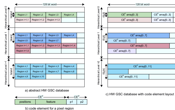
Figure 12: Hardware GSC database
