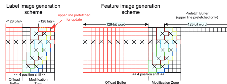
Figure 19: Image Generator scheme
