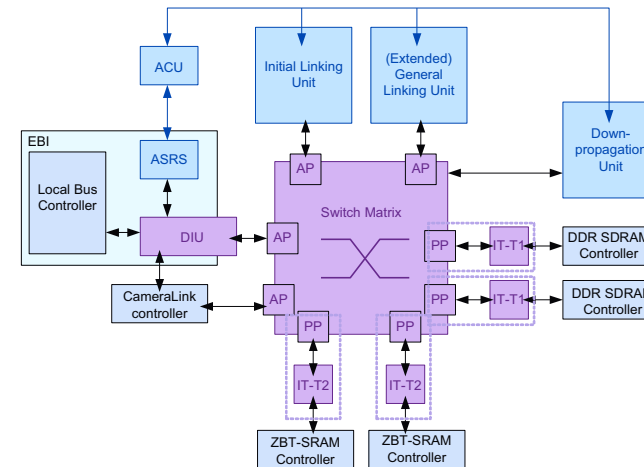
Figure 27: System on the FPGA chip
