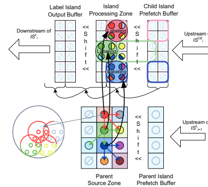
Figure 18: Downpropagation Unit pipeline
