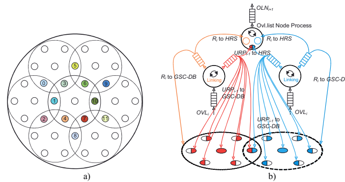
Figure 10: Linking data-flow model a) Fixed mapping scheme of overlapping nodes in a macroisland; b) Data-flow model of linking process
