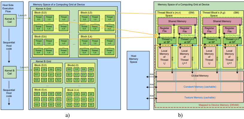
Figure 6: CUDA architecture a) CUDA application model; b) CUDA memory model
