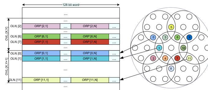
Figure 13: Hardware Overlap-list layer
