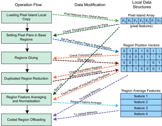
Figure 38: Coding kernel processing flow
