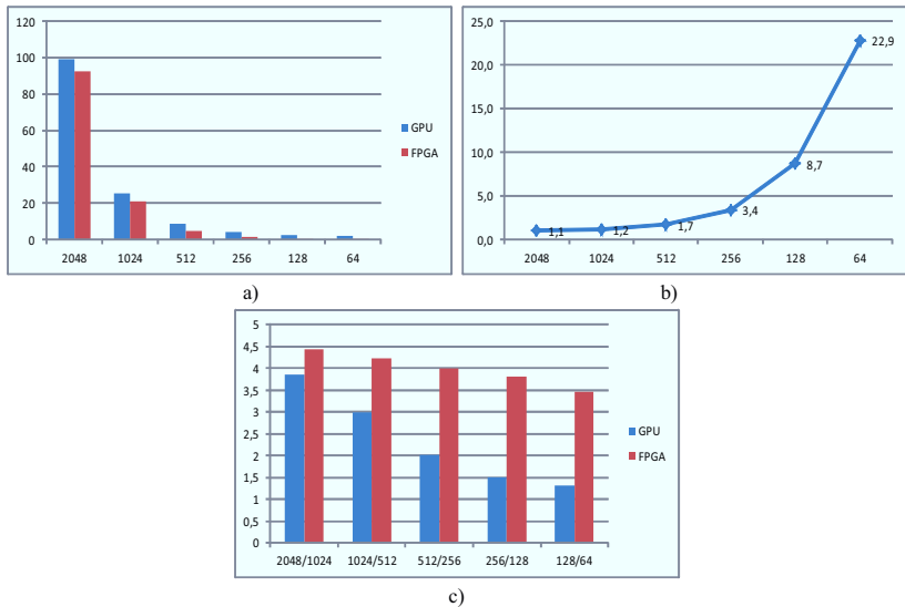
Figure 46: Processing times and dataset size scaling ratios a) Processing time for different resolutions (ms); b) GPU to FPGA processing time ratios c) Processing time scaling ratios (next to previous resolutions)
