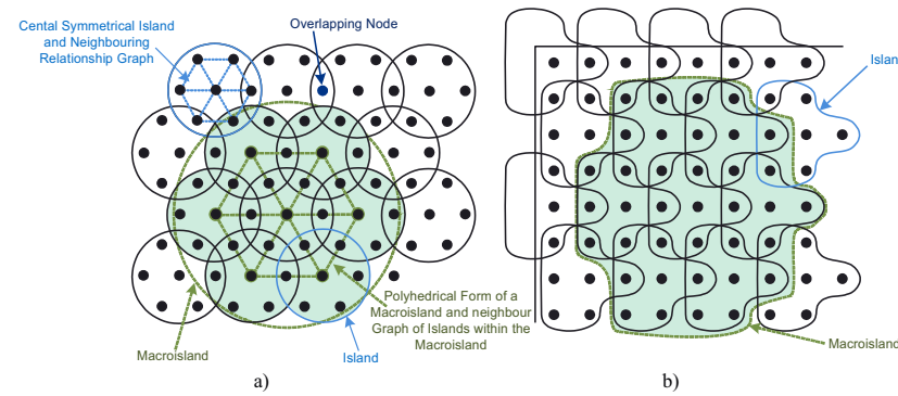
Figure 1: Forming hierarchical island structure a) Overlapping central symmetric islands on the hexagonal Bravais lattice b) Mapping of hierarchical overlapping island structure to a pixel image
