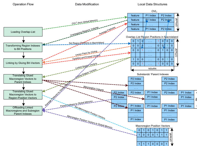
Figure 42: Processing flow of Linking kernel
