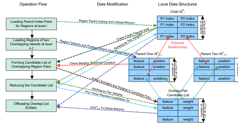
Figure 40: Processing flow of Overlap-list Creation kernel
