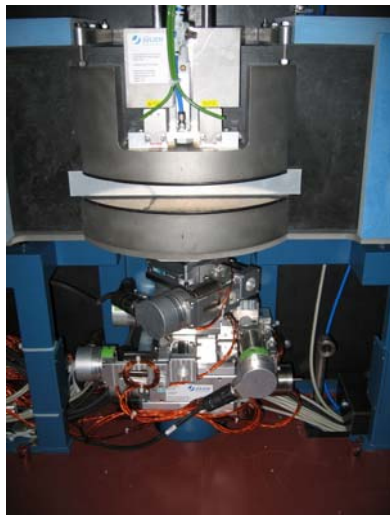
FIG. 2: The monochromator column inside the monochromator shielding (blue part on the right in Fig. 1) with the five axes assembly necessary to move the monochromator crystal according to the desired wavelength. In the upper part of the picture the first instrument shutter called photo-shutter can be seen which consists of a 4 mm B 4 C ceramic plate moved by an air piston. The remaining space in front of the monochromator column is reserved for two apertures and a velocity selector.
