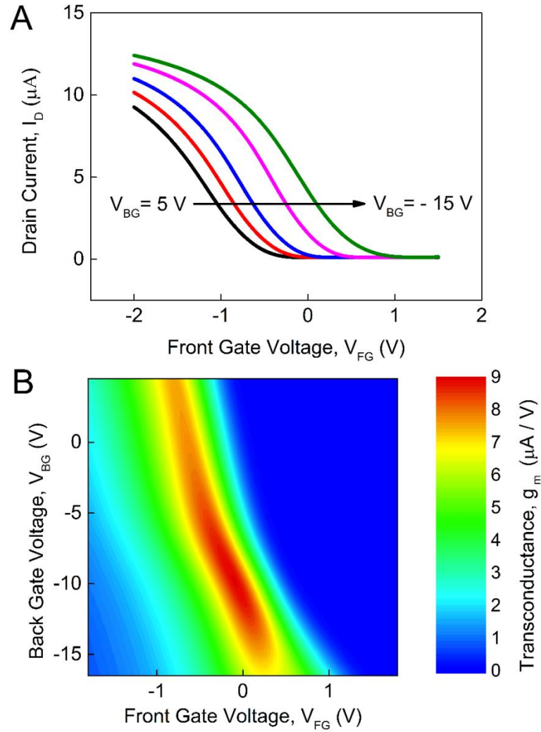
Figure 2. (a) Transfer curve of Si NW array FET with 50 nanowires (with 250 nm width and channel length of 16μm), measured at drain voltage, V_{DS} , of 1 V and back-gate voltages, V_{BG} , which varied in the range from 5V to -15V with a step size of 5V. The direction of V_{BG} changes is shown with an arrow in the figure. (b) Transconductance of the Si NW array FET measured at V_{DS} , of 1 V and plotted in a colour map as a function of V_{BG} and V_{FG} . Red corresponds to the maximum transconductance.
