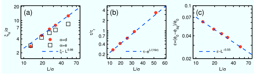
Fig. 5: (color online) (a) Correlation lengths of the displacements \xi_d(\tau) and the orientations \xi_e as a function of system size L . (b) Exponential grow of the build-up time \tau with L . (c) Local density of the liquid phase \phi_{liq} increases with L . The same parameter as in Fig. 4, \phi = 0.6 and Pe = 272 .
