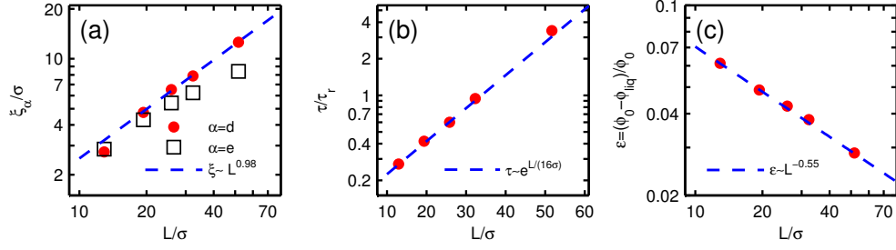
Fig. 5: (color online) (a) Correlation lengths of the displacements \xi_d(\tau) and the orientations \xi_e as a function of system size L . (b) Exponential growth of the build-up time \tau with L . (c) Local density of the liquid phase \phi_{liq} increases with L . The same parameter as in Fig. 4, \phi = 0.6 and Pe = 272 .
