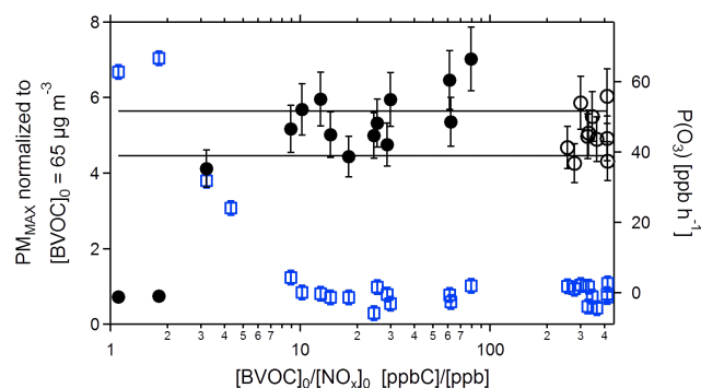
Fig. 7. PM max normalized to [BVOC] 0 = 65 \mu\text{g m}^{-3} in dependence of BNR assuming incremental mass yield of 0.117. Solid circles show data from experiments with NO x addition; open circles are from experiments without NO x addition. The error in PM MAX,norm is mainly due to the extra- and interpolations to [BVOC] 0 = 65 \mu\text{g m}^{-3} and estimated to \pm 12\% . The black lines show the average \pm 1\sigma standard deviation (upper/lower line) of the data without NO x addition. For comparison P(O 3 ) is shown (blue squares) as in Fig. 5. For one of the experiments (BNR = 4.3, [NO x ] 0 = 23 ppb) PM MAX was not available. Therefore the number of data in Fig. 7 include one less than in Fig. 5.
