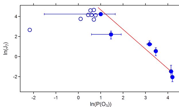
Fig. 10. Double logarithmic plot of J_7 ( \text{cm}^{-3} \text{s}^{-1} ) vs. P(O_3) ( \text{ppb h}^{-1} ). Open circles are data obtained at P(O_3) < 2.5 \text{ ppb h}^{-1} , closed circles are data obtained at P(O_3) > 2.5 \text{ ppb h}^{-1} . Data pairs with P(O_3) < 2.5 \text{ ppb h}^{-1} were regarded as error prone because P(O_3) was calculated to -0.15 \pm 2.5 \text{ ppb h}^{-1} when no NO x was added although P(O_3) was essentially zero. Therefore linear regression analysis was restricted to data points with P(O_3) > 2.5 \text{ ppb h}^{-1} . The slope of the linear regression line is -1.6 \pm 0.27 , R^2 = 0.9 . Data points with formally negative P(O_3) are not included in the plot. Error bars added only to data points used for the fit. Note that for P(O_3) approaching the significance level, the error of the logarithm approaches infinity ( \infty ).
