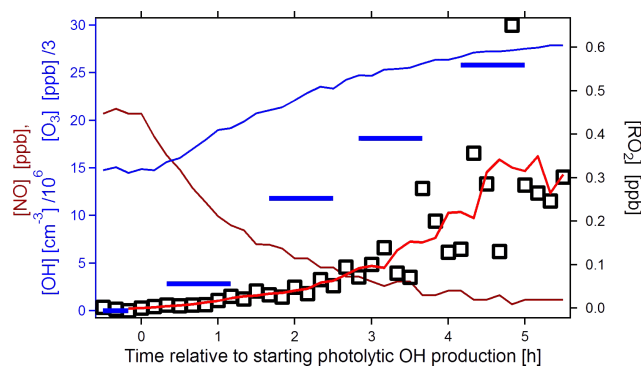
Fig. 9. Estimated [RO_2] ( = \sum_i [RO_2^i] ) using deviation from PSS
