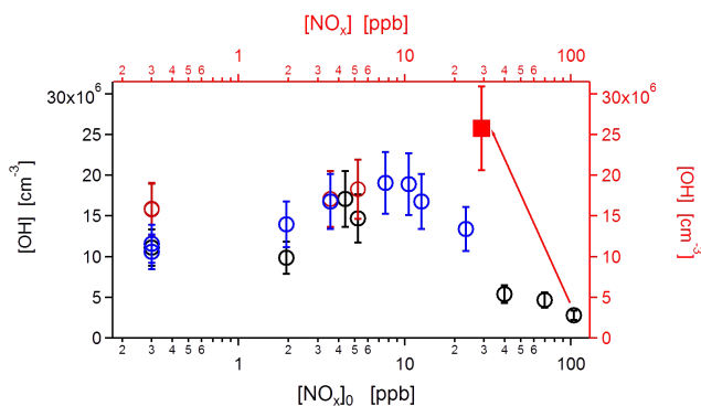
Fig. 6. OH concentrations measured during the first hour after switching on the TUV lamp in dependence of [NO x ] 0 (note logarithmic scale of x axis). The error in OH concentrations is estimated to be \pm 20\% . Brown circles represent OH measured at [BVOC] 0 < 55 \mu\text{g m}^{-3} , blue circles those measured at 55 < [BVOC] 0 < 65 \mu\text{g m}^{-3} and black circles those measured at [BVOC] 0 > 65 \mu\text{g m}^{-3} . The red square shows the OH concentration measured for the highest NO x addition ([NO x ] 0 = 103.5 ppb), 5 h after ignition of the TUV lamp. After that time new particle formation was observed, [O 3 ] had increased to 85 ppb and [NO x ] had decreased to 26 ppb.
