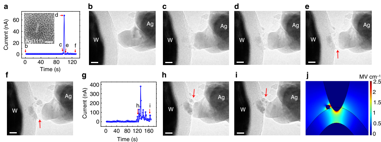
Figure 5 | Filament instability due to electrode depletion and recovery. (a) I - t curve of the device. A constant voltage of 7 V was applied on the Ag electrode. The SiO 2 film thickness was 20 nm. The inset shows high-resolution transmission electron microscopy image of a Ag nanocluster inside the SiO 2 film, resolving (111) planes of Ag with a face-centered cubic (fcc) structure. Scale bar, 2 nm. (b-f) Real-time TEM images showing the filament growth at different stages corresponding to data points b-f in a. Scale bar, 10 nm. (g) I - t characteristics of the same device during reprogramming with a constant voltage of 2 V. (h,i) Real-time TEM images of the device corresponding to data points h, i in g, showing recovery of the Ag/SiO 2 contact. Scale bar, 10 nm. (j) Electric field distribution in the device state shown in (h,i) by COMSOL simulation.
