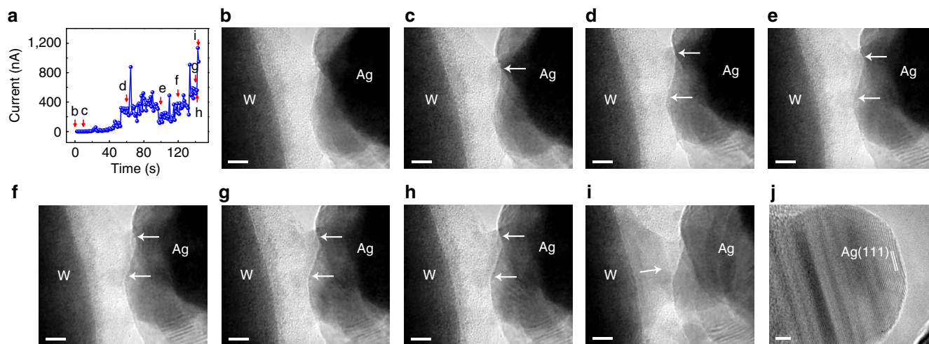
Figure 6 | Transition between different filament growth modes. (a) I - t curve of the device with a 10-nm SiO 2 film. A constant voltage of 2 V was applied on the Ag electrode. (b–i) Real-time TEM images showing filament growth corresponding to data points b–i in a . Scale bar, 5 nm. (j) High-resolution transmission electron microscopy image of the filament in i after removing the Ag electrode. Scale bar, 2 nm. The filament was found to be a solid crystalline Ag wire with face-centered cubic (fcc) structure.
