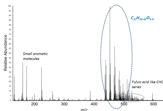
Figure 3. High-resolved spectrum (negative mode) of guttation droplets
