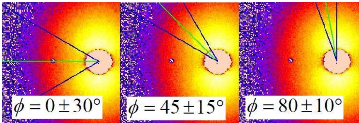
Image 12: Typical 2D SANS pattern with the mask \Phi=0\pm30^\circ , \Phi=45\pm30^\circ , \Phi=80\pm30^\circ [Koh97].
