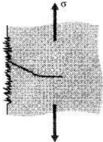
Image 5: Model of fatigue crack initiation [Dav01]
