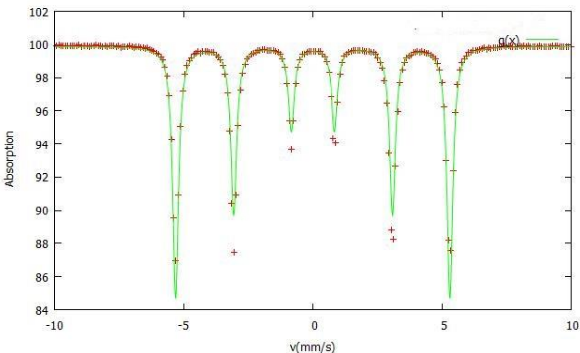
Image 38: Fitted Mössbauer spectrum for standard \alpha -Fe
