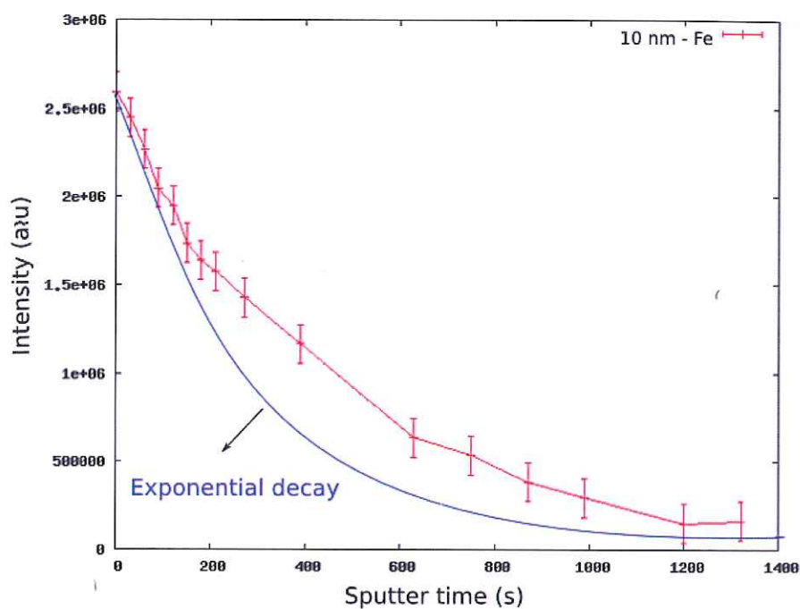
Figure 5.5 – Intensity of Fe (measured by AES) not exponentially dependent on sputter time
