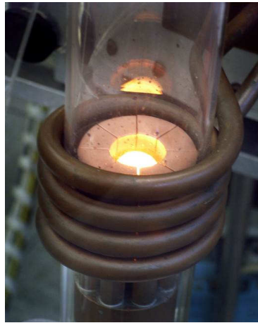
Figure 5.1: Photo of the melting process of the material in the cold crucible induction melting.
