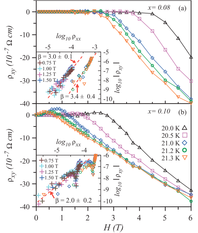
FIG. 5. (Color online) Magnetic-field dependence of \rho_{xy} for BFCA with (a) x=0.08 and (b) 0.10 at various temperatures. Insets of (a) and (b) demonstrate the plots of \log_{10} |\rho_{xy}| vs \log_{10} \rho_{xx} taken respectively at fixed magnetic fields and fixed temperatures for the corresponding samples. The dashed lines indicate the fitting of \rho_{xy} \propto (\rho_{xx})^\beta .
