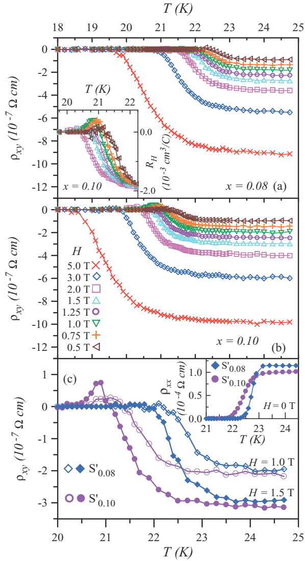
FIG. 4. (Color online) Temperature dependence of \rho_{xy} for BFCA samples with (a) x=0.08 and (b) 0.10 . Inset of (a): Hall coefficient versus temperature for BFCA with x=0.10 . (c) Temperature dependence of Hall resistivity \rho_{xy} taken on the other two samples as described in the text. Inset of (c): Resistive transition for the corresponding samples.
