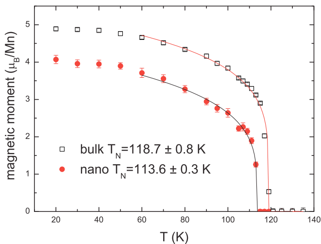
FIG. 2. (Color online) The temperature-dependent magnetic moment of the MnO bulk and nanoparticles of sample A. The solid lines are guides for the eye.
