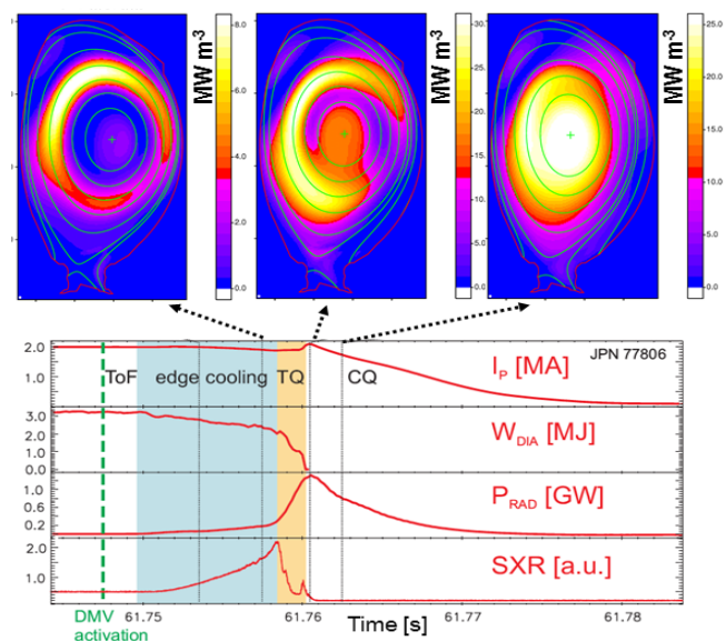
Fig.1. Time traces during a typical induced disruption caused by injection of a mixture of 10%Ar and 90%D 2 . Also shown are the radiation distributions during different time phases of the disruption.
