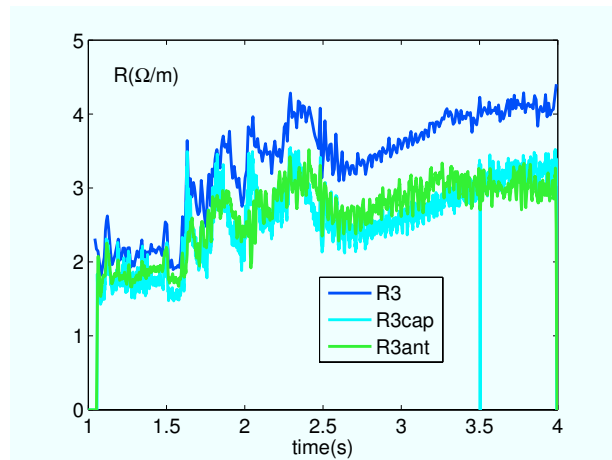
Figure 2 Comparison of the evolution of loading resistance versus time using standard method ( R_3 ) or deduced from voltages measured near the antenna or close to the capacitors ( R_{3ant}, R_{3cap} )
