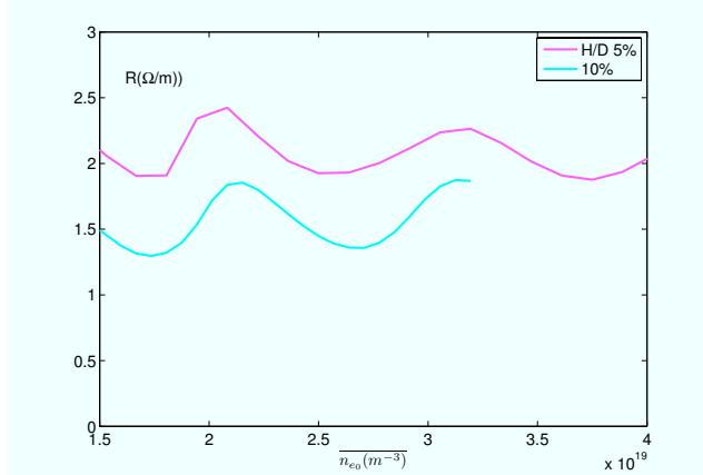
Figure 5 Evolution of loading resistance versus \overline{n_{e0}} for 2 values of Hydrogen minority concentration deduced from run of BRACC code for constant density in the edge.
