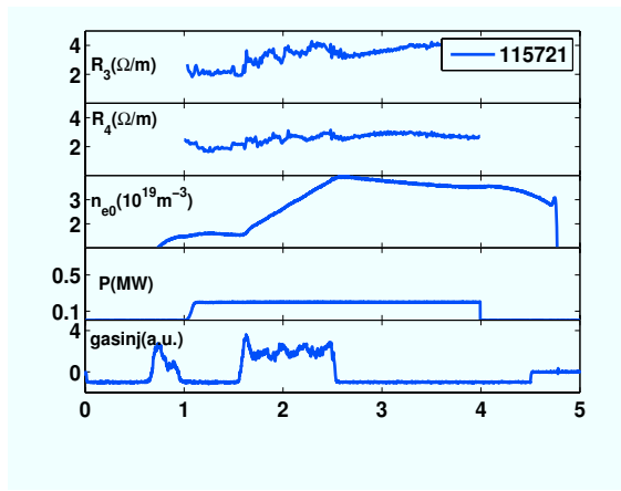
Figure 1 Time evolution of loading resistance ( R_3, R_4 ) of the two CT antenna straps, line integrated density, RF power and signal indicating gas injection.
