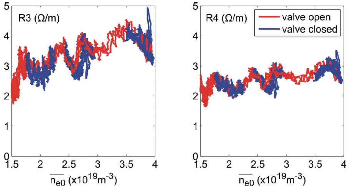
Figure 3 Comparison between the evolution of the loading resistance vs n_{e0} with gas injection valves open or closed
