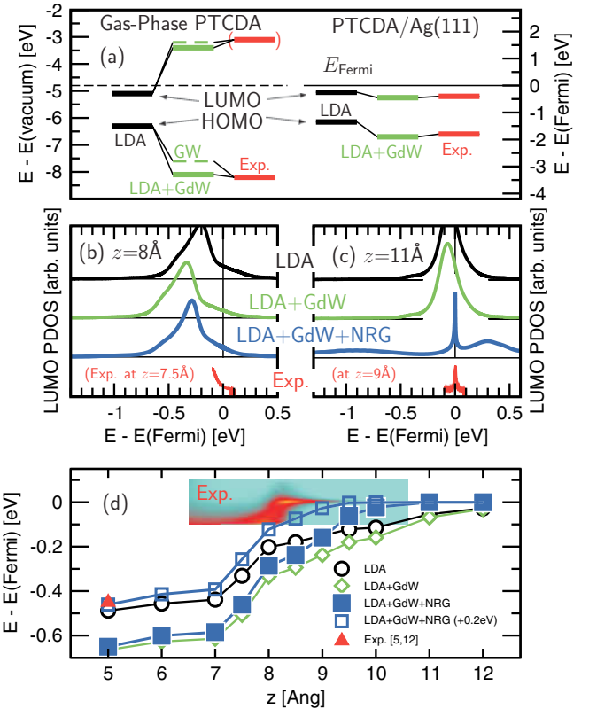
FIG. 2. (Color online) (a) HOMO and LUMO energies of gas-phase PTCDA and PTCDA/Ag(111) (peak of the PDOS; without STM tip). Experimental data are from Refs. 27,28 (gas phase), and 14 [on Ag(111)]. The two energy scales differ by E_F = E_{\text{vac}} - E_W [ E_W = work function of Ag(111)]. (b) and (c) LUMO spectra for the tip/PTCDA/Ag(111) junction at tip heights of z = 8 Å and z = 11 Å. The experimental spectra are cuts through the dI/dV map of panel d, at z values of 7.5 Å and 9 Å. (d) LUMO peak positions and experimental dI/dV color map, ranging from 0 G_0 (light blue) to 0.10 G_0 (yellow). Experiments were performed by approach-retraction cycles of the tip, with bias voltages increasing in steps of 1 mV. dI/dV was detected with a lock-in amplifier, modulation amplitude 4 mV and modulation frequency 2.9 kHz. For bias voltages exceeding \pm 100 meV, the tip-PTCDA contact becomes unstable. The experimental data point at ( z = 5 Å, E = -0.45 eV) is an estimate from Ref. 2 (−0.35 eV with the tip attached to the PTCDA monolayer) and Ref. 26 (the difference -0.1 eV between single-molecule and monolayer spectra).
