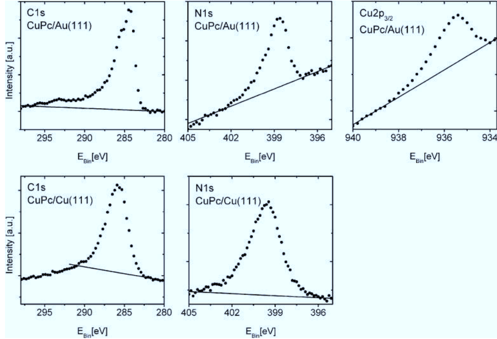
FIG. 1. Exemplary XPS spectra of the investigated species.
